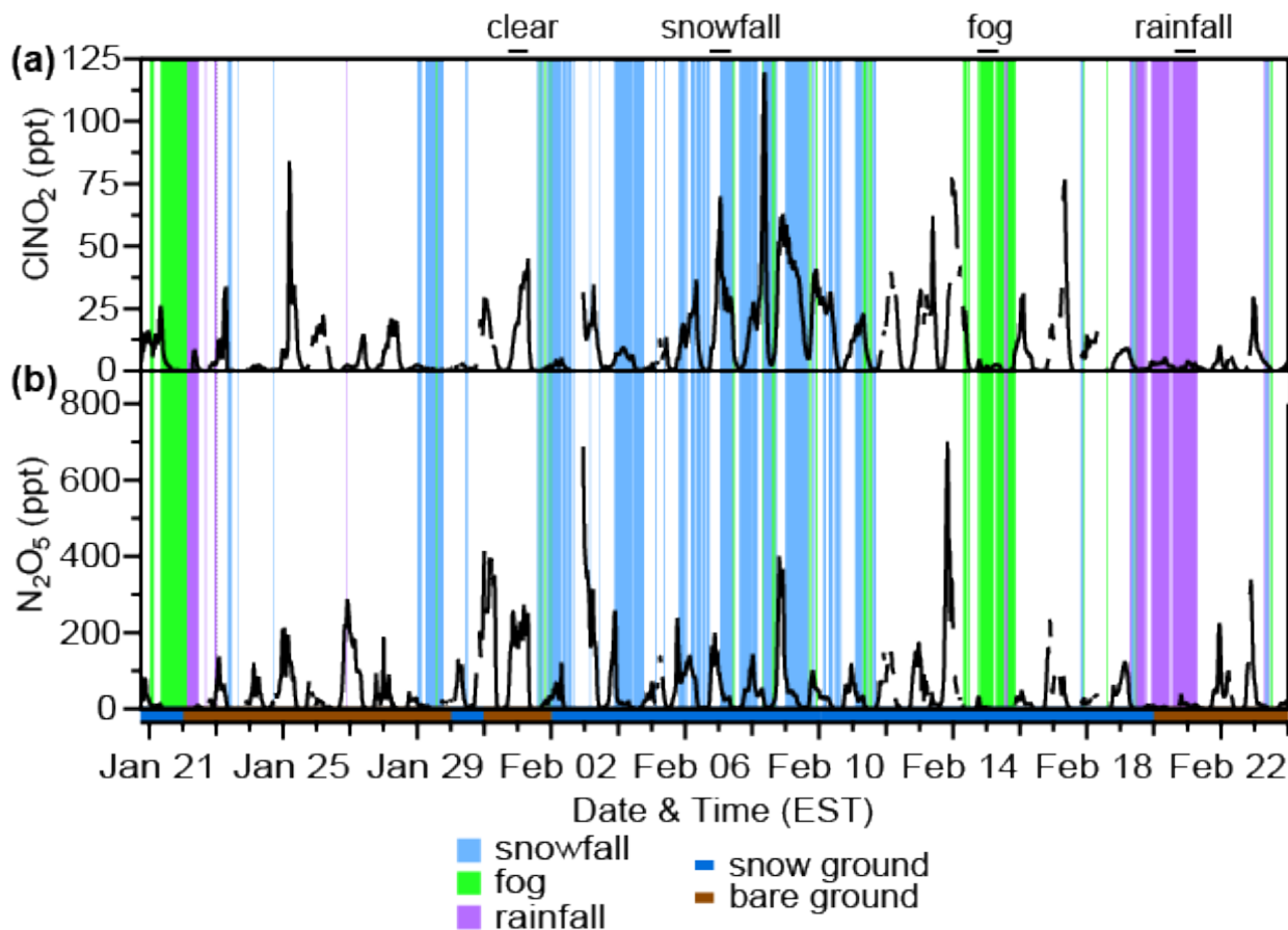
Figure 1: Mole ratios of 30 min averaged (a) \text{ClNO}_2 and (b) \text{N}_2\text{O}_5 during the campaign, and occurrence of snowfall (light blue), fog (green), and rainfall (purple). The shading below the x-axis represents ground cover – snow (blue) or bare ground (brown). The black bars on the top of the plot show the selected case study nights for each weather event type. Between 18:00 and 08:00 h EST, where n =number of 30 min periods, the air was clear 72% of the time [ n=726 ; 363 h], snowfall occurred 16% of the time [ n=157 ; 78.5 h], rainfall occurred 6% of the time [ n=63 ; 31.5 h], and fog occurred 6% of the time [ n=58 ; 29 h]. The ground was snow-covered 57% of the study [20 d] and was bare for 43% of the study [15 d]. Figure S3 gives further details about the occurrence of weather events (rainfall, fog, snowfall) in relation to friction velocity and ground cover.
