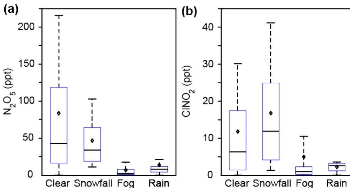
250 Figure 2: Box plots showing 30 min averaged mole ratios of (a) N_2O_5 and (b) ClNO_2 during clear conditions and weather events (snowfall, fog, and rain) from the entire campaign, January 20 - February 24. Bars represent the 10 th , 50 th , and 90 th percentiles, boxes represent the 25 th and 75 th percentiles, and diamonds represent the means. Only nighttime data between 18:00 and 08:00 EST are included. Data during all weather events (snowfall, fog, rain) are significantly different ( p < 0.05 , t-test) from clear 255 conditions.
