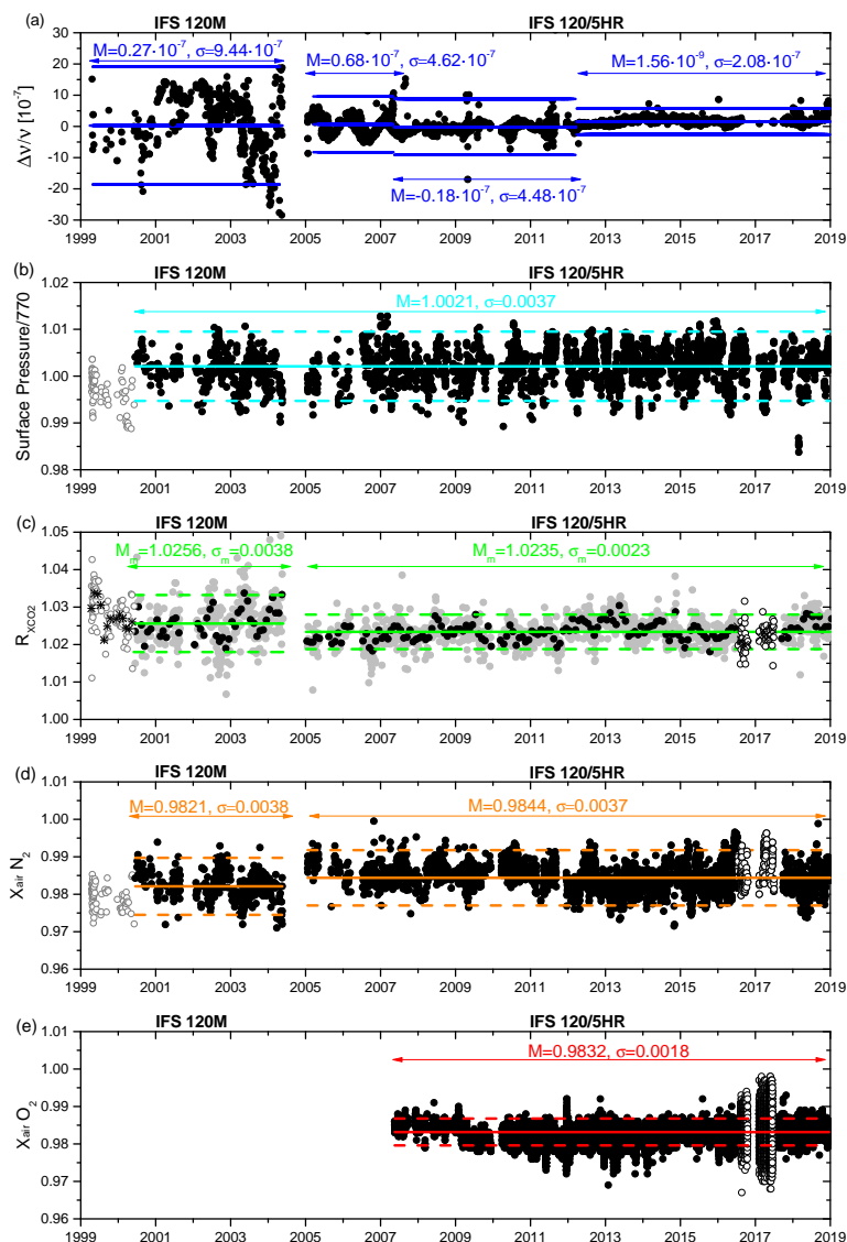
Figure 6. Time series of (a) Doppler spectral scaling factor \Delta\nu/\nu estimated from measured MIR spectra around 2104\text{ cm}^{-1} solar line; (b) surface pressure (normalised by typical surface pressure at IZO of 770 hPa); (c) R_{XCO_2} ratio; (d) and (e) X_{\text{air}N_2} and X_{\text{air}O_2} parameters, calculated using N_2 TCs from the NDACC FTIR spectra and O_2 TCs from the TCCON FTIR spectra, respectively. M_m and \sigma_m stand for mean and standard deviation values computed from the monthly time series (in (c)), while M and \sigma refer to the same statistics, but based on single measurements (in (d) and (e)). The period marked with grey-white dots (in (b), (c), and (d)) denotes instrumental issues on surface pressure records and has been ruled out to compute the statistics displayed in the sub-plots. Black-white dots in (d) correspond to 2016-2017 period, when frequency instabilities were detected in FTIR internal reference laser. Solid and dashed lines represent mean values and \pm 2\sigma ranges, respectively.
