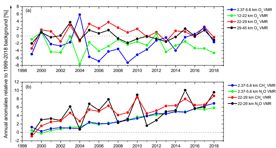
Figure 11. Time series of annual anomalies relative to the 1999-2018 background [in %] for NDACC VMR means of (a) \text{O}_3 (2.37-5.6, 12-22, 22-29, and 29-45 km layers), and (b) \text{CH}_4 , and \text{N}_2\text{O} (2.37-5.6, and 22-29 km layers). Annual anomalies are computed according to temporal decomposition as detailed in Appendix B.
