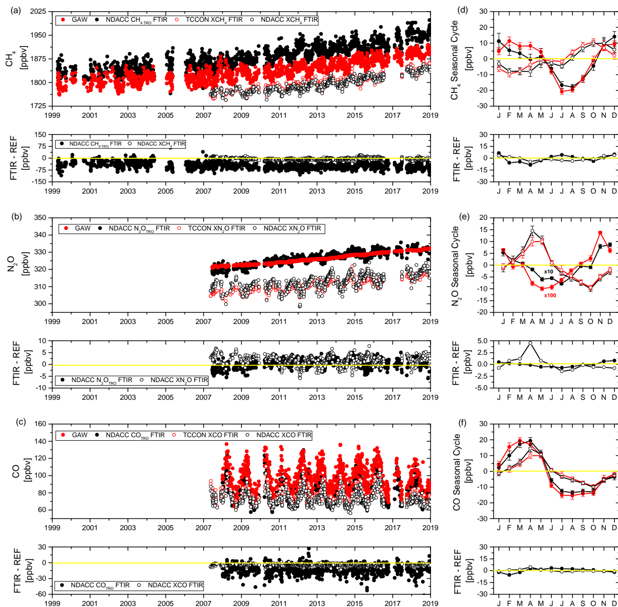
Figure 13. As for Figure 12, but for tropospheric and column-averaged NDACC products: (a) and (d) CH 4 , (b) and (e) N 2 O, (c) and (f) CO.
