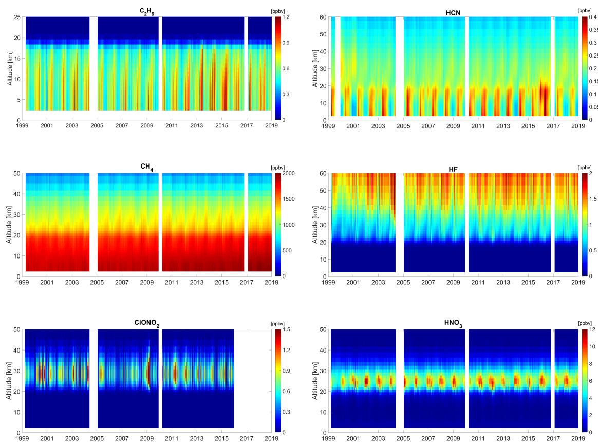
Figure 9. Time series of NDACC VMR vertical profiles at IZO from 1999 to 2018: C_2H_6 , CH_4 , ClONO_2 , HCN , HF , and HNO_3 . Ordinate limits as in Figure 3. Also note that the range of the coloured scale, showing VMR concentrations, has also been adapted for each trace gas. White areas correspond to data gaps due to instrumental issues (recall Table 1).
