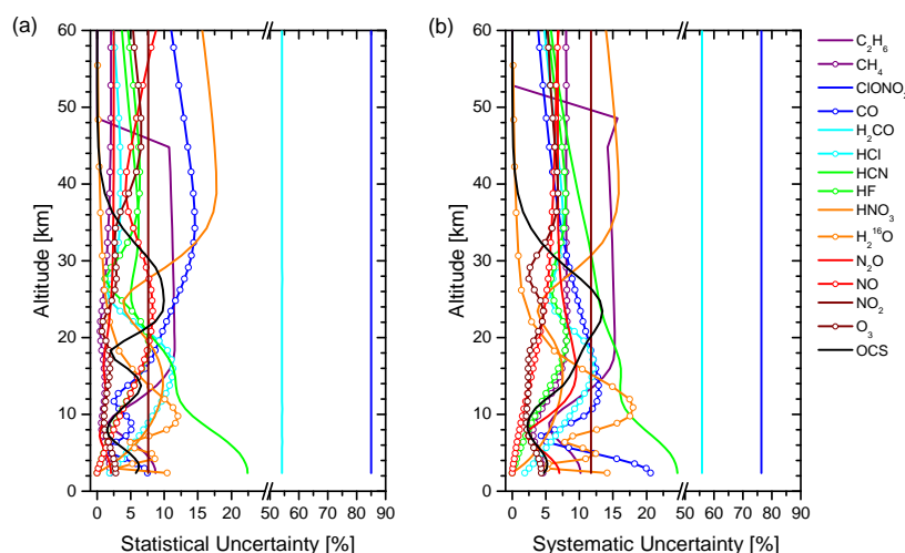
Figure 4. Example of estimated uncertainty profiles for all standard and non-standard NDACC products for typical measurement conditions at IZO (same spectrum as Figure 3): (a) total errors due to statistical uncertainty sources, and (b) total errors due to systematic uncertainty sources. Total errors are computed as the square root of the quadratic sum of all statistical and systematic error sources considered according to Appendix A. Note that for water vapour only the error profiles of the main isotopologue ( \text{H}_2^{16}\text{O} ) are shown.
