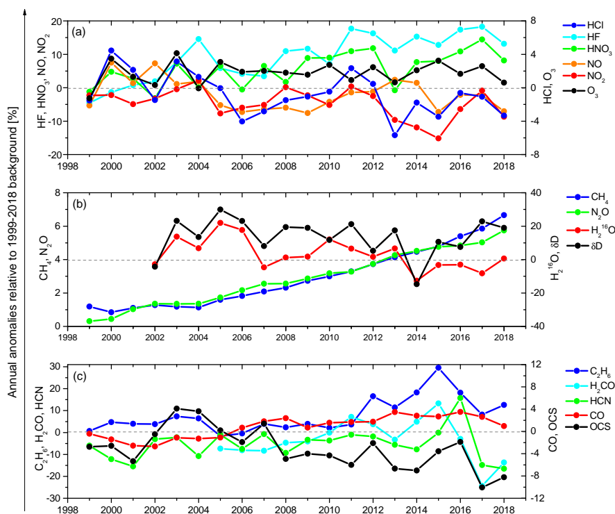
Figure 8. Time series of annual anomalies relative to the 1999-2018 background [in %] for NDACC TCs of (a) stratospheric gases (HCl, HF, \text{HNO}_3 , NO, \text{NO}_2 , and \text{O}_3 ), (b) greenhouse gases ( \text{CH}_4 , \text{H}_2\text{O} , and \text{N}_2\text{O} ) and \delta\text{D} , and (c) tropospheric and air quality gases ( \text{C}_2\text{H}_6 , CO, \text{HC}_2\text{O} , HCN, and OCS). Annual anomalies are computed according to temporal decomposition as detailed in Appendix B.
