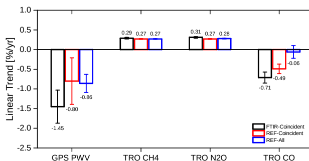
Figure 16. Linear trend (in %/yr) for coincident FTIR and reference data sets (FTIR-Coincident and REF-Coincident, respectively) for PWV GPS, and ground-level CO, \text{CH}_4 , and \text{N}_2\text{O} records. For the reference, the linear trends for the entire time series are also shown, without pairing to FTIR observations, in the coincident period given in Table 4 (REF-All). Trends are calculated by fitting a linear function combined with a Fourier time series to the data according to Eq.(B1) (see details in Appendix B). Trend values are included in the plot for each data set. Error bars represent the 95% confidence interval.
