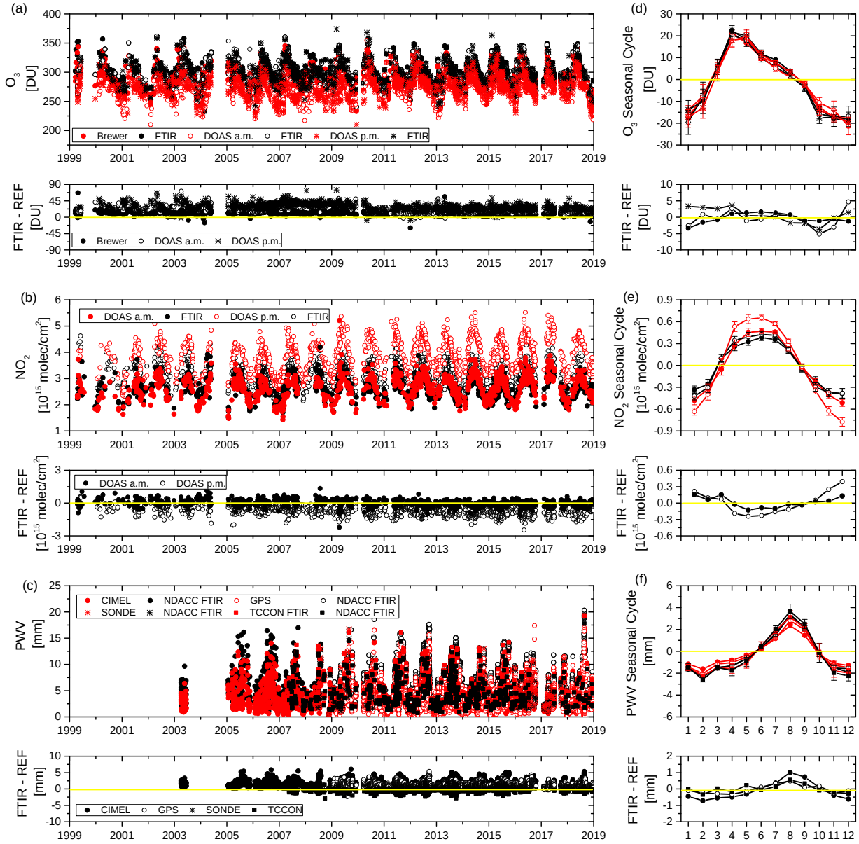
Figure 12. Time series of coincident NDACC FTIR TCs and IZO reference data sets, and of differences (FTIR - Reference, in absolute units) on left panels for: (a) O_3 , (b) NO_2 , and (c) PWV. Right panels show the averaged annual cycle of variations relative to the long-term background, from temporal decomposition analysis, and of differences for: (d) O_3 , (e) NO_2 , and (f) PWV. Error bars in annual cycles are standard errors of the monthly mean: 2 \times \sigma / \sqrt{n} , with \sigma the standard deviation and n the number of monthly measurements. Yellow line indicates zero value (i.e. no difference or no annual cycle signal).
