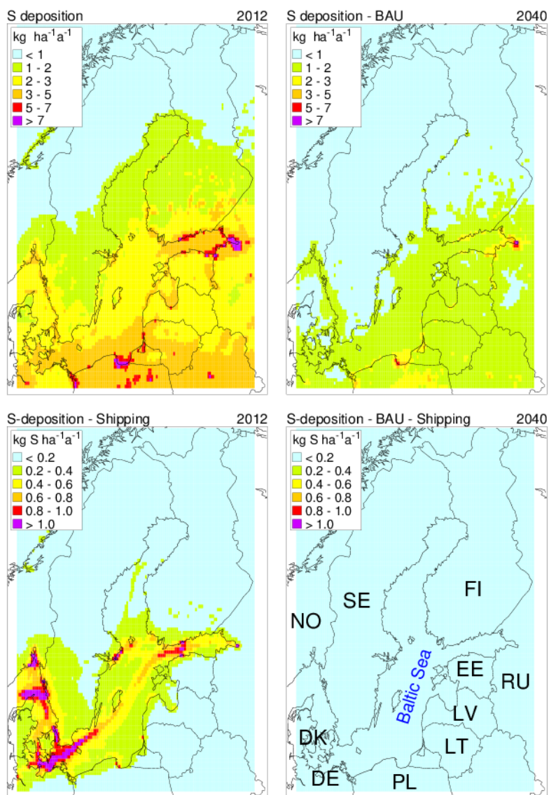
590 Figure 1. Top: Total deposition of S in 2012 (left) and in 2040 under the BAU scenario (right) in the extended Baltic sea region. Bottom: S deposition originating from shipping in 2012 (left) and in 2040 (right), calculated as the difference between the scenario based on total emissions and a scenario where shipping emissions are removed. In the bottom-right map the countries are labelled with their ISO-3166 2-letter codes.
