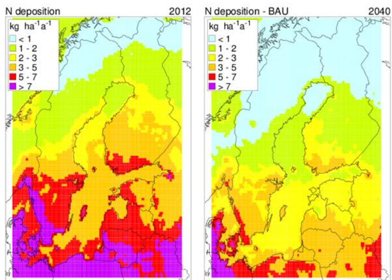
595 Figure 2. Total deposition of N deposition in 2012 (left) and the 2040-BAU scenario (right).
