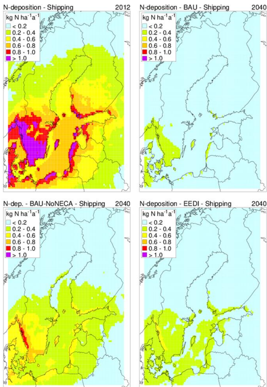
600 Figure 3. N deposition originating from shipping in 2012 (top left) and in 2040 (BAU top right, BAU-NoNECA bottom left, EEDI bottom right). Deposition from shipping was calculated as the difference between the scenario based on total emissions and the scenario where shipping has been removed.
