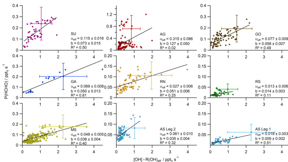
Figure 4: Scatter plots with bivariate fits (York et al., 2004) of the product [\text{OH}] \times R(\text{OH})_{\text{eff}} ( \pm 58\% ) versus the HCHO production rate P(\text{HCHO}) ( \pm 62\% ), subdivided into the different regions probed during the AQABA cruise. The slope of the respective regression represents the HCHO yield \alpha_{\text{eff}} , while the intercept can be interpreted as additional HCHO sources not related to OH chemistry ( P_{\text{add}}(\text{HCHO}) ).
