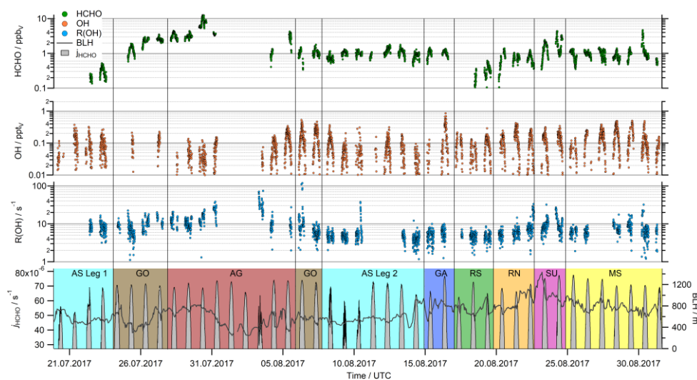
15 Figure 2: Time series of HCHO, OH, R(OH) and the HCHO photolysis ( j_{\text{HCHO}} , sum of the molecular and the radical channel) in 5 min resolution. For the boundary layer height (BLH) we used the ERA-5 meteorological reanalysis data in hourly averages, which resolves the earth's atmosphere on a 30 km grid ( https://www.ecmwf.int/en/forecasts/datasets/reanalysis-datasets/era5 ).
