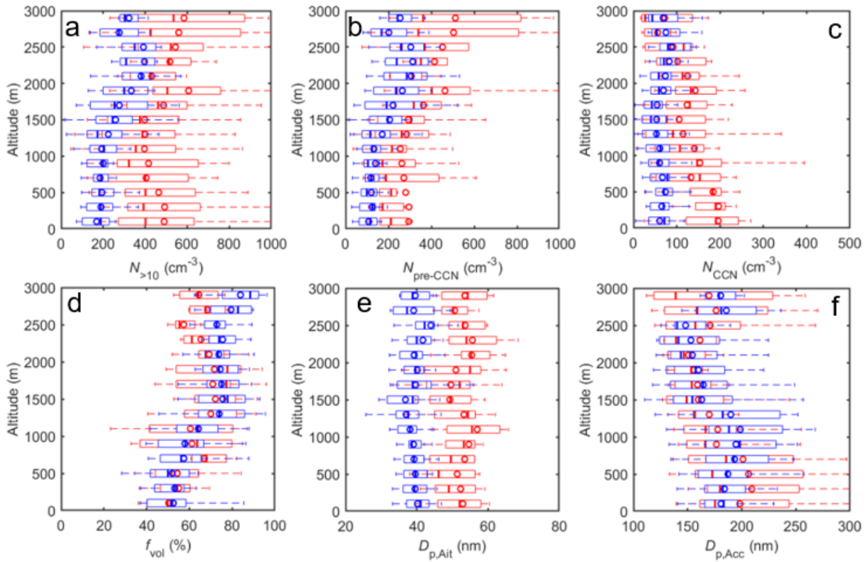
15 Fig. S2. Vertical profiles showing the (a) concentration of particles larger than 10 nm ( N_{>10} ), (b) concentration of Aitken-mode aerosols or aerosols too small to form cloud droplets ( N_{\text{pre-CCN}} ), (c) concentration of accumulation-mode aerosols or CCN ( N_{\text{CCN}} ), (d) aerosol volatile fraction ( f_{\text{vol}} ), (e) average size of Aitken-mode aerosol ( D_{\text{p,Ait}} ), and (f) average size of accumulation-mode aerosol ( D_{\text{p,Acc}} ) over the ENA site during the summer IOP (red) and winter IOP (blue). The data correspond to the periods when BC mass concentrations are below 5 \text{ ng m}^{-3} . The line and circle markers represent the median and mean of the data, and the edges of the box indicate the 25th and 75th percentiles, respectively.
