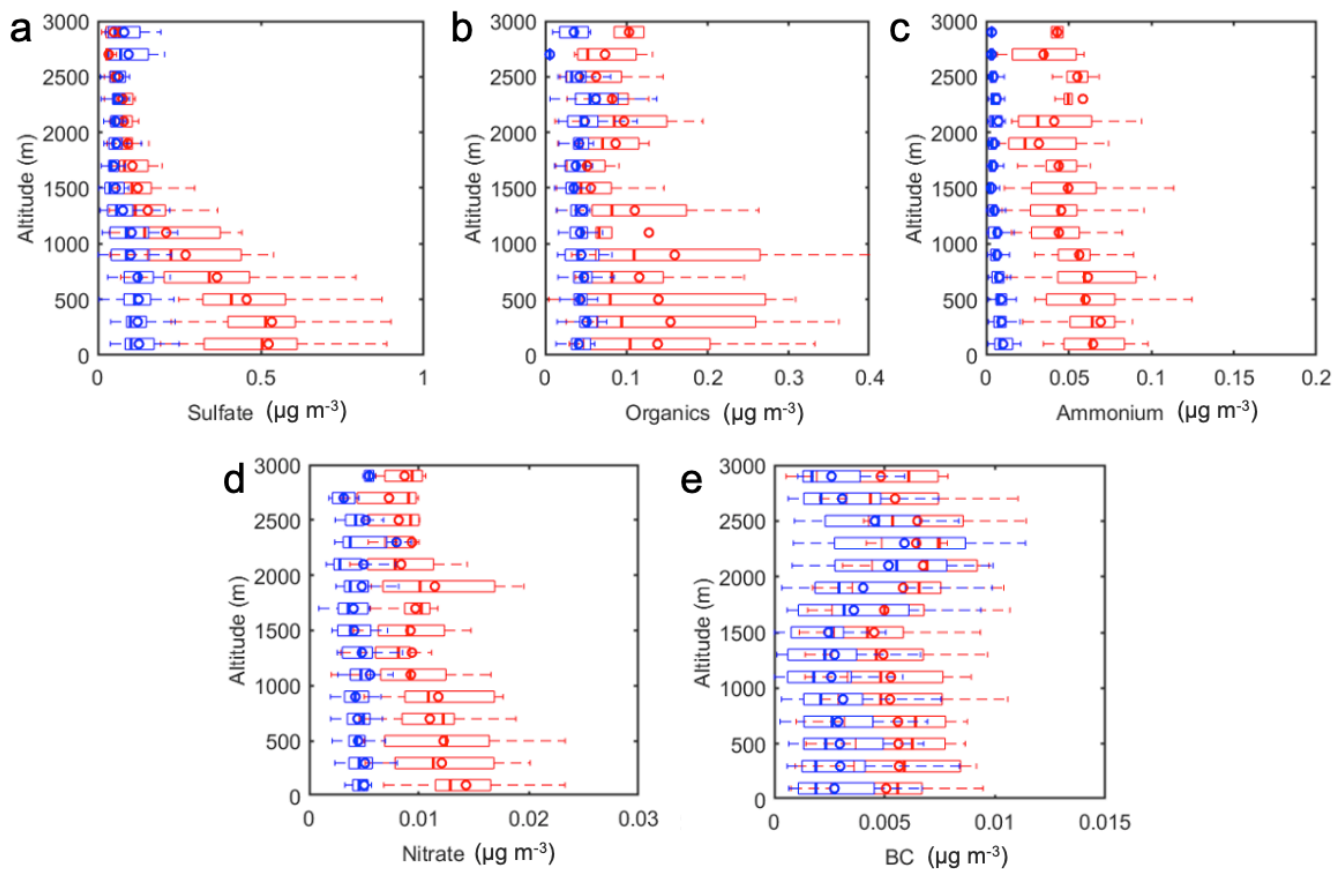
25 Fig. S3. Vertical profiles showing the mass concentrations of (a) sulfate, (b) organics, (c) ammonium, (d) nitrate, and (e) black carbon (BC) over the ENA site during the summer IOP (red) and winter IOP (blue). BC is measured by the SP2, and the rest of the compositions are measured by the HR-ToF-AMS. The data correspond to the periods when BC mass concentrations are below 5 \text{ ng m}^{-3} . The line and circle markers represent the median and mean of the data, and the edges of the box indicate the 25th and 75th percentiles, respectively.
