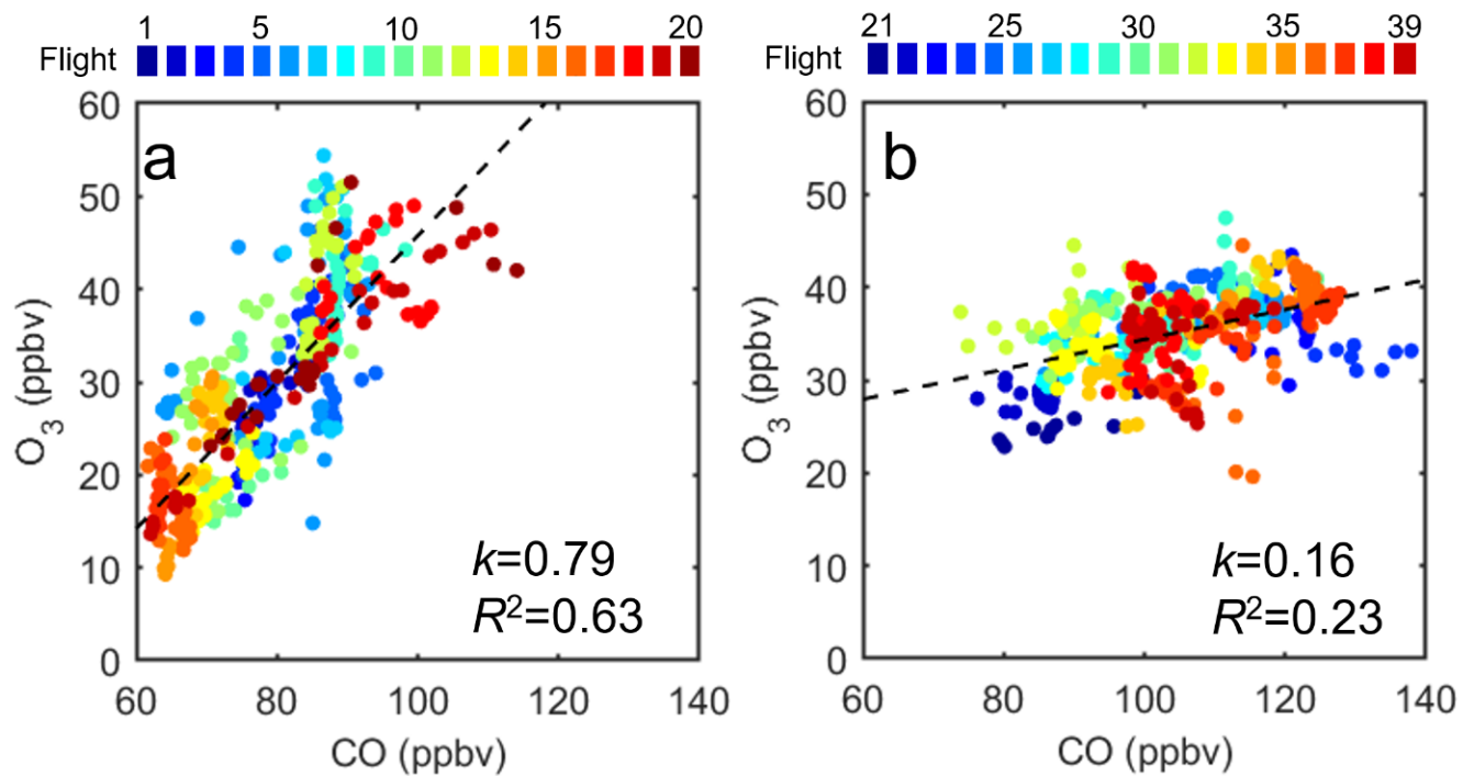
10 Fig. S1. Correlation between O_3 and CO during the (a) summer IOP and (b) winter IOP in the FT colored by flight number. The dashed lines show the linear fits of the data points.
