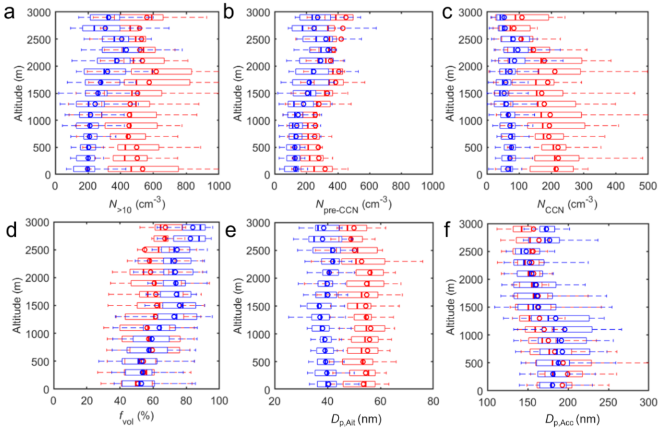
850 Fig. 6. Vertical profiles showing the (a) concentration of particles larger than 10 nm ( N_{>10} ), (b) concentration of Aitken-mode aerosols or aerosols too small to form cloud droplets ( N_{\text{pre-CCN}} ), (c) concentration of accumulation-mode aerosols or CCN ( N_{\text{CCN}} ), (d) aerosol volatile fraction ( f_{\text{vol}} ), (e) average size of Aitken-mode aerosol ( D_{\text{p,Ait}} ), and (f) average size of accumulation-mode aerosol ( D_{\text{p,Acc}} ) over the ENA site during the summer IOP (red) and winter IOP (blue). The concentrations are normalized to standard temperature and pressure (273.15 K and 101.325 kPa; STP). The line and circle markers represent the median and mean of the data, and the edges of the box indicate the 25th and 75th percentiles, respectively.
