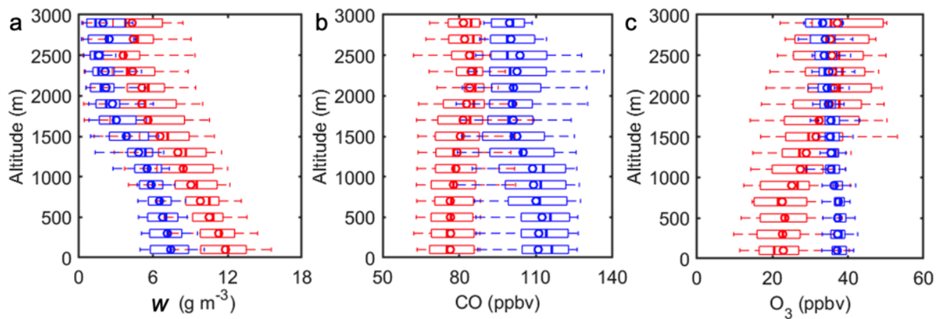
830 Fig. 4. Vertical profiles of (a) water vapor mixing ratio ( w ), (b) carbon monoxide mixing ratio (CO), and (c) ozone mixing ratio ( O_3 ) over the ENA site during the summer IOP (red) and winter IOP (blue). The mixing ratios are normalized to standard temperature and pressure (273.15 K and 101.325 kPa; STP). The line and circle markers represent the median and mean concentrations, and the edges of the box indicate the 25th and 75th percentiles, respectively.
