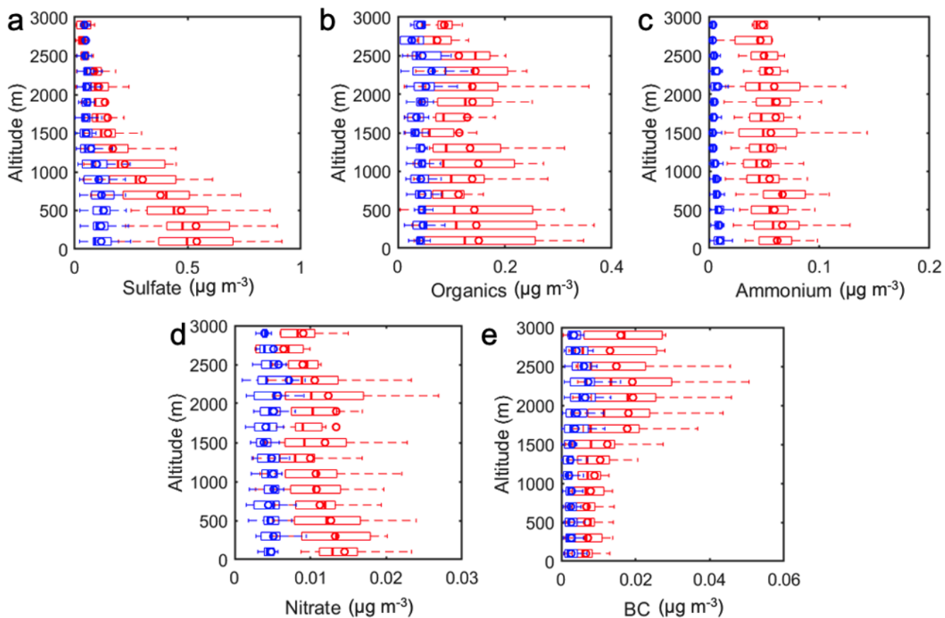
860 Fig. 7. Vertical profiles of the mass concentrations of (a) sulfate, (b) organics, (c) ammonium, (d) nitrate, and (e) black carbon (BC) in the ENA during the summer IOP (red) and winter IOP (blue). BC is measured by the SP2, and the rest of the compositions are measured by the HR-ToF-AMS. The line and circle markers represent the median and mean of the data, and the edges of the box indicate the 25th and 75th percentiles, respectively. The concentrations are normalized to standard temperature and pressure (273.15 K and 101.325 kPa; STP).
