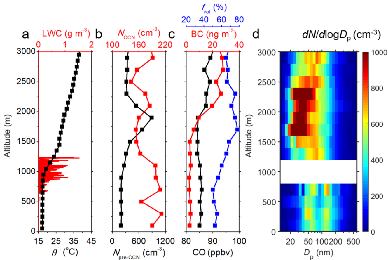
875 Fig. 9. Vertical profiles of parameters under the synoptic condition of Azores high on July 8, 2017. (a) Potential temperature ( \theta ) and liquid water content (LWC). (b) N_{\text{pre-CCN}} and N_{\text{CCN}} . (c) Concentrations of carbon monoxide (CO) and black carbon (BC), and aerosol volatile fraction ( f_{\text{vol}} ). (d) Vertical contour of aerosol size distributions as a function of altitude. Size distributions between 800 and 1200 m are not shown due to the interference of cloud droplet shattering. The CO mixing ratio, BC concentration, particle concentrations, and size distributions are normalized to standard temperature and pressure (273.15 K and 101.325 kPa; STP).
