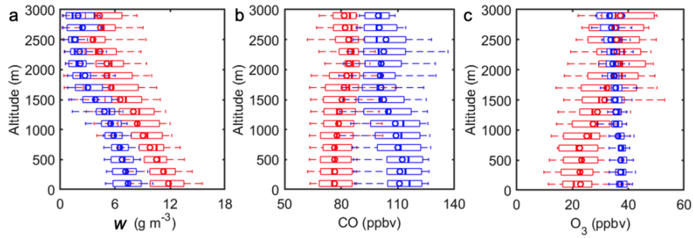
Fig. 4. Vertical profiles of (a) water vapor mixing ratio ( w ), (b) carbon monoxide mixing ratio (CO), and (c) ozone mixing ratio ( \text{O}_3 ) over the ENA site during the summer IOP (red) and winter IOP (blue). The mixing ratios are normalized to standard temperature and pressure (273.15 K and 101.325 kPa; STP). The line and circle markers represent the median and mean concentrations, and the edges of the box indicate the 25th and 75th percentiles, respectively.
