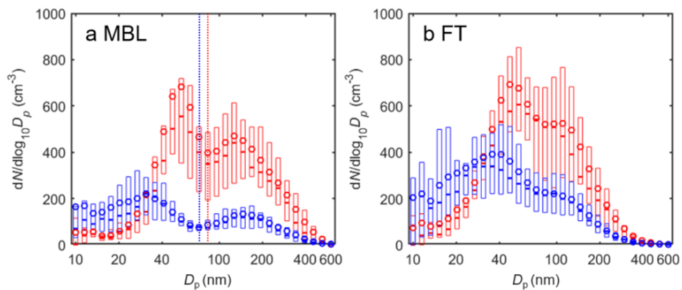
845 Fig. 5 Aerosol size distributions measured by the FIMS onboard the G-1 aircraft within (a) MBL and (b) lower FT during the summer IOP (red) and winter IOP (blue). The line and circle markers represent the median and mean of the size distribution, and the edges of the box indicate the 25th and 75th percentiles, respectively. The dotted lines in panel (a) show the Hoppel minimum for the averaged size distributions in the MBL.
