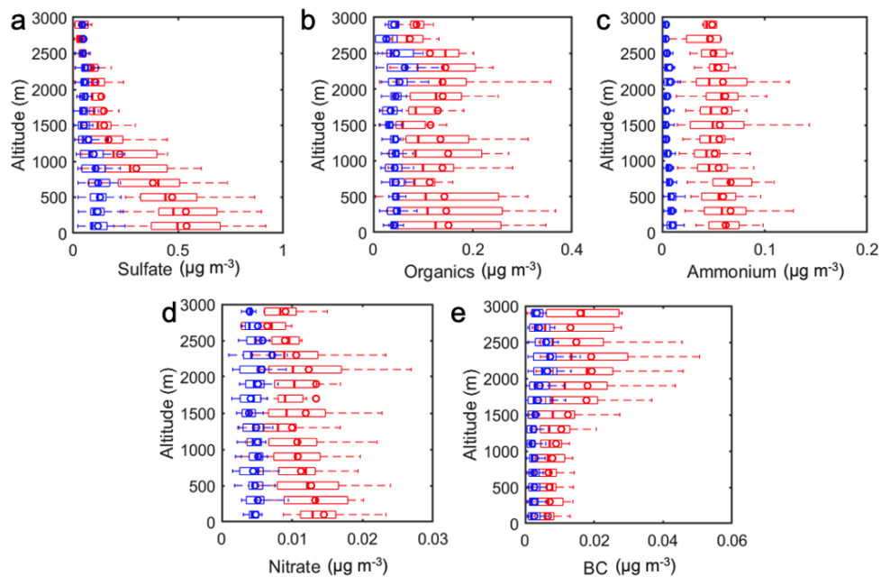
Fig. 7. Vertical profiles of the mass concentrations of (a) sulfate, (b) organics, (c) ammonium, (d) nitrate, and (e) black carbon (BC) in the ENA during the summer IOP (red) and winter IOP (blue). BC is measured by the SP2, and the rest of the compositions are measured by the HR-ToF-AMS. The line and circle markers represent the median and mean of the data, and the edges of the box indicate the 25th and 75th percentiles, respectively. The concentrations are normalized to standard temperature and pressure (273.15 K and 101.325 kPa; STP).
