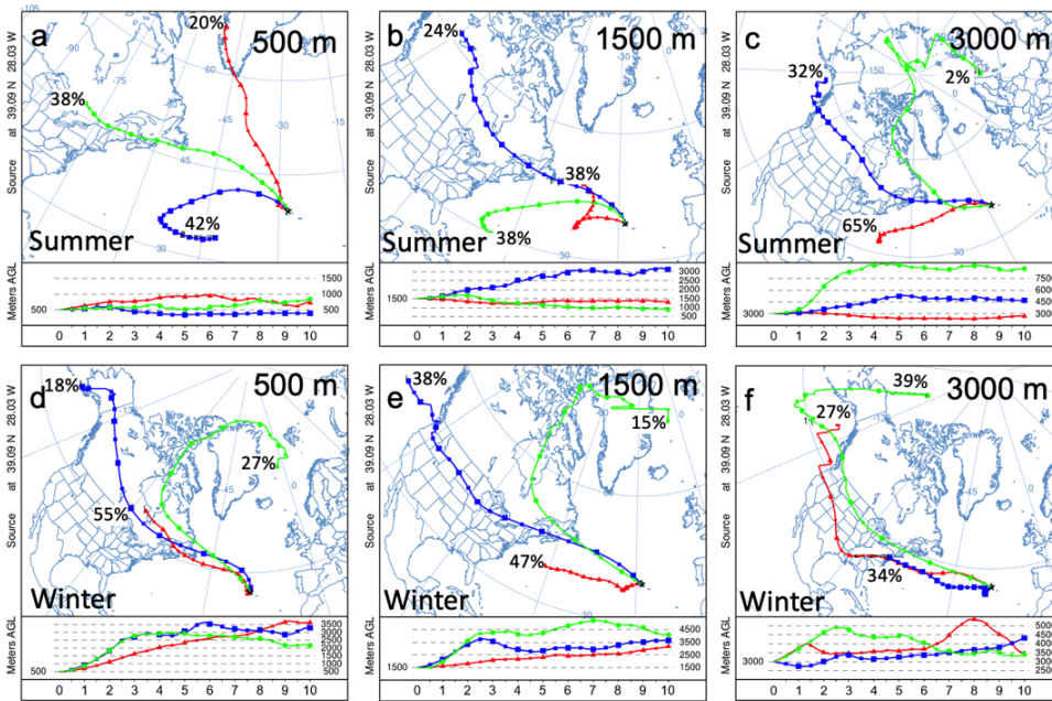
825 Fig. 3. Cluster analysis of 10-day back trajectories arriving at 500, 1500, and 3000 m above the ENA site during the summer (first row) and winter (second row) IOP. The average 10-day back trajectories of the three clusters are represented by different colors red, green, and blue lines, and the associated numbers denote the occurrence percentages of the clusters.
