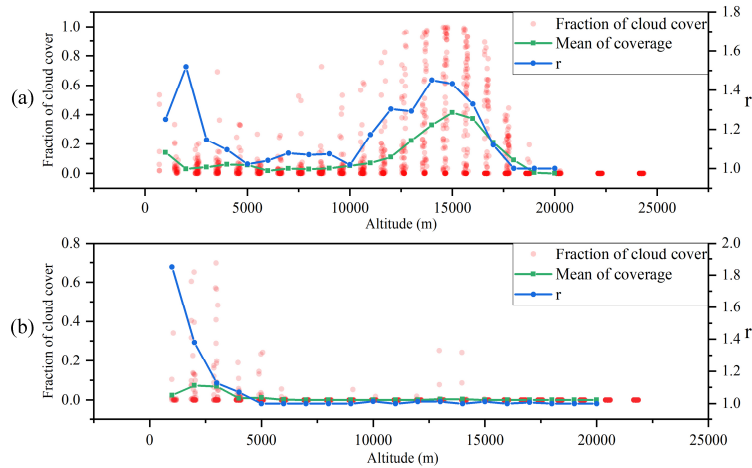
Figure 13. ERA5 cloud coverage of the valid Rayleigh channel data in the vertical direction. Data in (a) is from Qingyuan in July 2019, and in (b) is from Qingyuan in December 2019. The green line is the mean value of cloud coverage at different distance gates.
