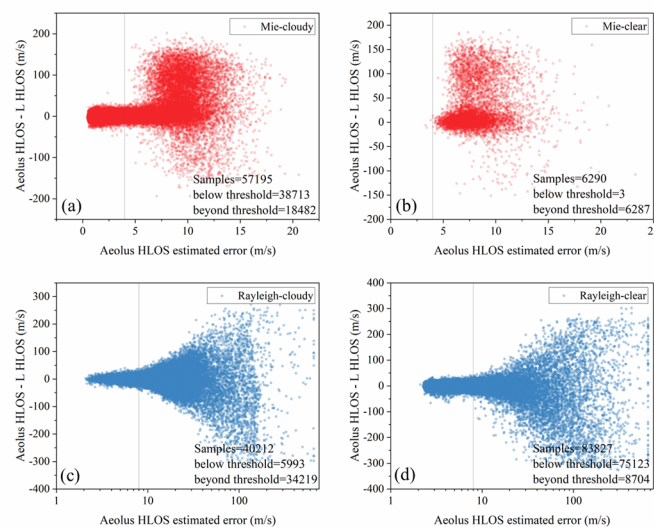
70 Figure 1. Difference between the Aeolus HLOS and L HLOS wind components as a function of estimated errors for (a) Mie-cloudy, (b) Mie-clear, (c) Rayleigh-cloudy, and (d) Rayleigh-clear. Samples mean the number of data points and the samples below or beyond the threshold are also listed. Reference lines are the screening threshold of estimated errors: 4 m/s (Mie) and 8 m/s (Rayleigh).
