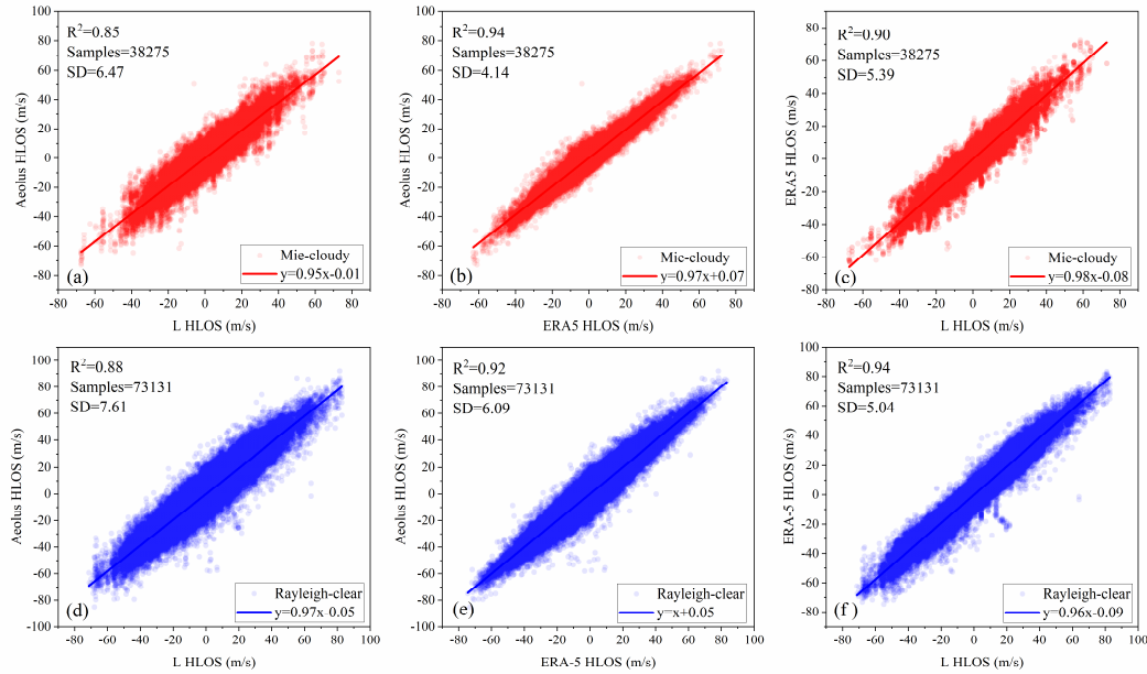
160 Figure 4. Comparison results of Aeolus, L-band RS, and ERA5 data in Mie-cloudy and Rayleigh-clear groups. (a, d) Aeolus vs L-band RS, (b, e) Aeolus vs ERA5, and (c, f) ERA5 vs L band RS
