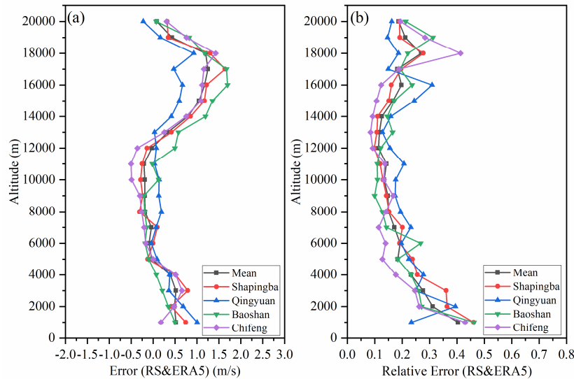
195 Figure 6. Vertical comparison of ERA5 and RS wind data for four regions. (a) Error and (b) Relative error
