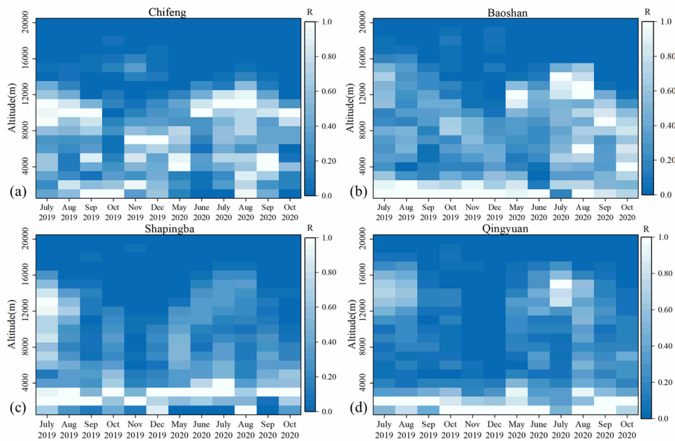
285 Figure 12. Vertical distribution of R values in different regions and months. (a) Chifeng, (b) Baoshan, (c) Shapingba, and (d) Qingyuan
