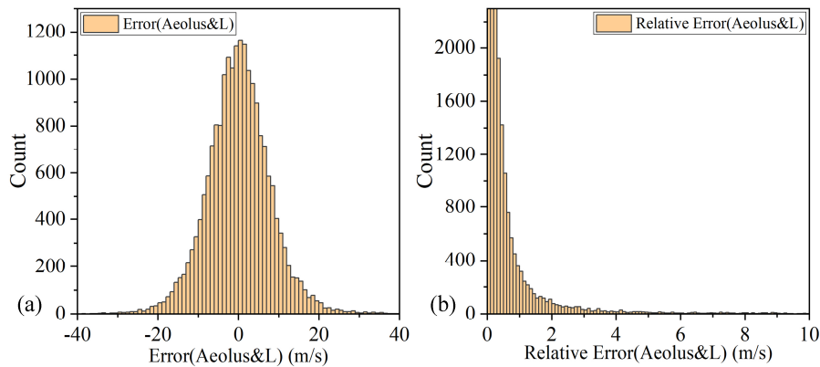
200 Figure 7. Statistical distribution of the error (a) and relative error (b) between Aeolus detection and L-band RS data. The data were from the Rayleigh-clear group for 12 months in Chifeng.
