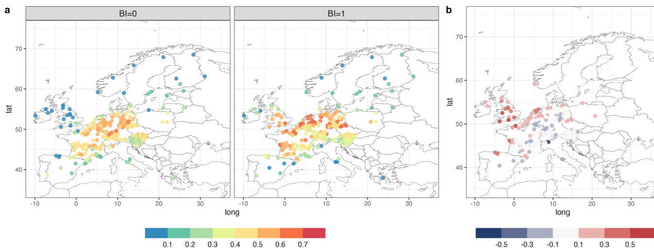
Figure 4. a) Spatial distribution of the upper tail dependence parameter derived from the copulas when BI=0 and BI=1. b) Differences between the values of the upper tail dependence parameter when BI=1 minus the values when BI=0.
