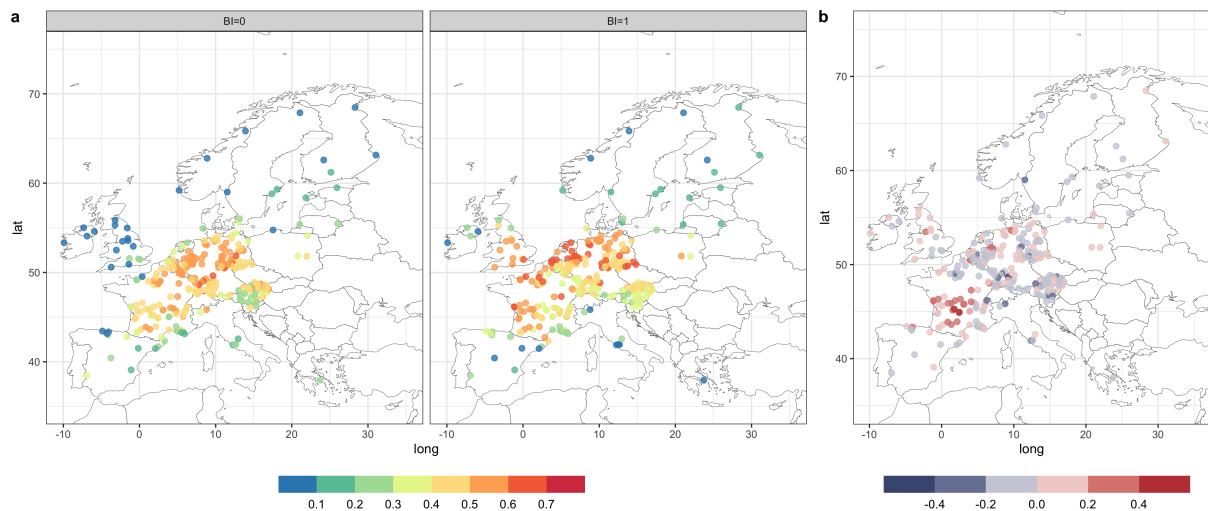
Figure 4. a) Spatial distribution of the upper tail dependence parameter derived from the copulas when BI=0 (left) and BI=1 (right) b) Differences between the values of the upper tail dependence parameter when BI=1 minus the values when BI=0.
