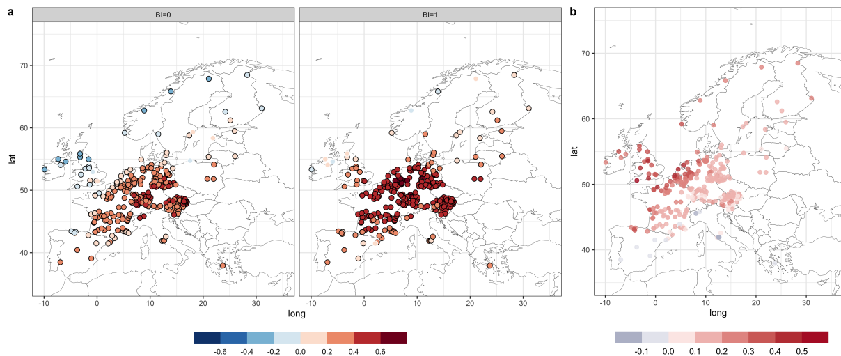
Figure 3. a): Spatial distribution of the Kendall's correlation coefficient between MDA8O 3 and Tmax under non blocking conditions (i.e. BI=0, left) and blocking conditions (i.e BI=1, right). Black contour indicates statistically significant anomalies at the 95% confidence level of a two-sided t test. b): Differences between the correlation values obtained when BI=1 minus the correlations when BI=0.
