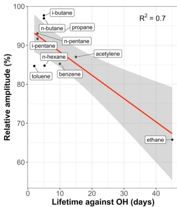
Figure S1: Mean seasonal amplitude, calculated as the relative difference between the winter maximum and the summer minimum, as a function of the lifetime of individual non-methane hydrocarbons against oxidation by the OH radical. The red line gives the fitted linear regression line with the 95 % confidence interval (grey shaded region).
