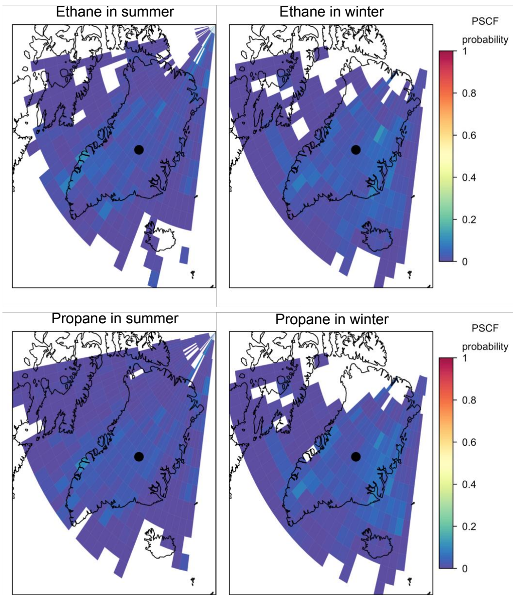
Figure S4: PSCF results for ethane and propane residuals greater than the 90 th percentile for April 2012-June 2019.
