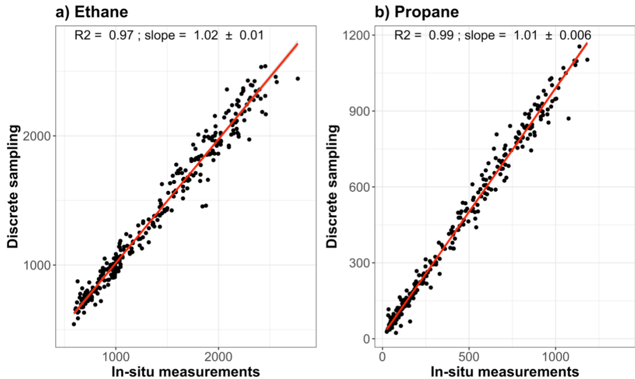
Figure S3: Scatter plot of daily averaged in-situ GC-FID measurements (x-axis) and discrete samples (y-axis) for a) ethane and b) propane. The red line gives the fitted linear regression. The slope ( \pm 95\% confidence interval) and correlation coefficient are given at the top. Note that these are not the same samples being compared: discrete samples are 5 minute-snapshots while in-situ GC-FID measurements are daily averages of 6-12 20 minute-samples.
