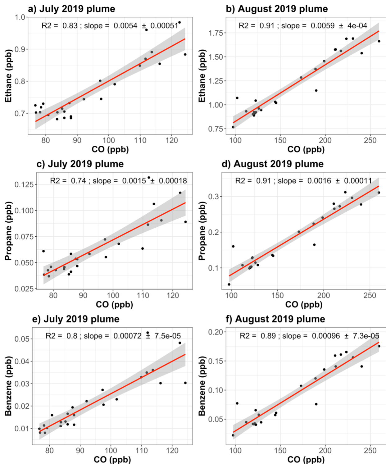
Figure S5: Scatter plot of ethane, propane, and benzene vs. carbon monoxide (CO) mixing ratios in the July and August 2019 biomass burning plumes observed at GEOSummit. The red line gives the fitted linear regression line with the 95 % confidence interval (grey shaded region). The slope, given at the top, gives the emission ratio (amount of compound emitted divided by that of a reference compound (CO here)).
