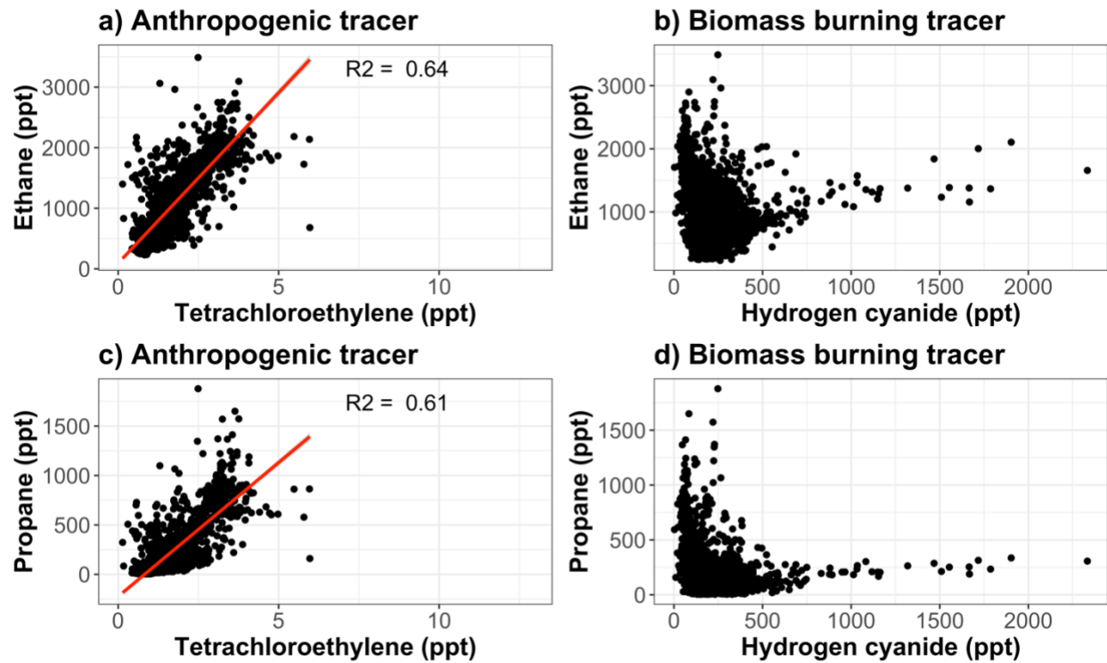
Figure S6: Scatter plot of ethane (a, b) and propane (c, d) vs. tetrachloroethylene and hydrogen cyanide mixing ratios in the remote free troposphere during the global-scale aircraft mission ATom. Tetrachloroethylene and hydrogen cyanide are used as tracers of anthropogenic and biomass burning emissions, respectively. The red line gives the fitted linear regression line with the 95 % confidence interval (grey shaded region). The correlation coefficient is given at the top.
