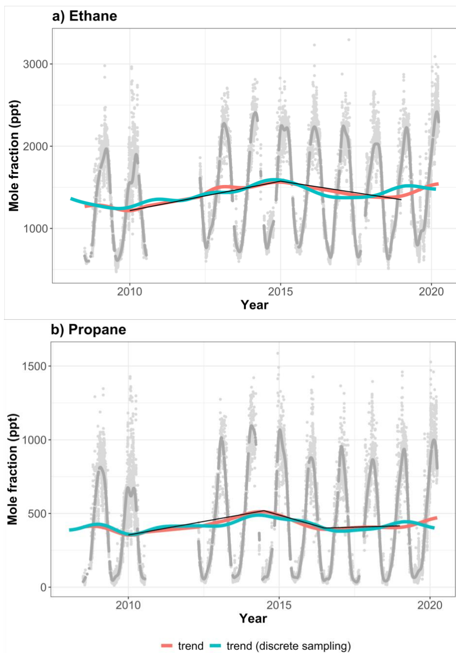
Figure S2: a) Ethane, and b) propane time-series at GEOSummit from July 2008 to March 2020. Individual data points are shown in light grey, smoothed fit in dark grey, and trends in salmon. Trends inferred from discrete flask sampling are shown in turquoise. The slopes given by the Theil-Sen test for trend analysis are shown in black.
