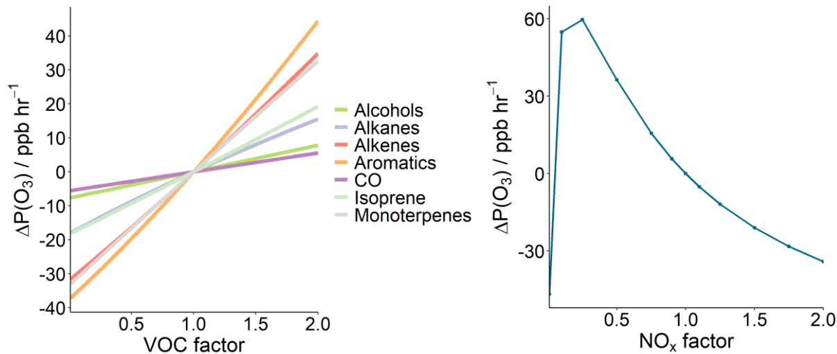
555 Figure 10: Modelled mean morning (08:00 – 12:00) change in P(O 3 ) rate for CO and six VOC classes upon varying their concentrations by multiplying by factor, “VOC factor” (left) and by vary just NO x (right).
