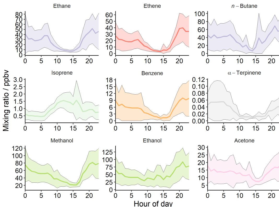
Figure 6: Mean campaign averaged diel mixing ratio profiles of selected VOCs during the campaign: ethane, ethene, n-butane, 430 isoprene, benzene, \alpha -terpinene, methanol, ethanol, acetone. The shaded ribbon represents one standard deviation from the mean. Colours correspond to the different VOC classes.
