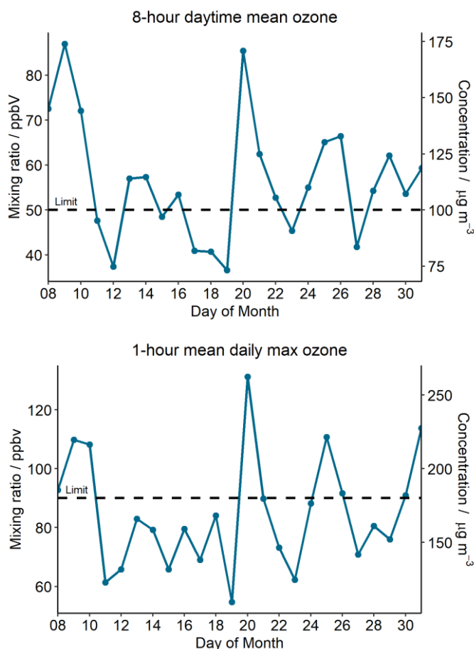
Figure 4: 8-hour mean O 3 concentration between 09:00 and 17:00 IST (top) and hourly averaged maximum daily O 3 concentration (bottom) during October 2018. The black dashed line is the prescribed national standards for O 3 .
