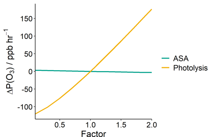
580 Figure 11: Impact of varying photolysis rates and aerosol surface area (ASA) on mean modelled morning O 3 production rates, ΔP(O 3 ) (08:00 – 12:00).
