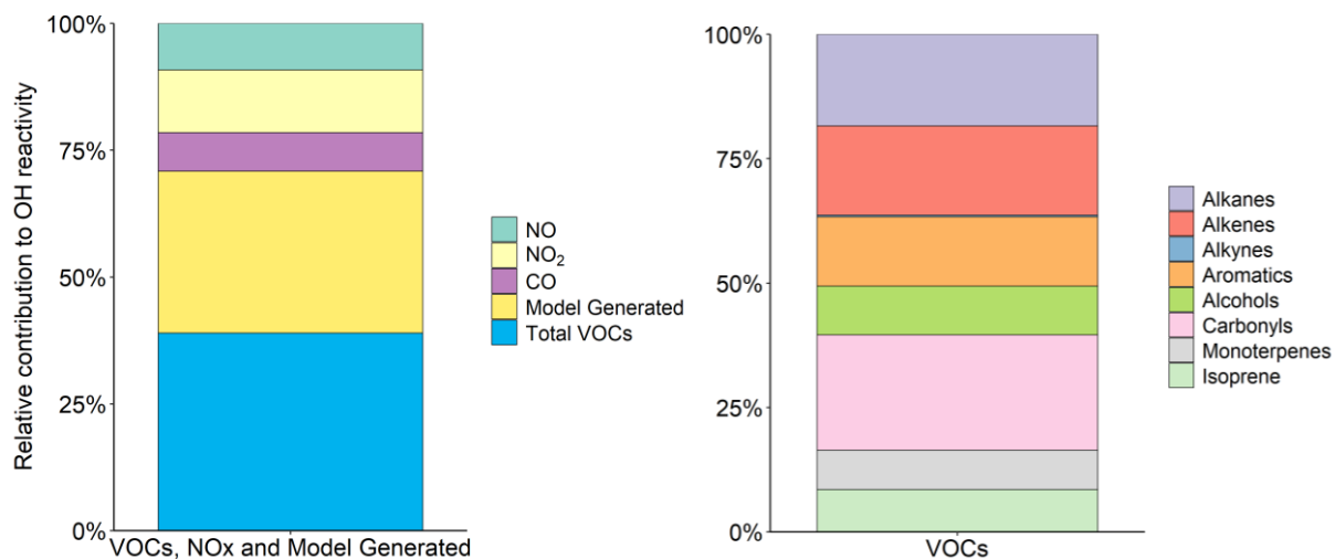
475 Figure 8: Relative contribution of species classes to average morning OH reactivity, k(\text{OH}) , (08:00-12:00). The contribution of each group to the total k(\text{OH}) including NO x and model generated species (left) and the contribution of each class to just the VOC proportion of k(\text{OH}) (right).
