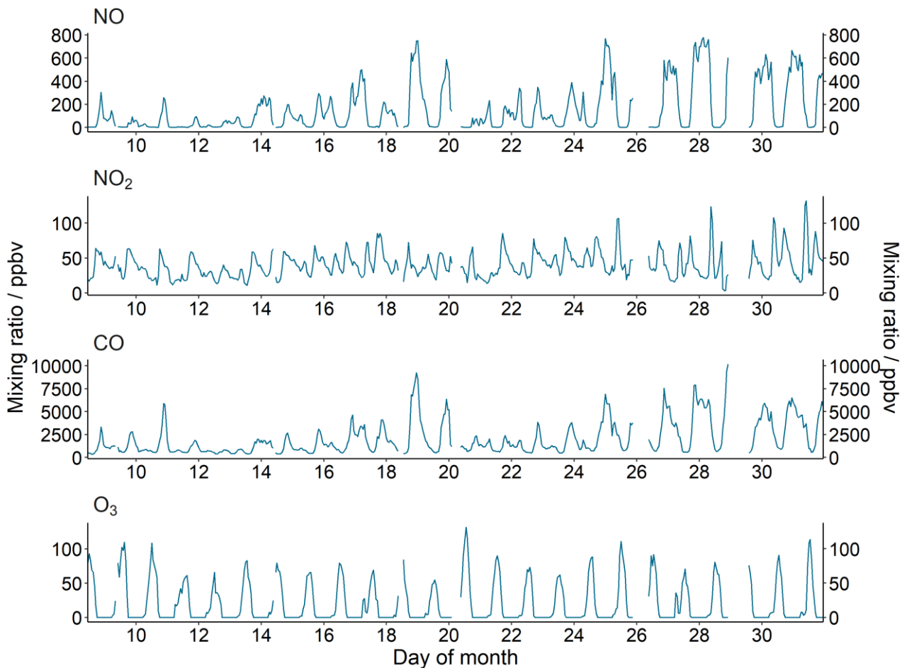
345 Figure 2: Observed mixing ratio timeseries of (from top to bottom): NO, NO 2 CO and O 3 during October 2018.
