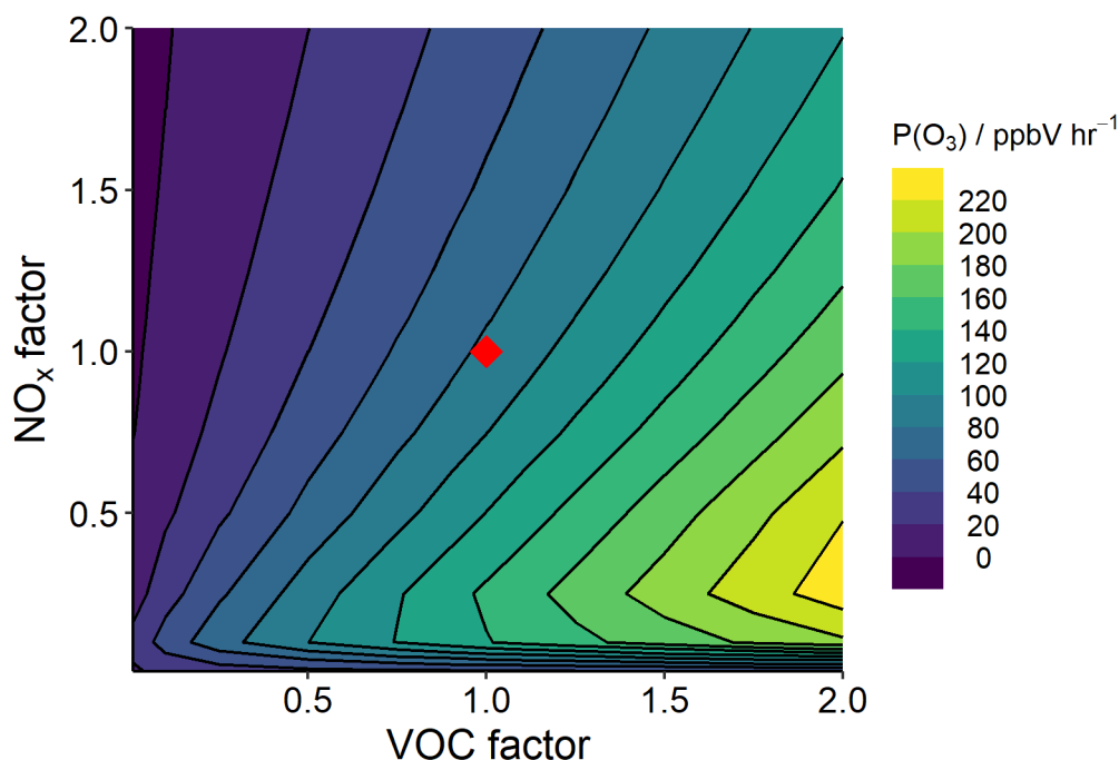
Figure 9: Mean modelled \text{O}_3 production, P(\text{O}_3) , isopleth between 08:00 and 12:00 based on varying VOC and \text{NO}_x concentrations in the model. The red diamond at point 1,1 represents modelled P(\text{O}_3) at observed VOC and \text{NO}_x concentrations.
