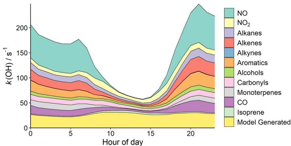
465 Figure 7: Diel profile of campaign averaged VOCs, CO and \text{NO}_x contributions to OH reactivity, k(\text{OH}) .
