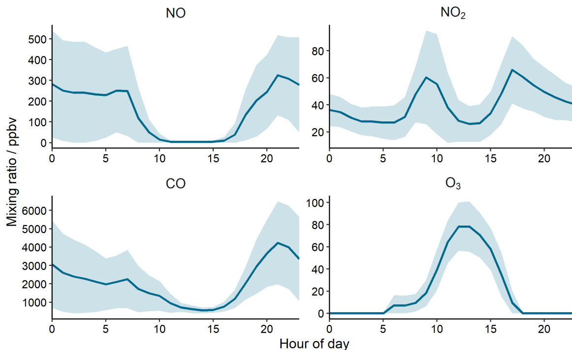
360 Figure 3: October campaign averaged diel profiles. The shaded ribbon represents the standard deviation of this average.
