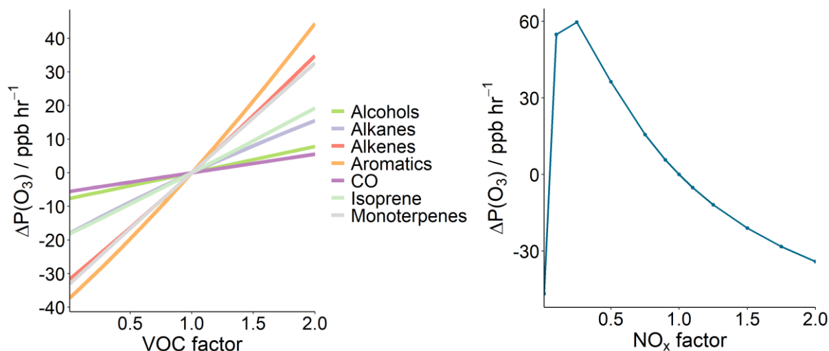
555 Figure 10: Modelled mean morning (08:00 – 12:00) change in \text{P}(\text{O}_3) rate for CO and six VOC classes upon varying their concentrations by multiplying by factor, “VOC factor” (left) and by vary just \text{NO}_x (right).
