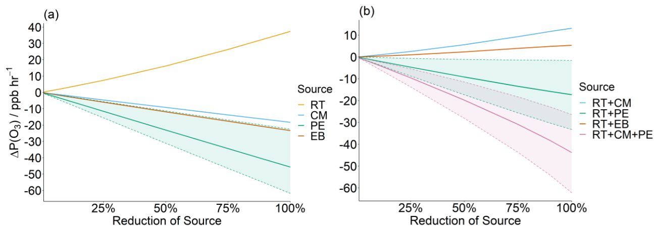
660 Figure 12: Change in P(O 3 ) on reducing road transport (RT), combustion for manufacturing (CM), process emissions (PE) 665 and energy for buildings (EB) (left); and (right) reducing road transport simultaneously along with either i) CM, ii) PE, iii) EB, iii) CM and PE. The shaded region, bounded by a dashed line, represents the variability in ΔP(O 3 ) when 0-100 % of observed monoterpenes contribute to anthropogenic EDGAR source sectors that include PE. The solid lines represent the base case whereby 50 % of monoterpenes are assumed to be from anthropogenic sources described in the EDGAR inventory (the other 50 % is assumed to be from biogenic sources).
