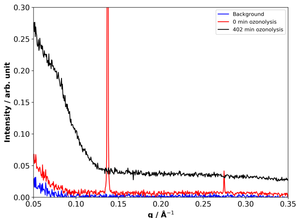
Figure S8. SAXS patterns of a levitated acid-soap complex before and after ozonolysis compared with an empty-levitator background. There is a clear increase in low- q scattering as a result of ozonolysis. [\text{O}_3] = 52 \pm 0.5 ppm.
