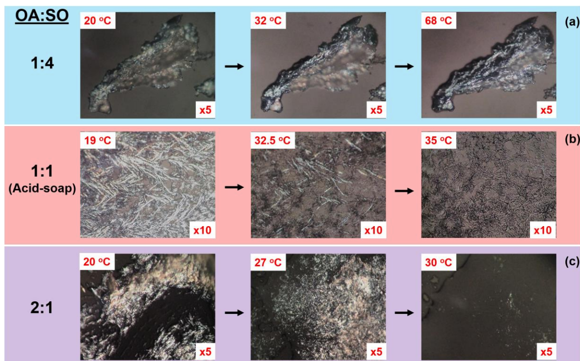
Figure S5. Polarising microscopy-temperature experiments of differing oleic acid:sodium oleate weight ratios deposited from ethanol onto microscope slides. OA = Oleic acid, SO = Sodium oleate. (a) 1: 4, (b) 1:1 (acid-soap complex) and (c) 2:1. RH \sim 50\% .
