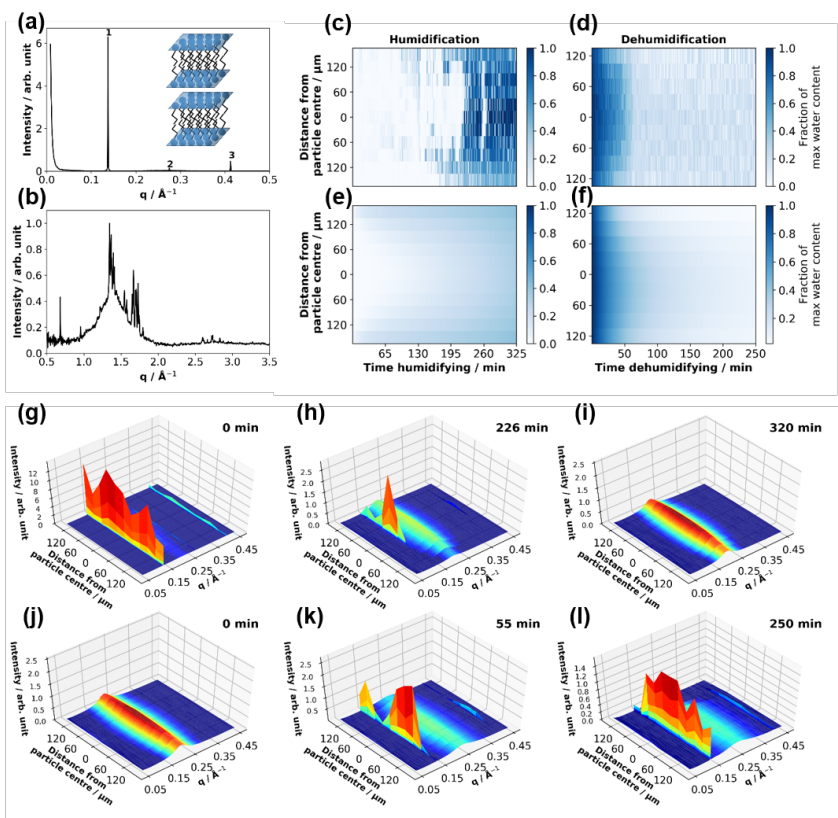
Figure 1. ((a) and (b)) 1-D SAXS and WAXS patterns obtained from a dry levitated particle of the acid-soap complex – 1 st , 2 nd and 3 rd lamellar peaks are labelled and a cartoon of the lamellar phase is presented (a). ((c) and (d)) experimental fraction of maximum water content as a function of distance from particle centre and time humidifying/dehumidifying. ((e) and (f)) modelled fraction of maximum water content – best fits to experimental data for humidification and dehumidification. 3-D surface plots of 1-D SAXS patterns plotted against distance from the particle centre for the same particle humidifying ((g) – (i)) and dehumidifying ((j) – (l)) with time humidifying/dehumidifying presented at the top right of each plot (particle size: ~ 150 \mu\text{m} (vertical radius) x 500 \mu\text{m} (horizontal radius); humidification experiment: ~ 38 % (room RH) ((g)) to 90 % ((h) and (i)) RH, dehumidification experiment: 90 % ((j) to ~ 38 % ((k) and (l)) RH).
