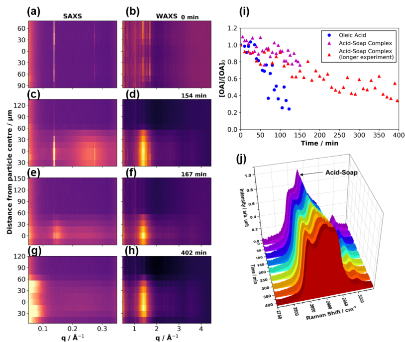
345 Figure 2. Vertical scans through the particle showing the effect of ozonolysis on self-assembly. Each row of plots ((a) and (b), (c) and (d), (e) and (f), (g) and (h)) shows simultaneous 1-D SAXS and WAXS scattering patterns vs. distance from the particle centre (measured in \mu\text{m} from what was deemed the particle centre from attenuation data) at increasing time exposed to ozone (labelled at the top-right of every WAXS plot). The particle moved and possibly changed shape during the experiment, vertical movement is apparent from the SAXS and WAXS patterns. (i) Comparison of a levitated pure oleic acid droplet vs. a levitated acid-soap complex particle undergoing ozonolysis, measured by Raman microscopy - A longer ozonolysis experiment on a different levitated acid-soap complex particle is also presented, totalling two ozonolysis experiments on this proxy . (j) Evolution of the Raman spectra between 2750 and 3050 \text{cm}^{-1} of a levitated acid-soap complex during ozonolysis. (Particle size: \sim 85 \mu\text{m} (vertical radius) \times \sim 500 \mu\text{m} (horizontal radius); [\text{O}_3] = 51.9 \pm 0.5 \text{ ppm} ).
