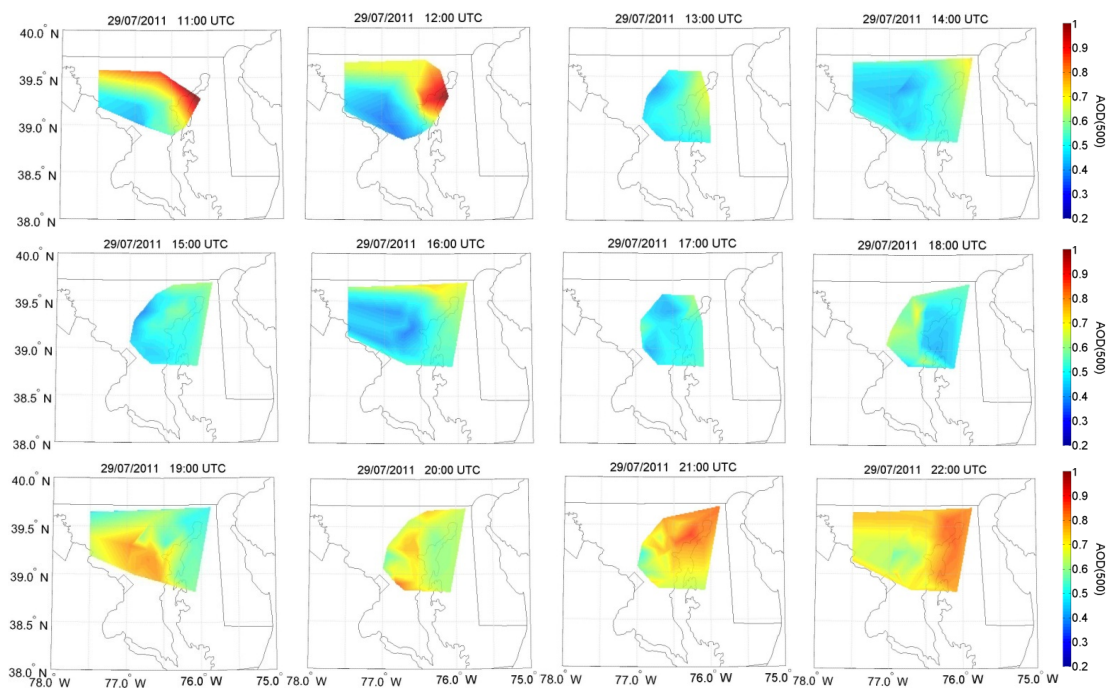
Figure 11: Temporal evolution of aerosol optical depth (AOD) at 500 nm from AERONET-DRAGON over the Washington-Baltimore area on 29th July 2011.
