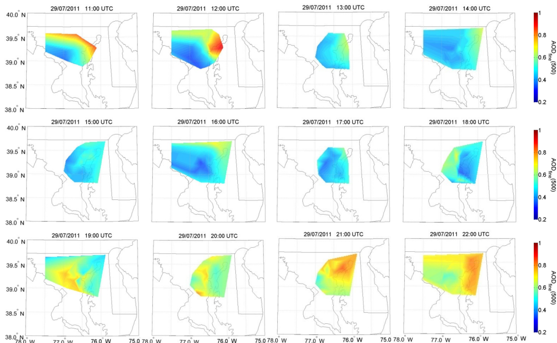
Figure 12: Temporal evolution of fine mode aerosol optical depth ( AOD_{fine} ) at 500 nm from AERONET-DRAGON over the Washington-Baltimore area on 29th July 2011
