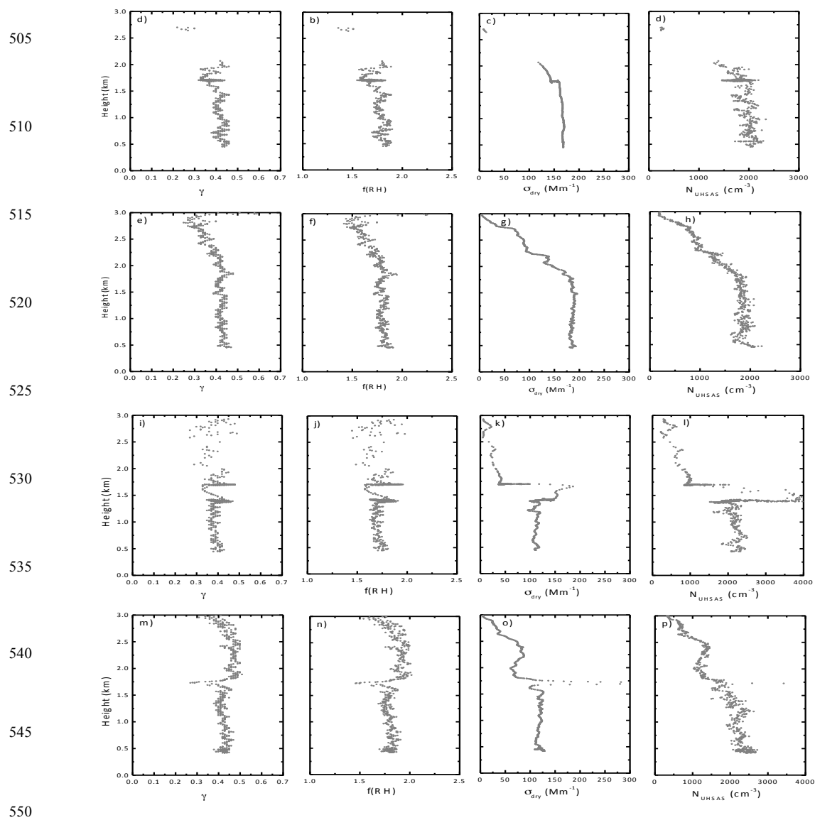
Figure 7: Vertical profiles of hygroscopicity parameter \gamma and F(RH) , scattering coefficient at dry conditions ( \sigma_{dry} ) and number of particles from UHSAS ( N_{UHSAS} ) acquired from the P-3B airplane over GSFC-HUBC region on (a) 29 th July spiral-down, (b) 29 th July spiral-up, (c) 22 nd July spiral-down and (d) 22 nd July spiral-up
