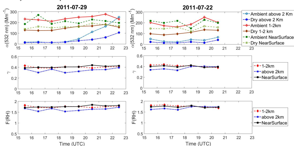
780 Figure 14: Hourly mean values of aerosol extinction at 532 nm ( \alpha(532 \text{ nm}) ) and hygroscopicity parameters \gamma and F(\text{RH}) for both 29 th and 22 nd July. Data are presented for three different altitudes: Near surface (altitude below 1 km), in planetary boundary layer (1-2 Km for 29 th July and 1-1.8 Km for 22 nd July) and above the planetary boundary layer (>2.0 Km for 29 th July and > 1.8 Km for 22 nd July).
