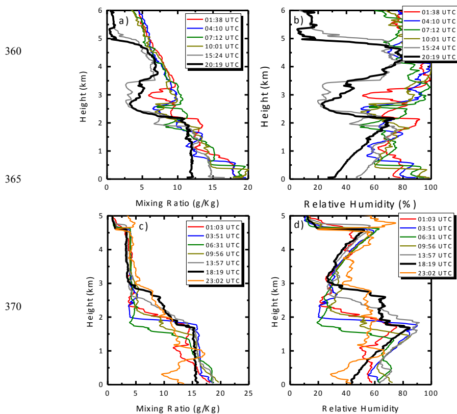
375 Figure 3: Water vapor mixing ratio and relative humidity profiles obtained from radiosondes launched at HUBC on (a-b) 29 th July 2011 and on (c-d) 22 nd July 2011.
