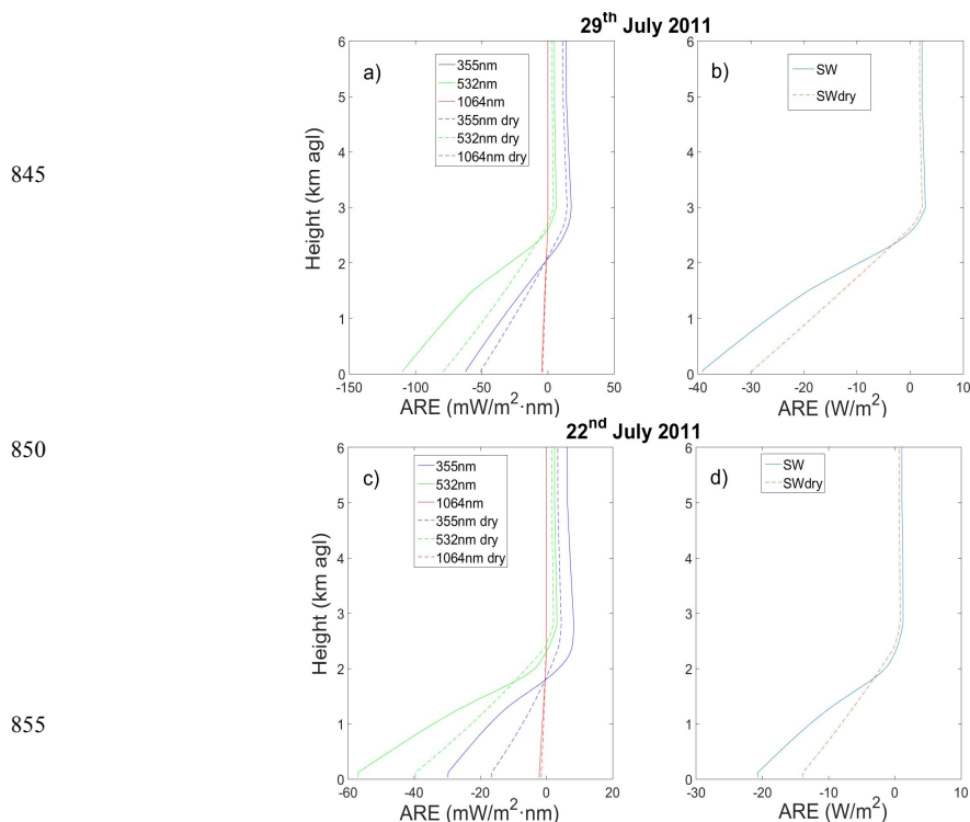
Figure 17: Vertical profiles of aerosol radiative effect (ARE) from the lidar measurements affected by aerosol hygroscopic growth. Data are presented (left) for the measured lidar measurements (355, 532 and 1064 nm) and (right) integrated for the shortwave range (280 – 860 3000 nm).
