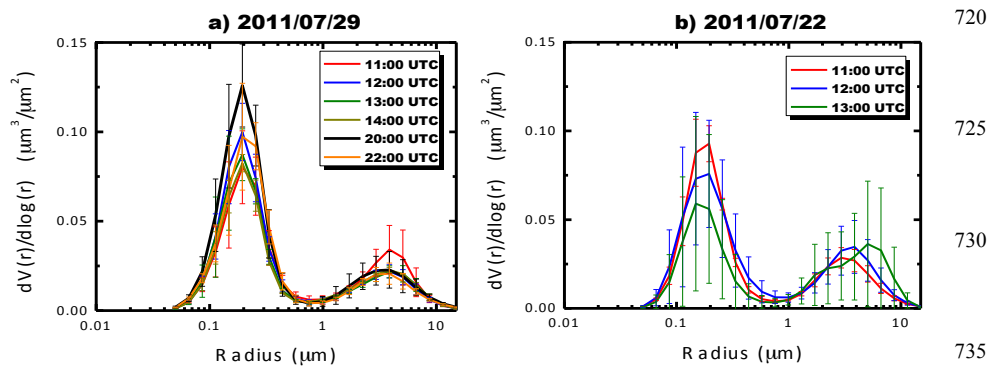
Figure 13: Mean hourly values of aerosol size distributions from AERONET-DRAGON stations over the Washington-Baltimore region on (a) 29 th July 2011 and (b) 22 nd July 2011.
