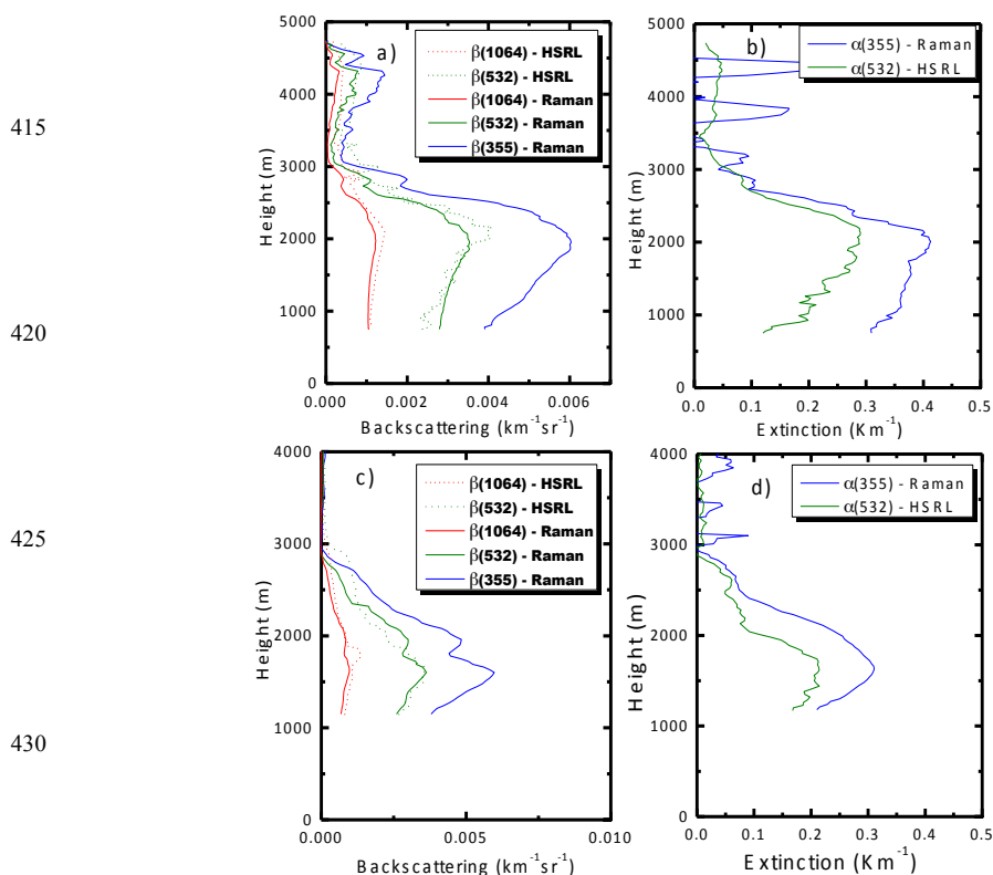
435 Figure 5: Vertical profiles of backscattering ( \beta ) and extinction ( \alpha ) measurements obtained by ground-based Raman lidar and airborne HSRL-1 at NASA Goddard Space Flight Center on (a-b) 29 th July 2011 at 20:00 UTC and on (c-d) 22 nd July 2011 at 18:35 UTC. The ground-based Mie-Raman measurements provided independent measurements of backscattering and extinction coefficients at 355 nm, while the airborne HSRL-1 system provide those for 532 nm. For 1064 nm both instruments provide only backscattering measurements.
