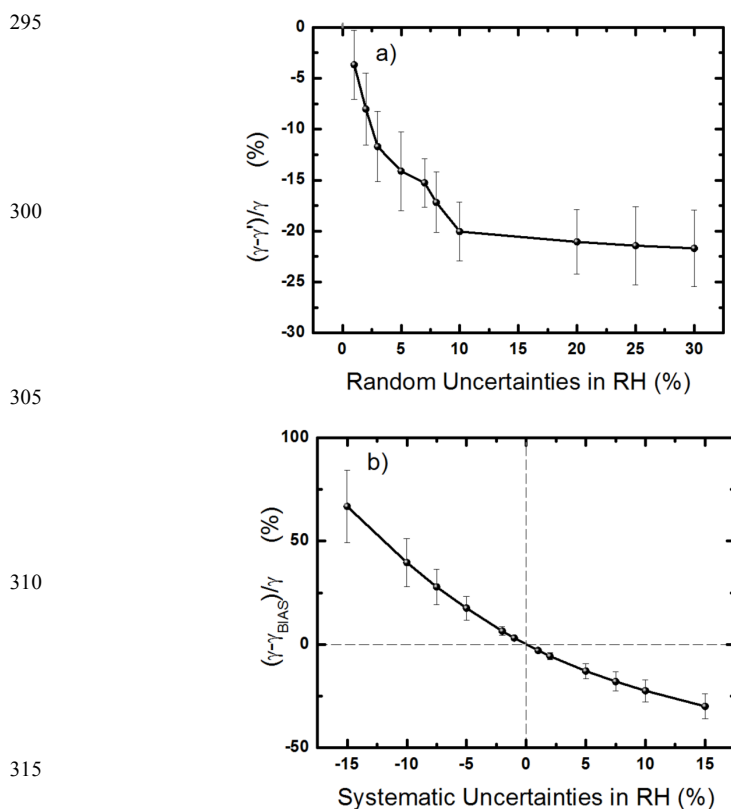
Figure 2: Sensitivity analyses of the hygroscopic growth parameter ' \gamma ' as function of (a) random errors in the relative humidity and (b) systematic errors in relative humidity
