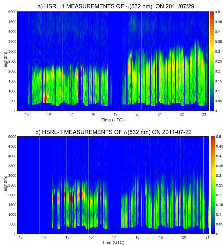
665 Figure 10: Temporal evolution of aerosol extinction coefficient ( \alpha ) at 532 nm obtained by HSRL-1 system over the Baltimore-Washington area on (a) 29 th July 2011 and (b) 22 nd July 2011. Vertical white lines represents times when the system flew over NASA Goddard Space Flight Center
