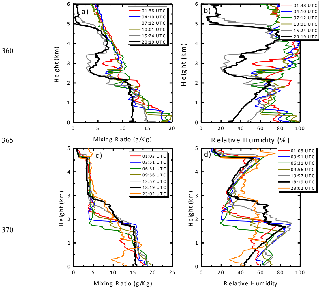
Figure 3: Water vapor mixing ratio and relative humidity profiles obtained from radiosondes launched at HUBC on (a-b) 29 th July 2011 and on (c-d) 22 nd July 2011.
