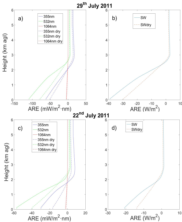
875 Figure 17: Vertical profiles of aerosol radiative effect (ARE) from the lidar measurements affected by aerosol hygroscopic growth. Data are presented (left) for the measured lidar measurements (355, 532 and 1064 nm) and (right) integrated for the shortwave range (280 – 3000 nm).
