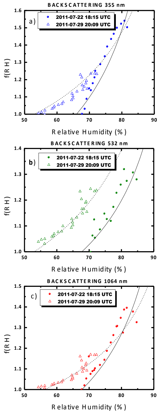
Figure 6: Humidigrams of f(\text{RH}) versus relative humidity for the aerosol backscattering data obtained on 29th July 2011 and on 22nd July 2011. Data are presented at the wavelengths of (a) 355 nm, (b) 532 nm and (c) 1064 nm.
