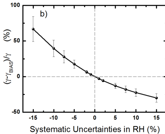
Figure 2: Sensitivity analyses of the hygroscopic growth parameter ' \gamma ' as function of (a) random errors in the relative humidity and (b) systematic errors in relative humidity
