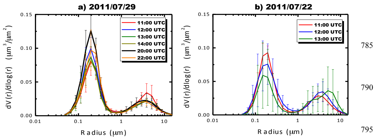
785 790 795 Figure 16 Mean hourly values of aerosol size distributions from AERONET-DRAGON stations over the Washington-Baltimore region on (a) 29 th July 2011 and (b) 22 nd July 2011.
