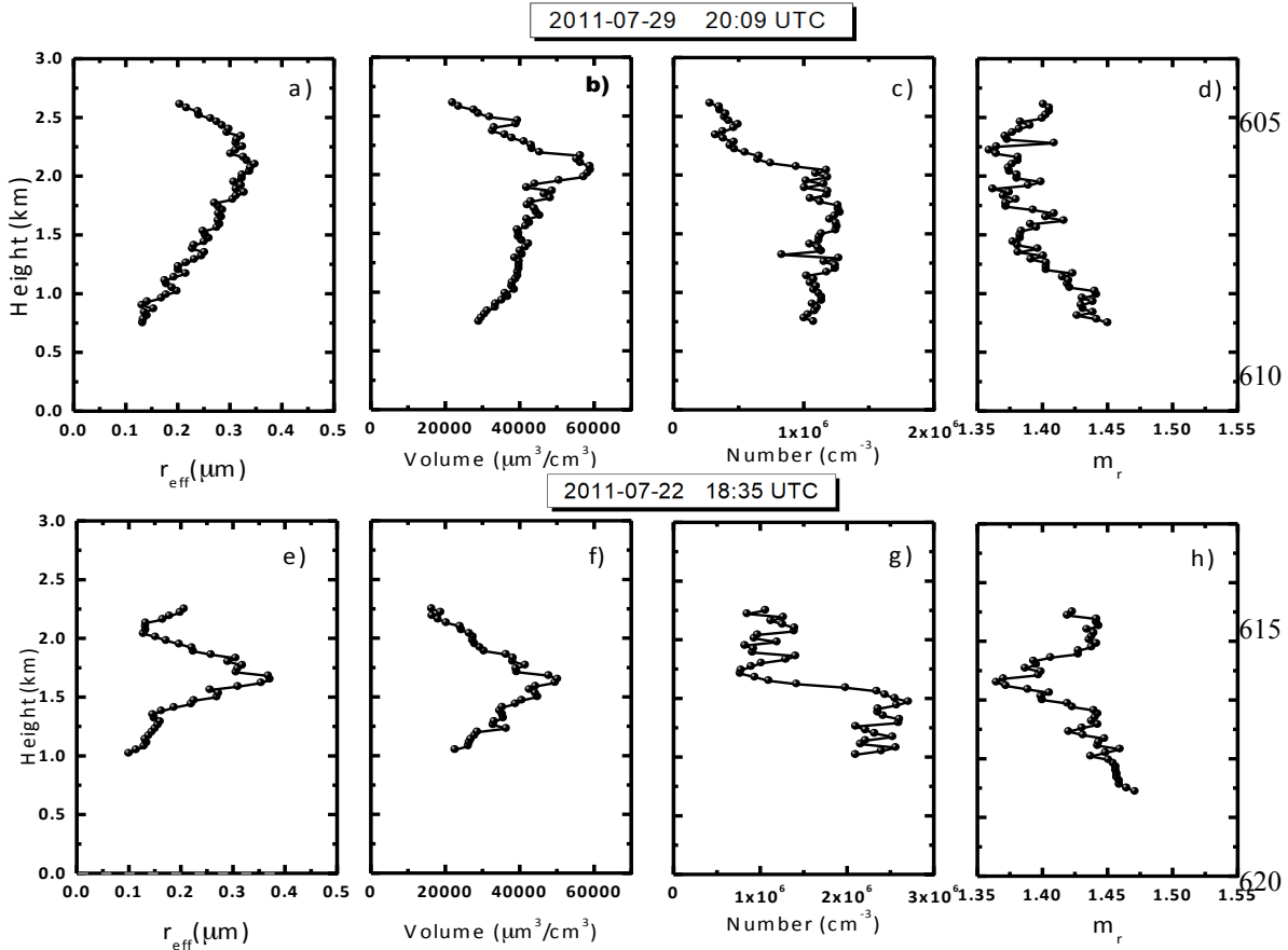
Figure 8: Retrieved effective radius ( r_{eff} ), volume and number concentrations and real part of refractive index ( m_r ) from the stand-alone 3\beta+2\alpha lidar inversion for (a-d) 29 th July 2011 and for (e-f) 22 nd July 2011.
