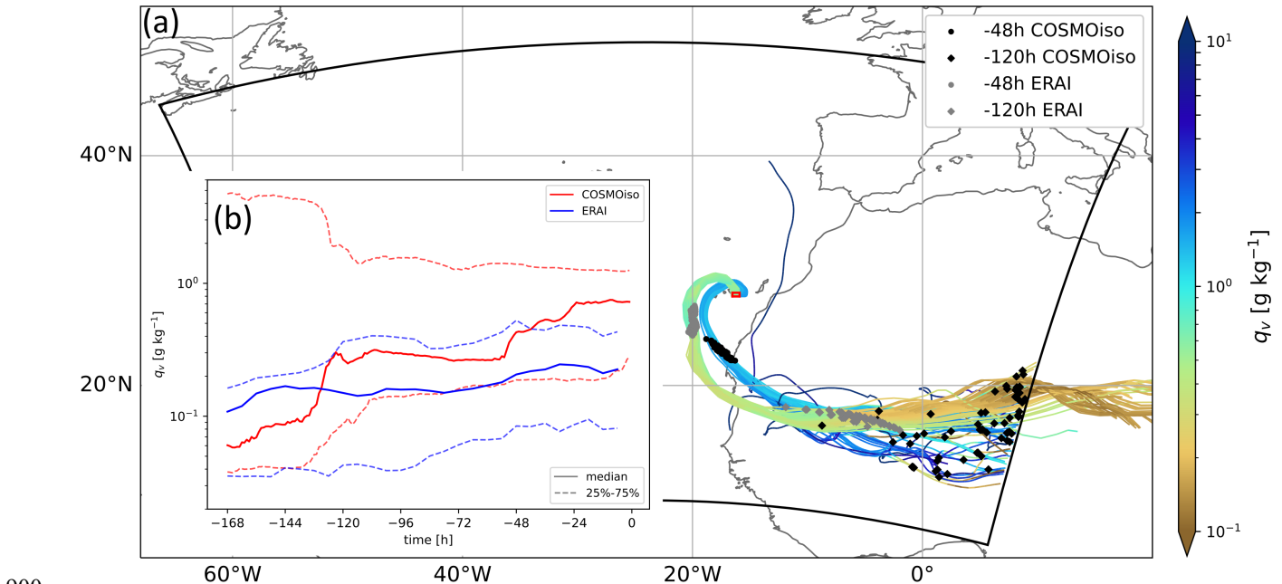
905 Figure A1: (a) COSMO iso and ERA-Interim backward trajectories started every hour between 10–13 UTC on 30 July 2013 (corresponding to observation period of airborne in situ measurements) from the 500 hPa level in the area of the MUSICA aircraft campaign (small red box). The trajectories are coloured according to their specific humidity q_v . The skewed black box depicts the COSMO iso model domain in rotated coordinates. Dots and diamonds show the COSMO iso (black) and ERA-Interim (grey) trajectory positions 2 and 5 days before arrival. (b) Temporal evolution of q_v along the COSMO iso and ERA-Interim backward trajectories displayed in (a). The red/blue solid lines represent the median of the 90 COSMO iso /ERA-Interim trajectories, the red/blue dashed lines the corresponding interquartile ranges.
