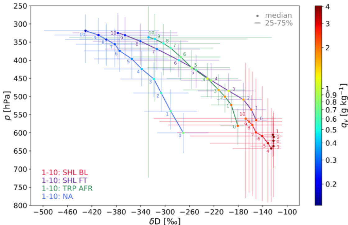
Figure 9: p - \delta D plot summarising the 10-day Lagrangian history of COSMO iso air parcels arriving at 500–700 hPa above Tenerife. The plot shows the median p and \delta D of the air parcels by the filled circles and the median q_v , by the colours of the filled circles. The numbers indicate the days before the air parcels arrive over Tenerife, where red numbers represent air parcels from the boundary layer of the Saharan heat low (SHL BL), purple numbers air parcels from the free troposphere above the Saharan heat low (SHL FT), green numbers air parcels from tropical Africa (TRP AFR) and blue numbers air parcels from the North Atlantic (NA). The interquartile range of p and \delta D is shown by the coloured vertical and horizontal lines.
