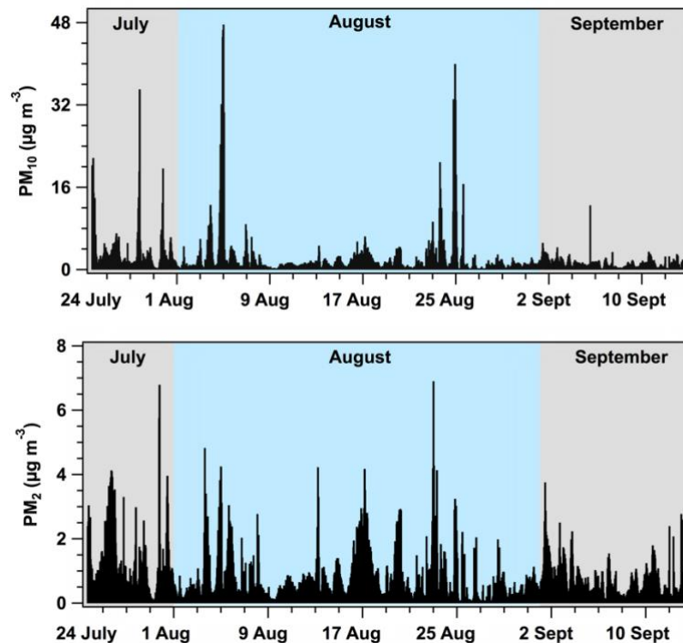
405 Figure 5. Mass concentration profiles for PM_2 and PM_{10} at Tuktoyaktuk during July-September 2018. The data are presented as 1-hour averages (Mountain Daylight Time), and each monthly period is demarcated by colour.
