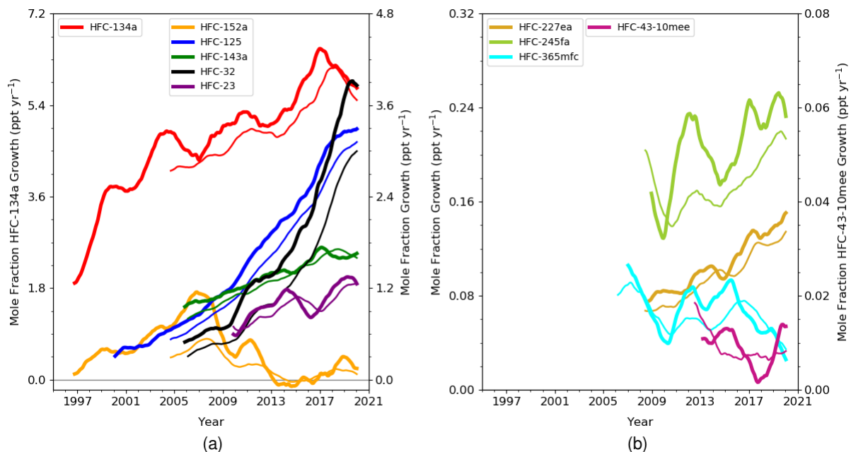
Figure 4. Northern Hemisphere atmospheric background mole fraction growth ( \text{ppt yr}^{-1} ) of HFCs at the Mace Head-MHD (Ireland) observing station are shown as thick lines, corresponding Southern Hemisphere values from Cape Grim-CGO (Australia) are shown as thin lines. A 2-year smoothing has been applied to the growths that are calculated by subtracting last year's mole fraction from this year's value on a monthly basis. The left y-axis for plot (a) relates to HFC-134a and the right axis relates to the other gases shown. The right y-axis for plot (b) relates to HFC-43-10mee and the left relates to the other gases shown. Note the change in y-scales.
