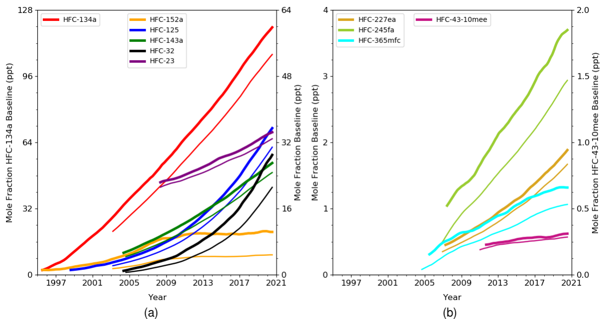
Figure 3. Northern Hemisphere atmospheric background mole fractions (ppt) of HFCs at the Mace Head-MHD (Ireland) observing station (thick lines) and Southern Hemisphere values at the Cape Grim-CGO (Australia) (thin lines). A 1-year smoothing has been applied to the monthly background estimates. The left y-axis for plot (a) relates to HFC-134a and the right axis relates to the other gases shown. The right y-axis for plot (b) relates to HFC-43-10mee and the left relates to the other gases shown. Note the change in y-scales.
