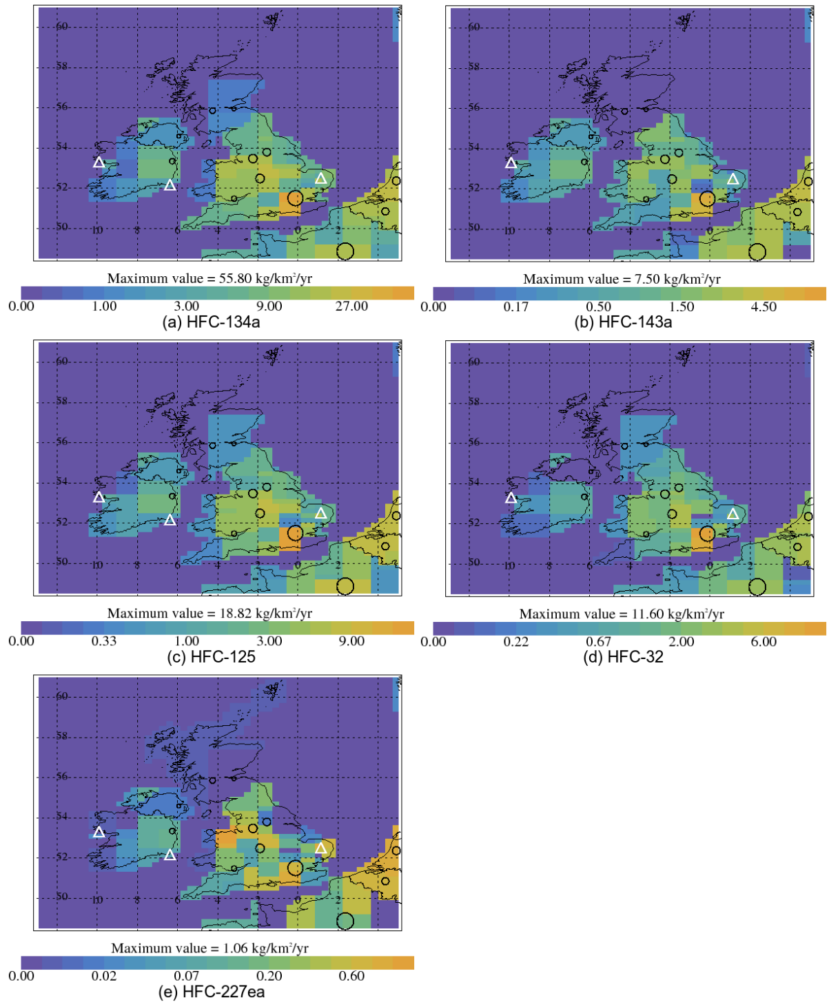
Figure 6. Two-year average InTEM emission estimate 2019–2020 ( \text{kg km}^{-2} \text{yr}^{-1} ) (a) HFC-134a (b) HFC-143a (c) HFC-125 (d) HFC-32 (e) HFC-227ea. Black circles represent major cities and white triangles show the location of the observation sites.
