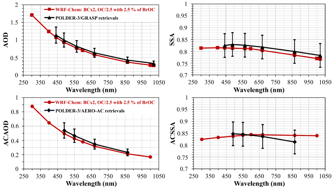
650 Figure 14: Spectral dependencies of AOD (left) and SSA (right) retrieved by POLDER-3/GRASP in clear-sky (top, black curves) and by POLDER-3/AERO-AC above clouds (bottom, black curves) and simulated with the WRF-Chem optimized configuration (BCx2, OC/2.5 with 2.5 % of BrOC, red curves). Black vertical error bars correspond to the uncertainties associated with the POLDER-3 data with an accuracy of \pm 15\% (per pixel estimate) on the aerosol optical depth and \pm 0.05 (per pixel estimate) on the single scattering albedo over the entire spectral domain. Values are averaged geographically on their respective study areas – (12°E-30°E, 10°S-0°S) over the Southern African continent in clear-sky and (0°E-15°E, 15°S-5°S) above clouds over the Southeastern Atlantic Ocean – and temporally over the first half of July 2008. 655
