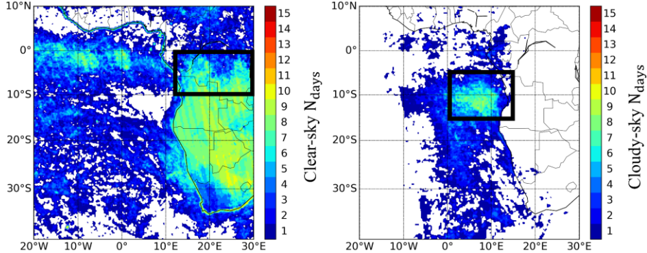
Figure 2: Number of observation days ( N_{\text{days}} ) in clear atmosphere (left) and cloudy atmosphere (right) available from the POLDER-3 space sensor during the 01-15 July 2008 period. The black frames indicate the two areas of study of the biomass burning aerosol optical properties in clear-sky over land (12°E-30°E, 10°S-0°S, left) and above clouds over the Southeastern Atlantic Ocean (0°E-15°E, 15°S-5°S, right).
