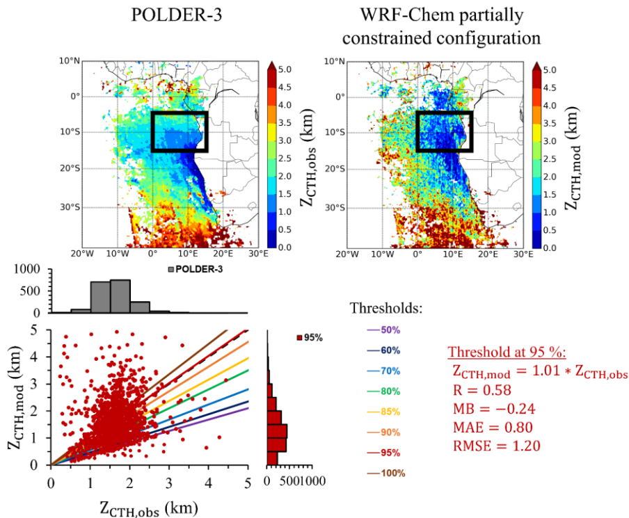
460 Figure 8: Monthly averaged cloud top heights retrieved by POLDER-3 (top, left) and simulated with the WRF-Chem partially constrained configuration with the threshold of 95 % (top, right) for July 2008, with an associated statistical analysis of the threshold values of the cloud top height tested in the model (bottom). The black frames (0°E-15°E, 15°S-5°S) represent the area of study.
