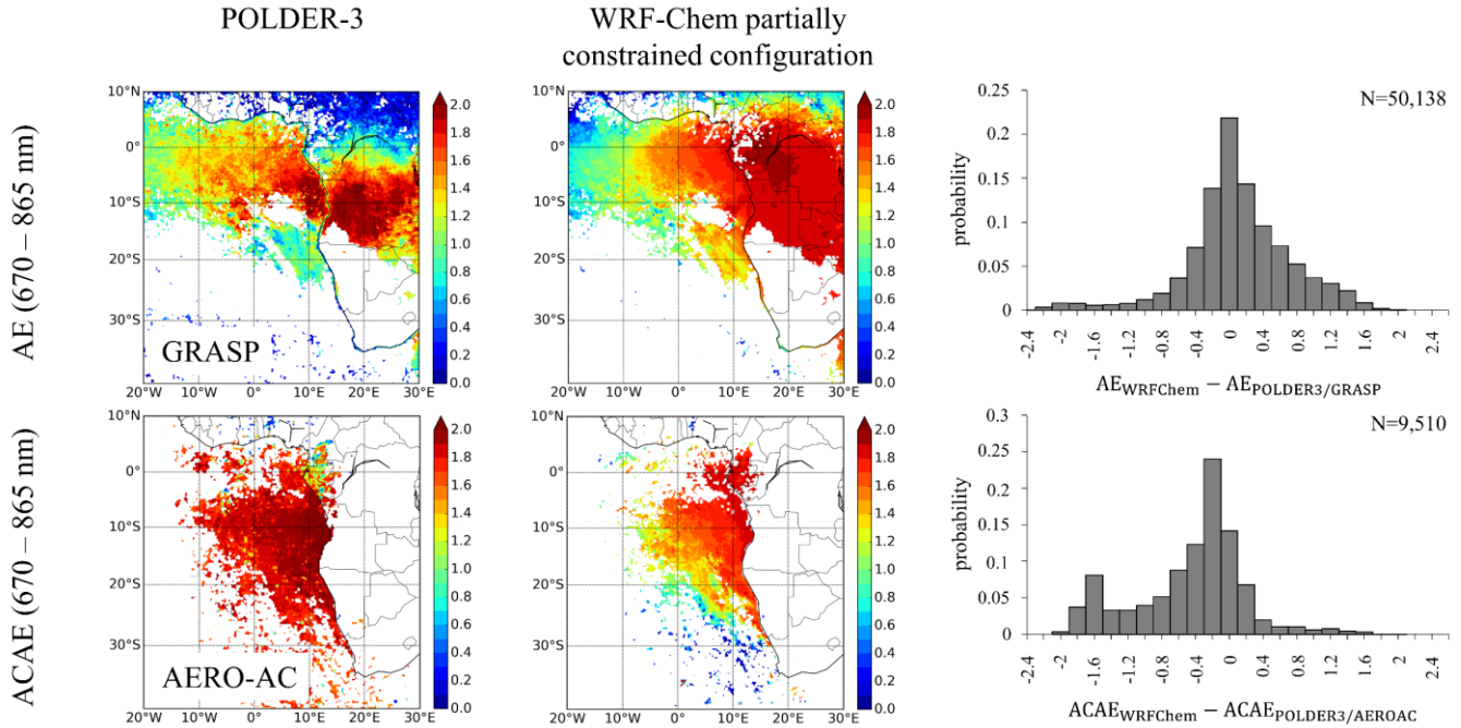
525 Figure 11: Monthly averaged Angström exponent retrieved by POLDER-3 in clear-sky with GRASP ( \text{AE}_{670-865} , top) and above clouds with AERO-AC ( \text{ACA}_{670-865} , bottom, left) and simulated with the WRF-Chem partially constrained configuration (middle) for July 2008, with the associated histograms of differences between the model and the satellite observations over the whole domain (right).
