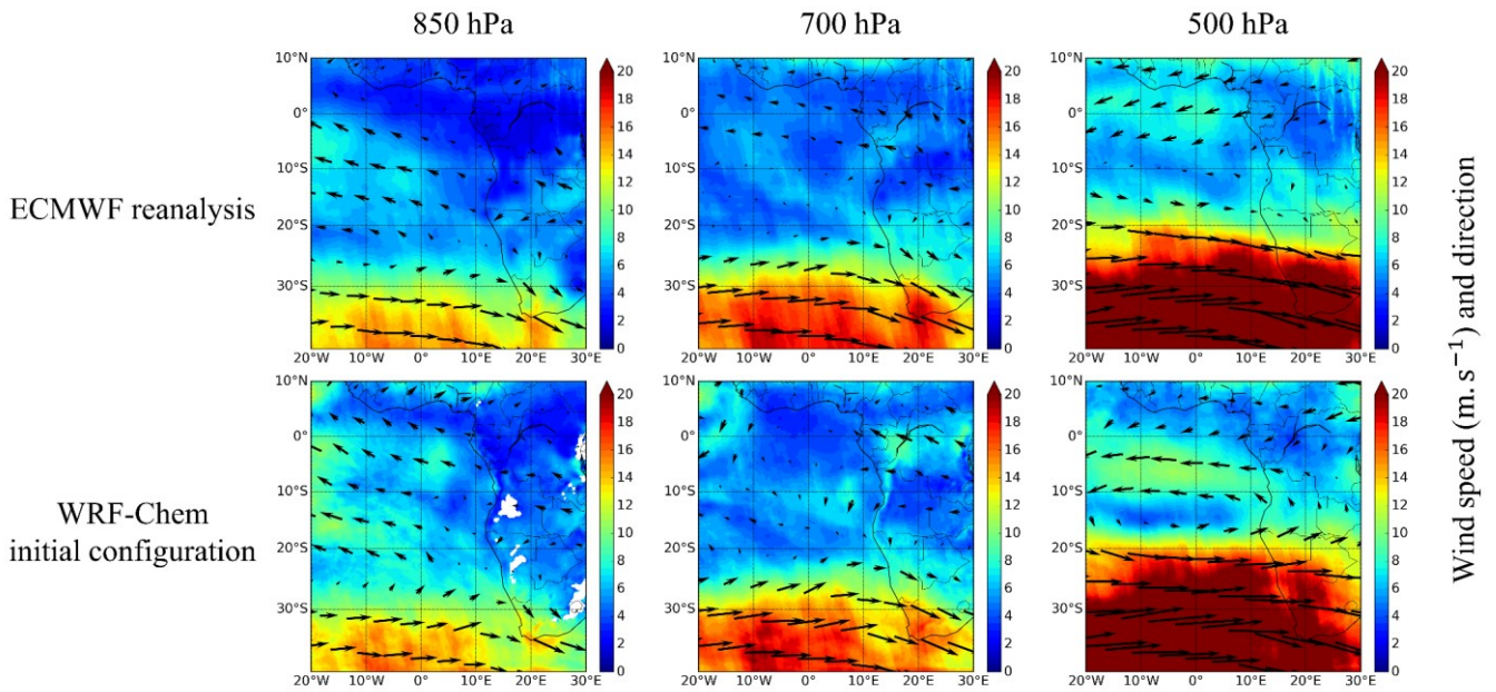
355 Figure 4: Monthly averaged wind speed (m. s -1 ) and direction at 850 hPa (left), 700 hPa (middle) and 500 hPa (right) from ECMWF ERA-Interim reanalysis (top) and simulated with the WRF-Chem initial configuration (bottom) for July 2008.
