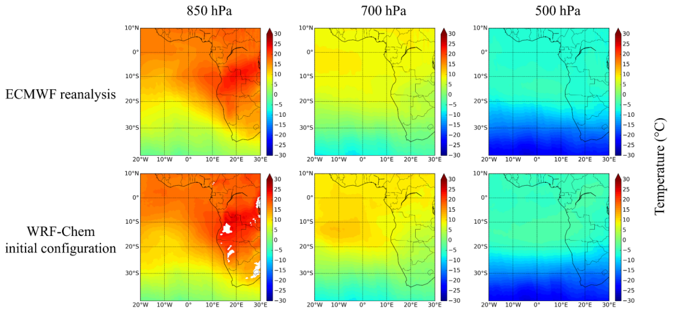
360 Figure 6: Same as Figure 4 but for temperature (in °C).
