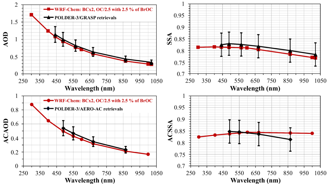
650 Figure 14: Spectral dependencies of AOD (left) and SSA (right) retrieved by POLDER-3/GRASP in clear-sky (top, black curves) and by POLDER-3/AERO-AC above clouds (bottom, black curves) and simulated with the WRF-Chem optimized configuration (BCx2, OC/2.5 with 2.5 % of BrOC, red curves). Black vertical error bars correspond to the uncertainties associated with the POLDER-3 data with an accuracy of \pm 15\% (per pixel estimate) on the aerosol optical depth and \pm 0.05 (per pixel estimate) on the single scattering albedo over the entire spectral domain. Values are averaged geographically on their respective study areas – (12°E-30°E, 10°S-0°S) over the Southern African continent in clear-sky and (0°E-15°E, 15°S-5°S) above clouds over the Southeastern Atlantic Ocean – and temporally over the first half of July 2008. 655
