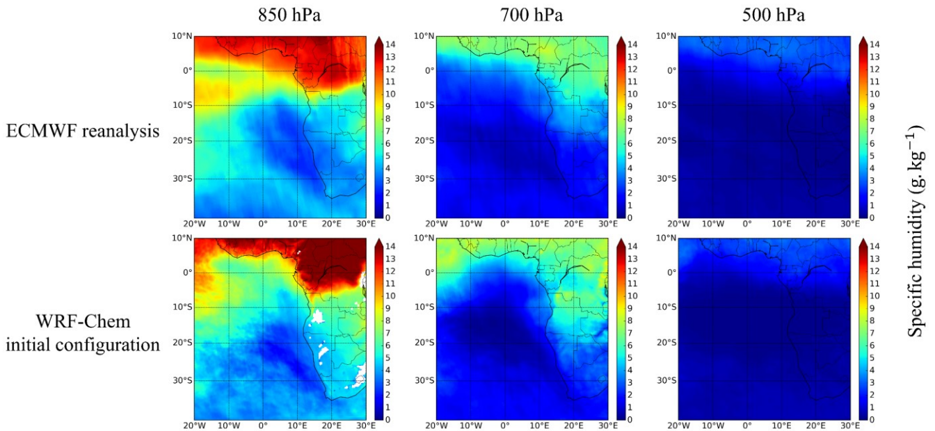
Figure 5: Same as Figure 4 but for specific humidity (in g. kg -1 ).
