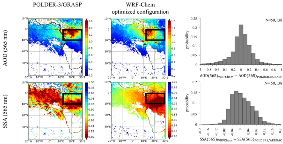
Figure 16: Comparison of monthly averaged AOD (top) and SSA (bottom) at 565 nm in clear-sky retrieved by POLDER-3/GRASP (left) and simulated with the WRF-Chem optimized configuration (right) over the Southeast Atlantic region for July 2008. The black frames of geographic coordinates, with the associated histograms of differences between the model and the satellite observations over the whole domain (right). The black frames (12°E-30°E, 10°S-0°S) represent the area of study.
