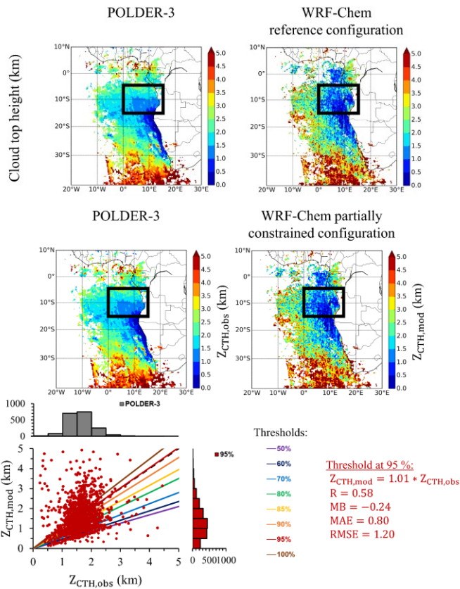
Figure 8: Monthly averaged cloud top heights retrieved by POLDER-3 (top, left) and simulated with the WRF-Chem reference configuration (top, right) for July 2008, with an associated statistical analysis of the threshold values of the cloud top height tested in the model (bottom). The black frames of geographic coordinates (0°E-15°E, 15°S-5°S) represent the area of study area.
