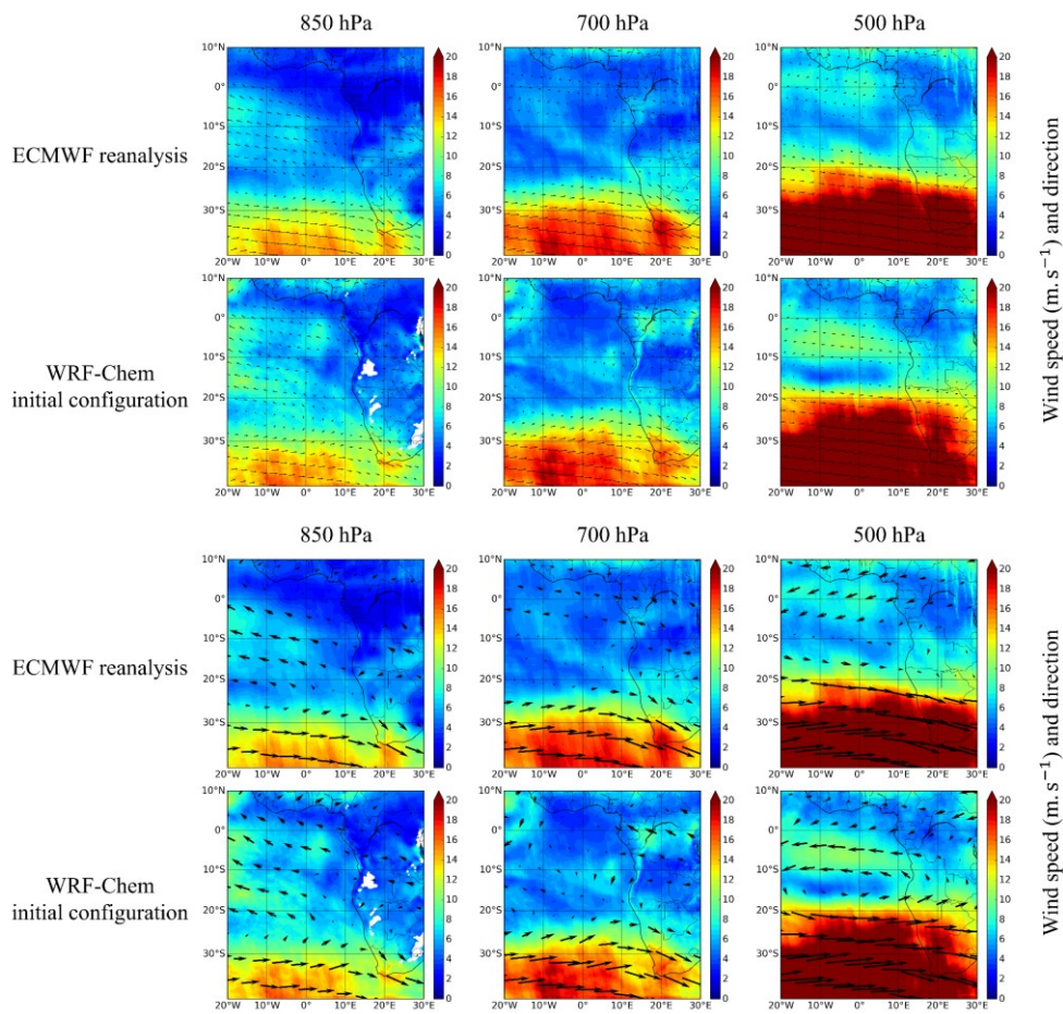
500 Figure 4: Monthly averaged wind speed ( \text{m} \cdot \text{s}^{-1} ) and direction at 850 hPa (left), 700 hPa (middle) and 500 hPa (right) from ECMWF ERA-Interim reanalysis (top) and simulated with the WRF-Chem initial configuration (bottom) for July 2008.
