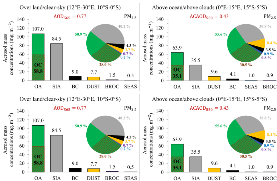
915 Figure 15: Evolution of the PM_{2.5} chemical composition simulated with the WRF-Chem optimized configuration between the Southern African continent in clear-sky (12°E-30°E, 10°S-0°S, left) and the Southeastern Atlantic Ocean above clouds (0°E-15°E, 15°S-5°S, right). Mass concentrations (in mg \cdot m^{-2} ) of the main aerosol compounds of biomass burning, i.e., black carbon (BC, in black), organic carbon (OC, in brown hatching), brown carbon (BrOC, in purple), organic aerosols (OA, in green) and secondary inorganic aerosols (SIA, in grey), as well as desert dust aerosols (DUST, in yellow) and sea salt aerosols (SEAS, in blue), are vertically integrated over the atmospheric column on average for the first half of July 2008.
