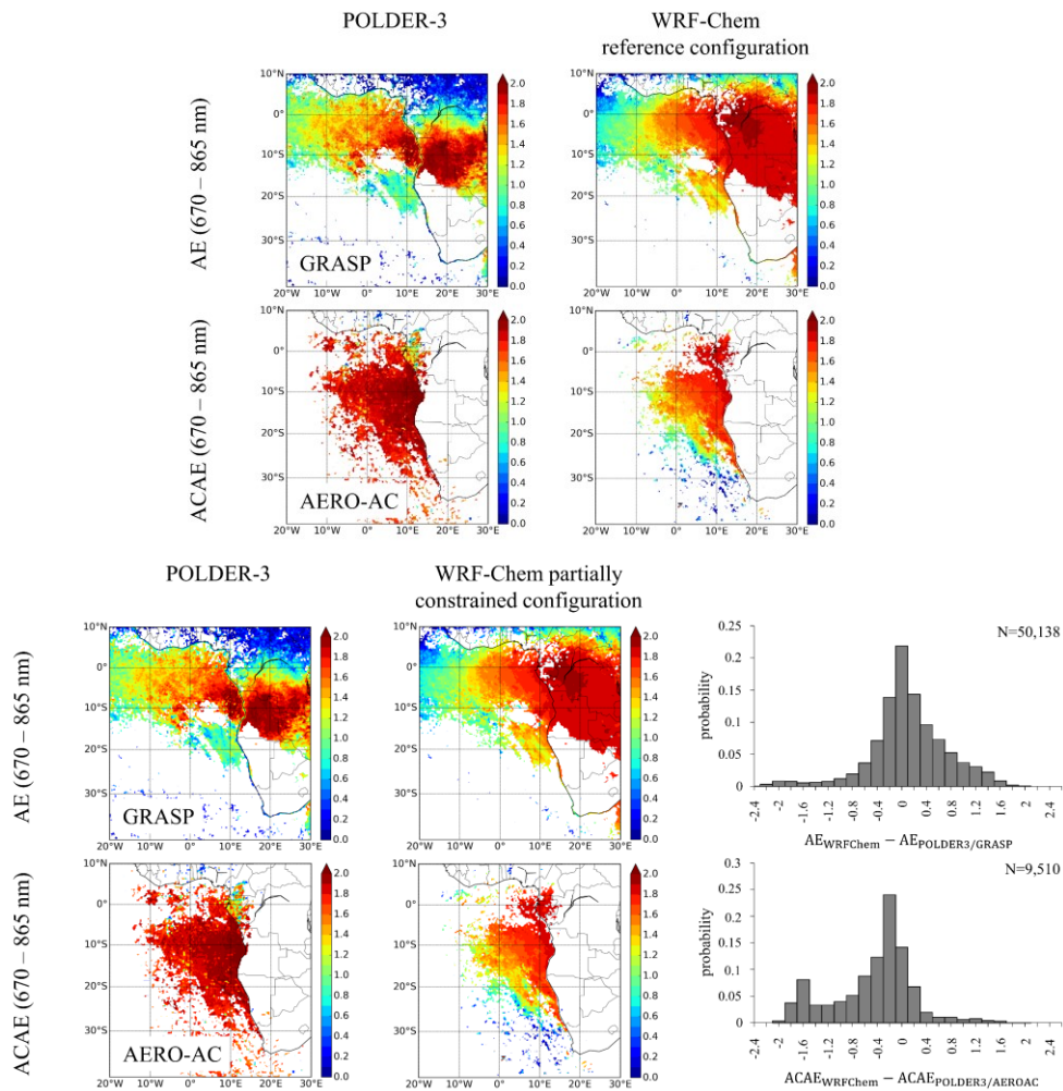
735 Figure 11: Monthly averaged Angström exponent retrieved by POLDER-3 in clear-sky with GRASP ( AE_{670-865} , top) and above clouds with AERO-AC ( ACAE_{670-865} , bottom) (left) and simulated with the WRF-Chem reference configuration (right middle) for July 2008, with the associated histograms of differences between the model and the satellite observations over the whole domain (right).
