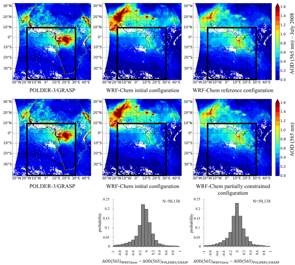
Figure 7: Monthly averaged aerosol optical depth (AOD) at 565 nm in clear-sky retrieved by POLDER-3/GRASP (top, left) and simulated with the WRF-Chem initial configuration (top, middle) and with the WRF-Chem reference configuration (top, right) for July 2008, with the associated histograms of differences between the model and the satellite observations over the whole domain (bottom). The black frames of geographic coordinates (20°W-30°E, 39.9°S-10°N) represent the domain area of study.
