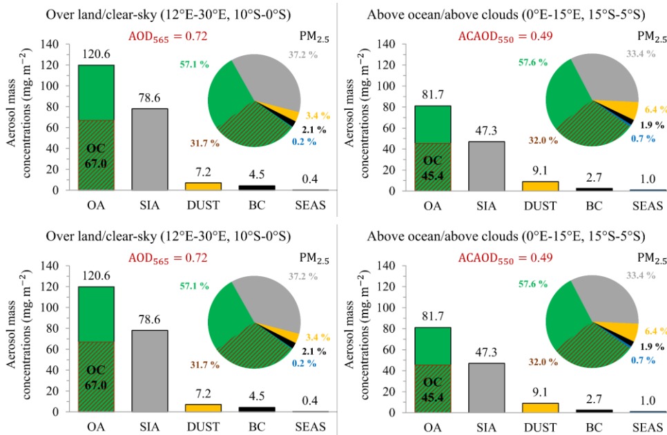
760 Figure 12: Evolution of the PM 2.5 chemical composition simulated with the WRF-Chem referencepartially constrained configuration between the Southern African continent in clear-sky (12°E-30°E, 10°S-0°S, left) and the Southeastern Atlantic Ocean above clouds (0°E-15°E, 15°S-5°S, right). Mass concentrations (in mg·m -2 ) of the main aerosol compounds of biomass burning, i.e. black carbon (BC, black), organic carbon (OC, brown hatching), organic aerosols (OA, green) and secondary inorganic aerosols (SIA, grey), as well as desert dust aerosols (DUST, yellow) and sea salt aerosols (SEAS, blue), are vertically integrated over the 765 atmospheric column on average for July 2008.
