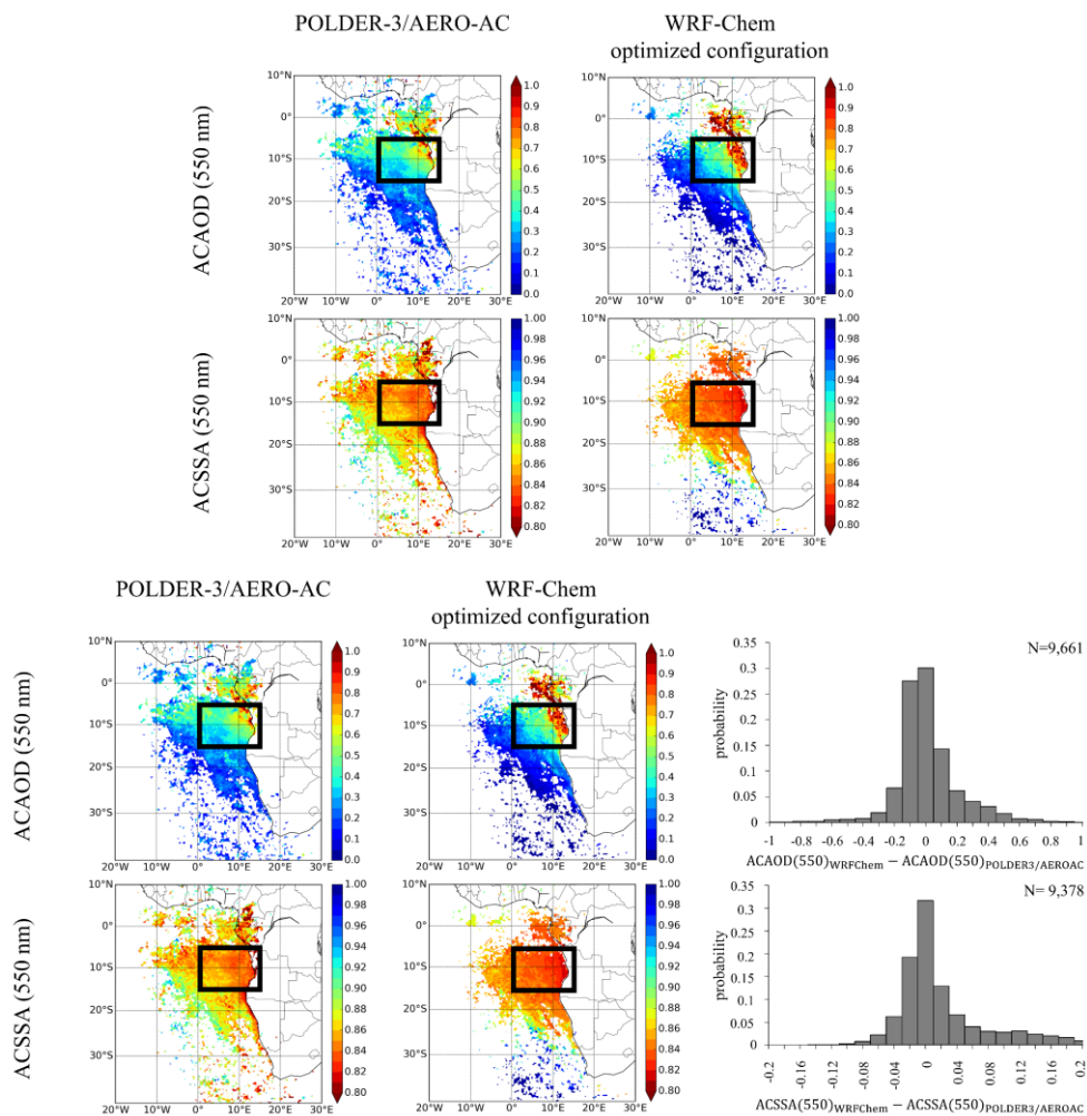
Figure 17: Comparison of monthly averaged ACAOD (top) and ACSSA (bottom) at 550 nm above clouds retrieved by POLDER-3/AERO-AC (left) and simulated with the WRF-Chem optimized configuration (right) over the Southeast Atlantic region for July 2008. The black frames of geographic coordinates, with the associated histograms of differences between the model and the satellite observations over the whole domain (right). The black frames (0°E-15°E, 15°S-5°S) represent the area of study.
