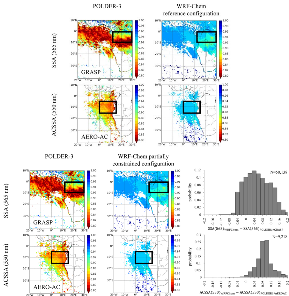
Figure 13: Monthly averaged single scattering albedo of aerosols at 565 nm in clear-sky (SSA, top) and at 550 nm above clouds (ACSSA, bottom) retrieved by POLDER-3 (left) and simulated with the WRF-Chem reference configuration (top right) and the WRF-Chem partially constrained configuration (bottom right) for July 2008, with the associated histograms of differences between the model and the satellite observations over the whole domain (right). The black frames of geographic coordinates (12°E-30°E, 10°S-0°S) and (0°E-15°E, 15°S-5°S) represent respectively the two study regions, in clear-sky (top) and above clouds (bottom).
