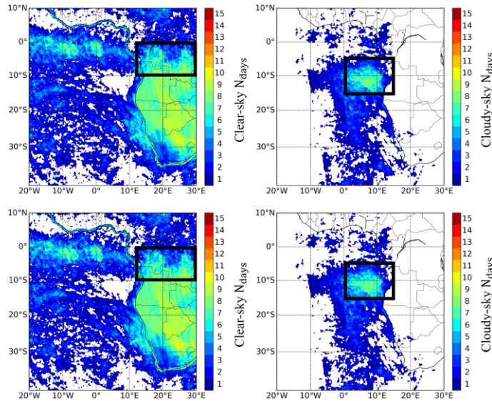
Figure 2: Number of observation days ( N_{\text{days}} ) in clear atmosphere (left) and cloudy atmosphere (right) available from the POLDER-3 space sensor during the 01-15 July 2008 period. The black frames indicate the two areas of study of the biomass burning aerosol optical properties in clear-sky over land (12°E-30°E, 10°S-0°S, left) and above clouds over the Southeastern Atlantic Ocean (0°E-15°E, 15°S-5°S, right).
