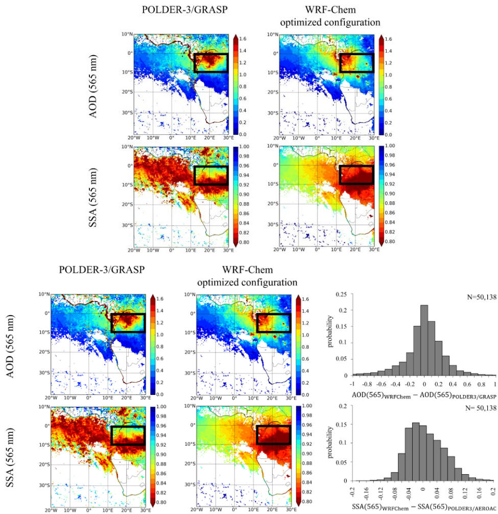
Figure 16: Comparison of monthly averaged AOD (top) and SSA (bottom) at 565 nm in clear-sky retrieved by POLDER-3/GRASP (left) and simulated with the WRF-Chem optimized configuration (right) over the Southeast Atlantic region for July 2008. The black frames of geographic coordinates, with the associated histograms of differences between the model and the satellite observations over the whole domain (right). The black frames (12°E-30°E, 10°S-0°S) represent the area of study.
