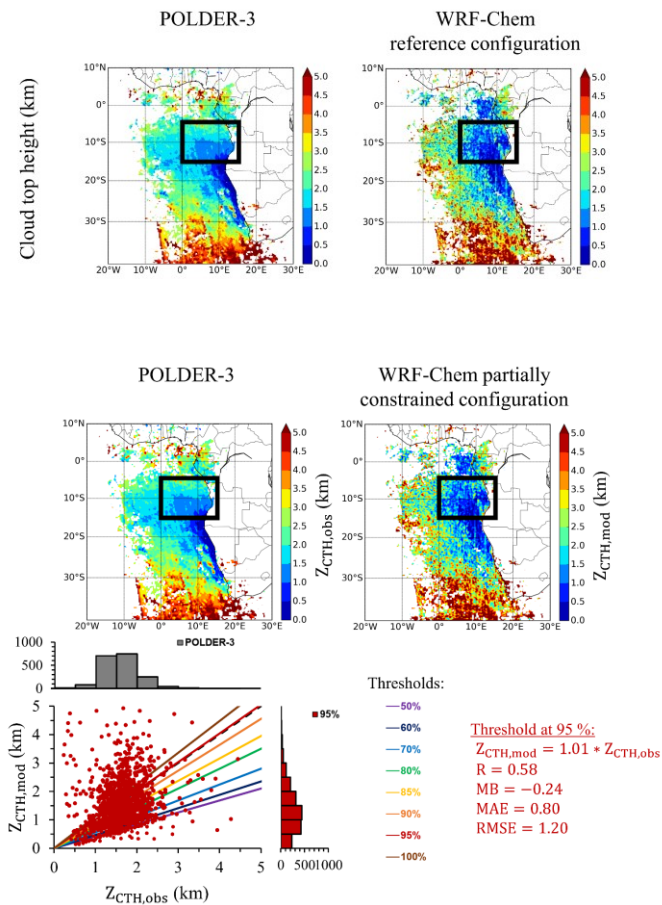
635 Figure 8: Monthly averaged cloud top heights retrieved by POLDER-3 (top_left) and simulated with the WRF-Chem referencepartially constrained configuration with the threshold of 95 % (top_right) for July 2008, with an associated statistical analysis of the threshold values of the cloud top height tested in the model (bottom). The black frames of geographic coordinates (0°E-15°E, 15°S-5°S) represent the area of study-area.
