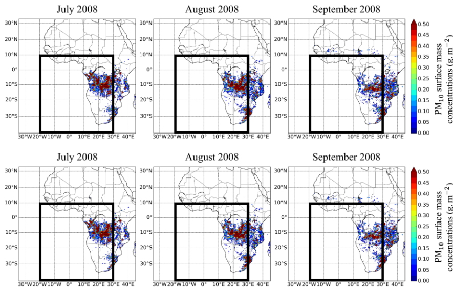
Figure 1: Monthly mass concentrations of PM_{10} (in g \cdot m^{-2} ) emitted at the surface by African biomass burning in July (left), August (middle) and September (right) 2008 from the APIFLAMEv1 biomass burning emission inventory (Turquety et al. 2014). The black frames of geographic coordinates ( 20^{\circ}W-30^{\circ}E, 39.4^{\circ}S-10^{\circ}N ) represent the domain (Turquety et al., 2014). The black frames ( 20^{\circ}W-30^{\circ}E, 39.4^{\circ}S-10^{\circ}N ) represent the area of study.
