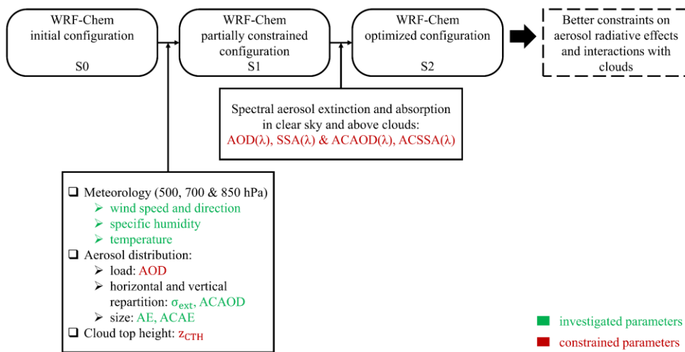
Figure 3: Schematic diagram of the general approach applied to constrain WRF-Chem simulations of aerosols using A-Train satellite coincident retrievals of the distributions of aerosols and clouds. AOD , ACAOD , SSA , ACSSA , \sigma_{ext} , AE , ACAE and z_{CTH} stand for aerosol optical depth, above-cloud aerosol optical depth, single scattering albedo, above-cloud single scattering albedo, aerosol extinction coefficient, Angstrom exponent, above-cloud Angstrom exponent and cloud top height, respectively.
