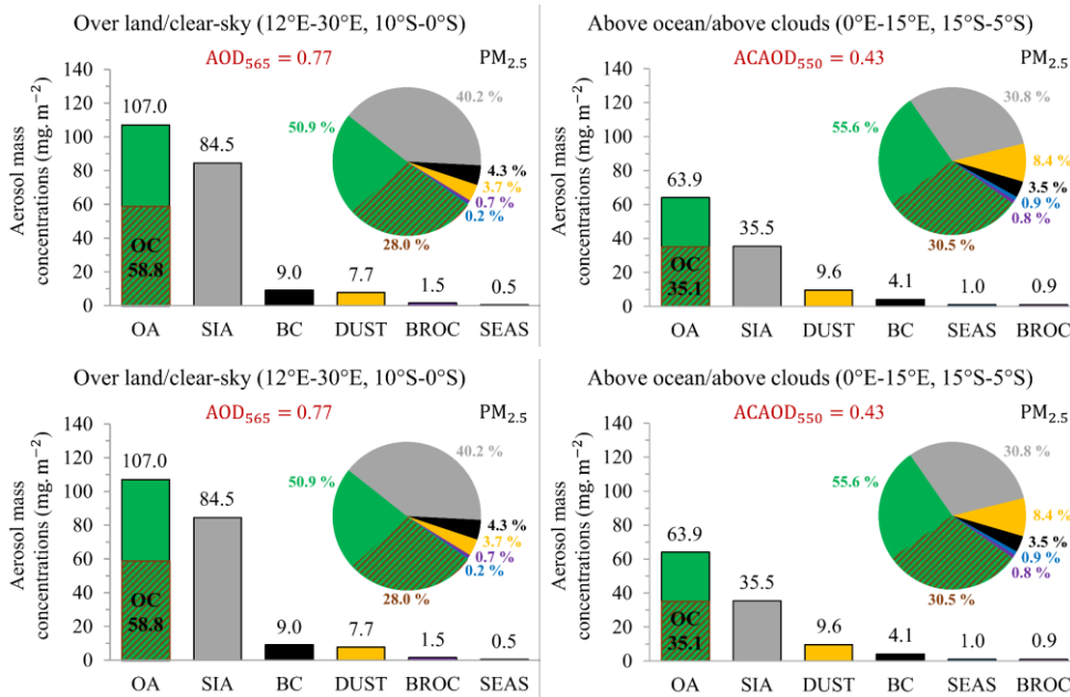
Figure 15: Evolution of the PM_{2.5} chemical composition simulated with the WRF-Chem optimized configuration between the Southern African continent in clear-sky (12°E-30°E, 10°S-0°S, left) and the Southeastern Atlantic Ocean above clouds (0°E-15°E, 15°S-5°S, right). Mass concentrations (in mg \cdot m^{-2} ) of the main aerosol compounds of biomass burning, i.e., black carbon (BC, in black), organic carbon (OC, in brown hatching), brown carbon (BrOC, in purple), organic aerosols (OA, in green) and secondary inorganic aerosols (SIA, in grey), as well as desert dust aerosols (DUST, in yellow) and sea salt aerosols (SEAS, in blue), are vertically integrated over the atmospheric column on average for the first half of July 2008.
