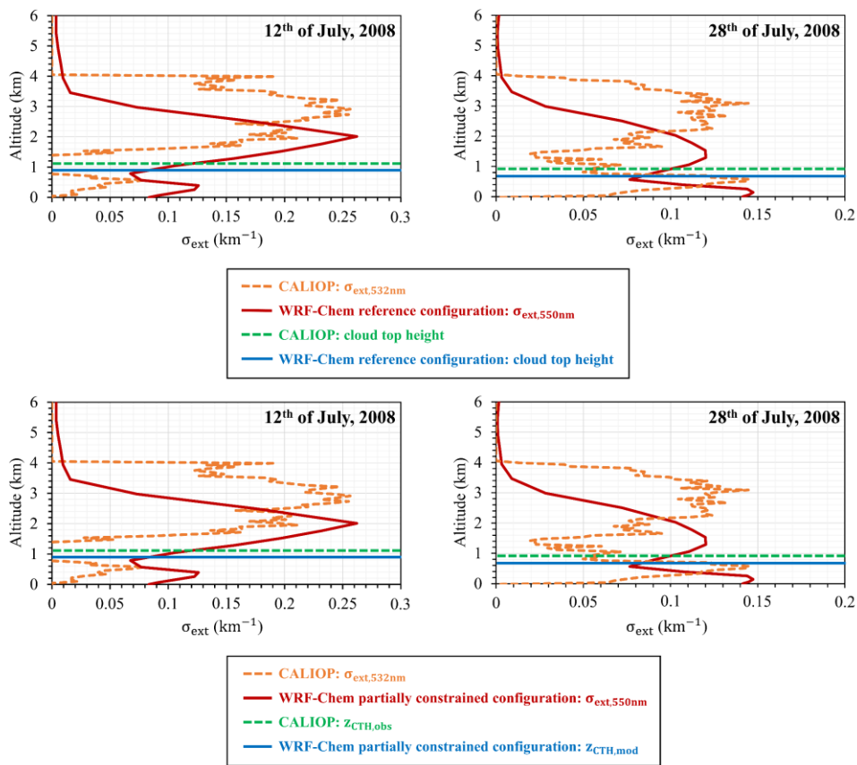
Figure 9: Mean vertical profiles of the aerosol extinction coefficients retrieved by CALIOP at 532 nm (orange dotted lines) and simulated with the WRF-Chem referencepartially constrained configuration at 550 nm (red solid lines) under the CALIOP track inside the study area of geographic coordinates (0°E-15°E, 15°S-5°S) for July 12, 2008 (left) and July 28, 2008 (right). Mean cloud top heights retrieved by CALIOP (green dotted lines) and simulated with the WRF-Chem referencepartially constrained configuration (blue solid lines) are also incorporated into the graphics. CALIOP data, initially at a horizontal spatial resolution of 5x5 km 2 , were aggregated onto the WRF-Chem mesh (30x30 km 2 ) and only the coincident pixels were selected for the comparison study.
