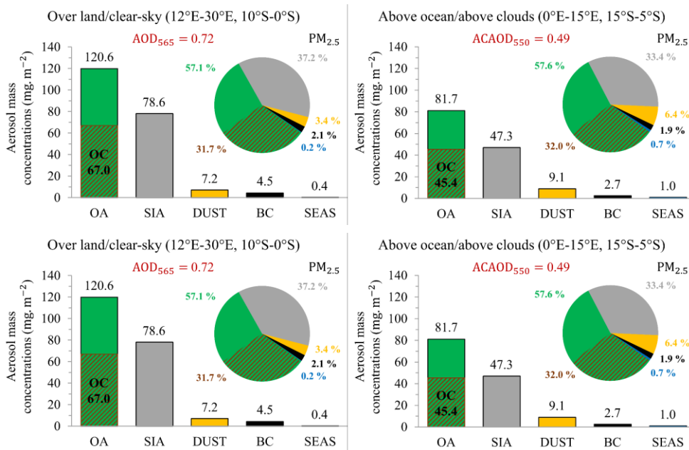
Figure 12: Evolution of the PM 2.5 chemical composition simulated with the WRF-Chem referencepartially constrained configuration between the Southern African continent in clear-sky (12°E-30°E, 10°S-0°S, left) and the Southeastern Atlantic Ocean above clouds (0°E-15°E, 15°S-5°S, right). Mass concentrations (in mg·m -2 ) of the main aerosol compounds of biomass burning, i.e. black carbon (BC, black), organic carbon (OC, brown hatching), organic aerosols (OA, green) and secondary inorganic aerosols (SIA, grey), as well as desert dust aerosols (DUST, yellow) and sea salt aerosols (SEAS, blue), are vertically integrated over the atmospheric column on average for July 2008.
