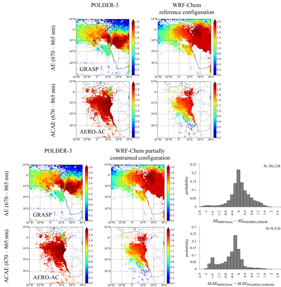
Figure 11: Monthly averaged Angström exponent retrieved by POLDER-3 in clear-sky with GRASP ( AE_{670-865} , top) and above clouds with AERO-AC ( ACAЕ_{670-865} , bottom) (left) and simulated with the WRF-Chem reference partially constrained configuration (right middle) for July 2008, with the associated histograms of differences between the model and the satellite observations over the whole domain (right).
