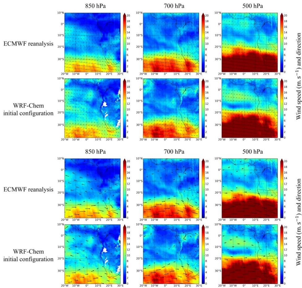
Figure 4: Monthly averaged wind speed ( \text{m} \cdot \text{s}^{-1} ) and direction at 850 hPa (left), 700 hPa (middle) and 500 hPa (right) from ECMWF ERA-Interim reanalysis (top) and simulated with the WRF-Chem initial configuration (bottom) for July 2008.
