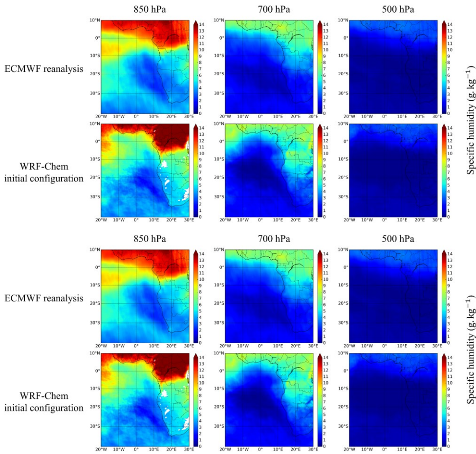
Figure 5: Same as Figure 4 but for specific humidity (in \text{g kg}^{-1} ).
