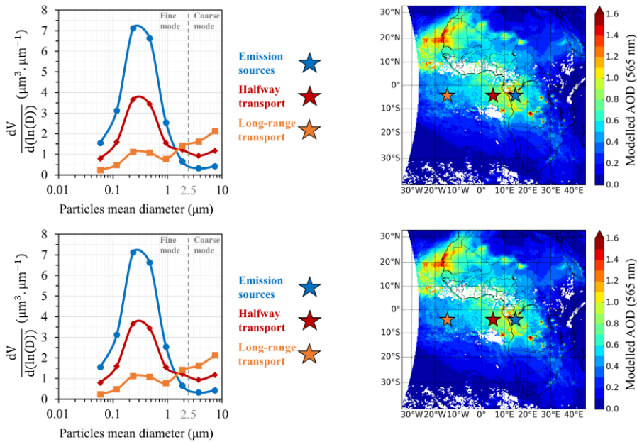
705 Figure 10: Evolution of the vertically integrated (whole atmospheric column) volume size distribution of aerosols simulated with the WRF-Chem referencepartially constrained configuration for three areas representative of the emission sources and transport progress of the biomass burning aerosol plume on average for July 2008. The blue star corresponds to the pixel of geographic coordinates (14.83°E, 4.00°S) and symbolizes the emission sources of biomass burning particles. The red star corresponds to the pixel of geographic coordinates (4.82°E, 4.00°S) and symbolizes the biomass burning aerosol plume transported halfway westward over the Southeastern Atlantic Ocean. The orange star corresponds to the pixel of geographic coordinates (14.93°W, 4.00°S) and symbolizes the long-range transport of the biomass burning aerosol plume. 710
