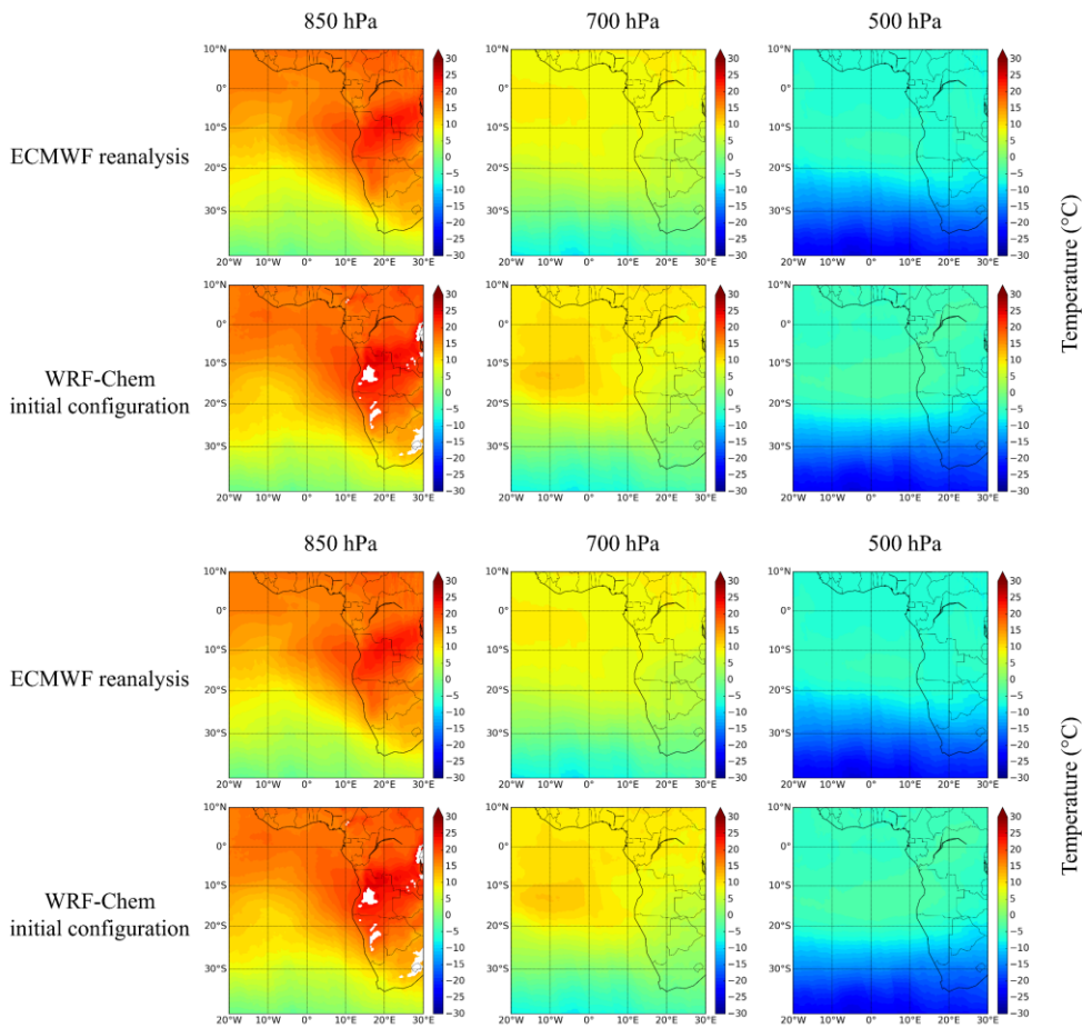
Figure 6: Same as Figure 4 but for temperature (in °C).
