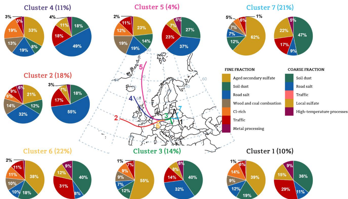
540 Figure 7: Trajectory cluster centroids arriving to Warsaw at 200 m (center map) with PMF factor contribution in different clusters for the fine (left pie charts) and coarse (right pie charts) fraction. The percentage of the trajectories classified into each cluster is given in parentheses.
