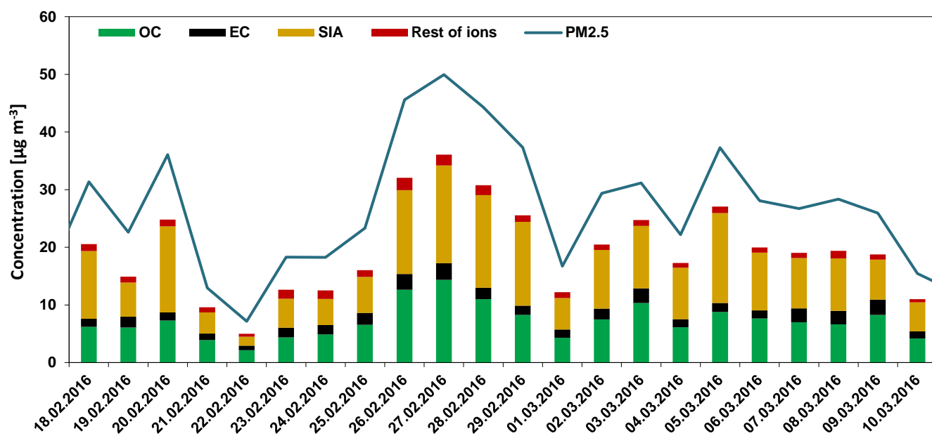
245 Figure 2: Time series of daily concentrations ( \mu g m^{-3} ) of PM_{2.5} (line) and its main components (bars) in Warsaw in the sampling period from 18 February to 10 March, 2016. Rest of ions indicate the sum of concentrations of K^+ , Cl^- , Na^+ , Mg^{2+} and Ca^{2+} ions.
