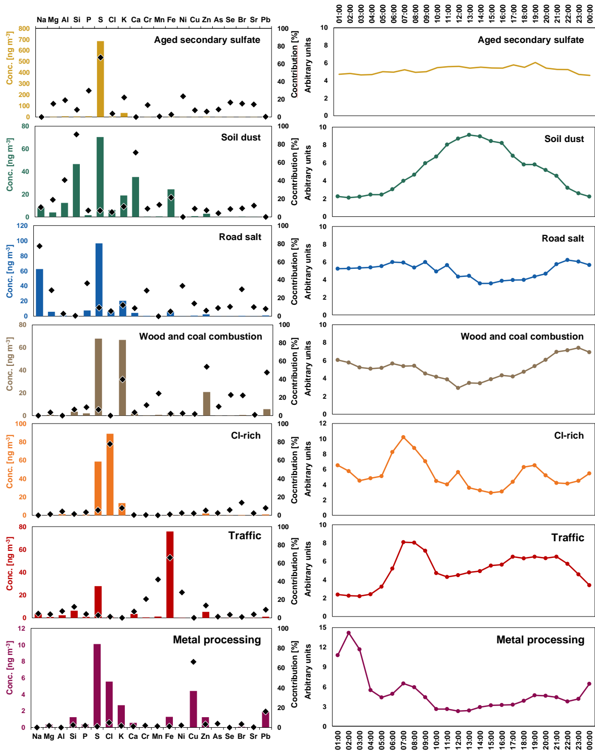
350 Figure 4: Left panel: PMF profiles (bars, left y axis) and contributions (black diamonds, right y axis) of the identified sources for the fine fraction. Right panel: Daily patterns of the identified sources (in arbitrary units).
