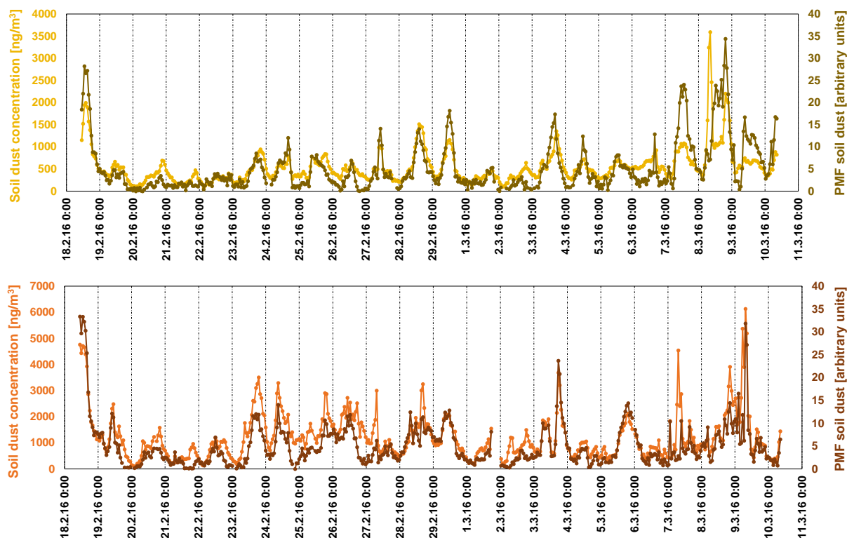
665 Figure 9: Hourly time series of the “Soil dust” source contributions identified by PMF analysis (dark colors) and calculated soil component concentrations (light colors) in the fine (upper panel) and coarse (bottom panel) fractions.
