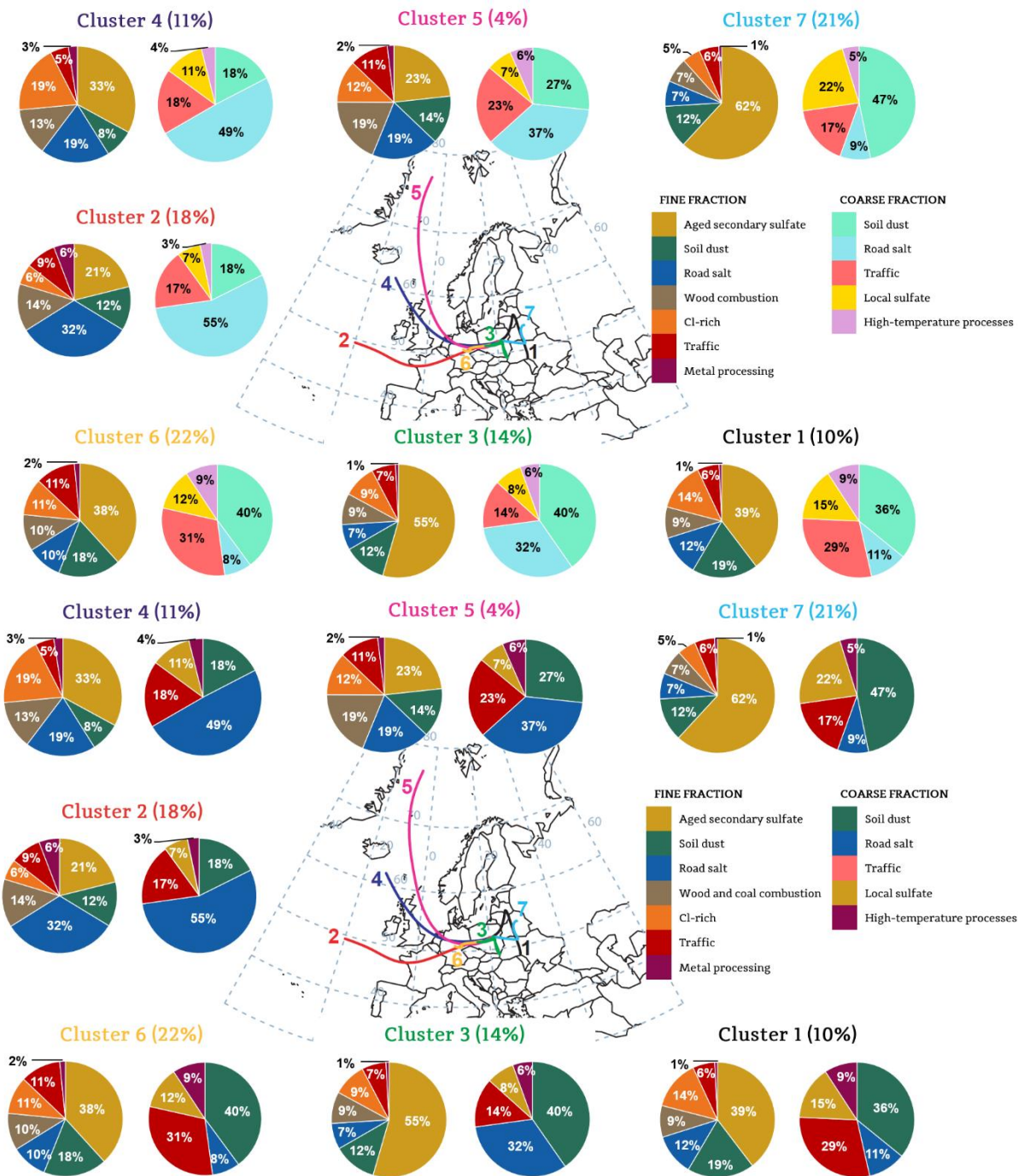
Figure 7: Trajectory cluster centroids arriving to Warsaw at 200 m (center map) with PMF factor contribution in different clusters for fine (left pie charts) and coarse (right pie charts) fraction. Percentage of the trajectories classified into each cluster is given in the parentheses.
