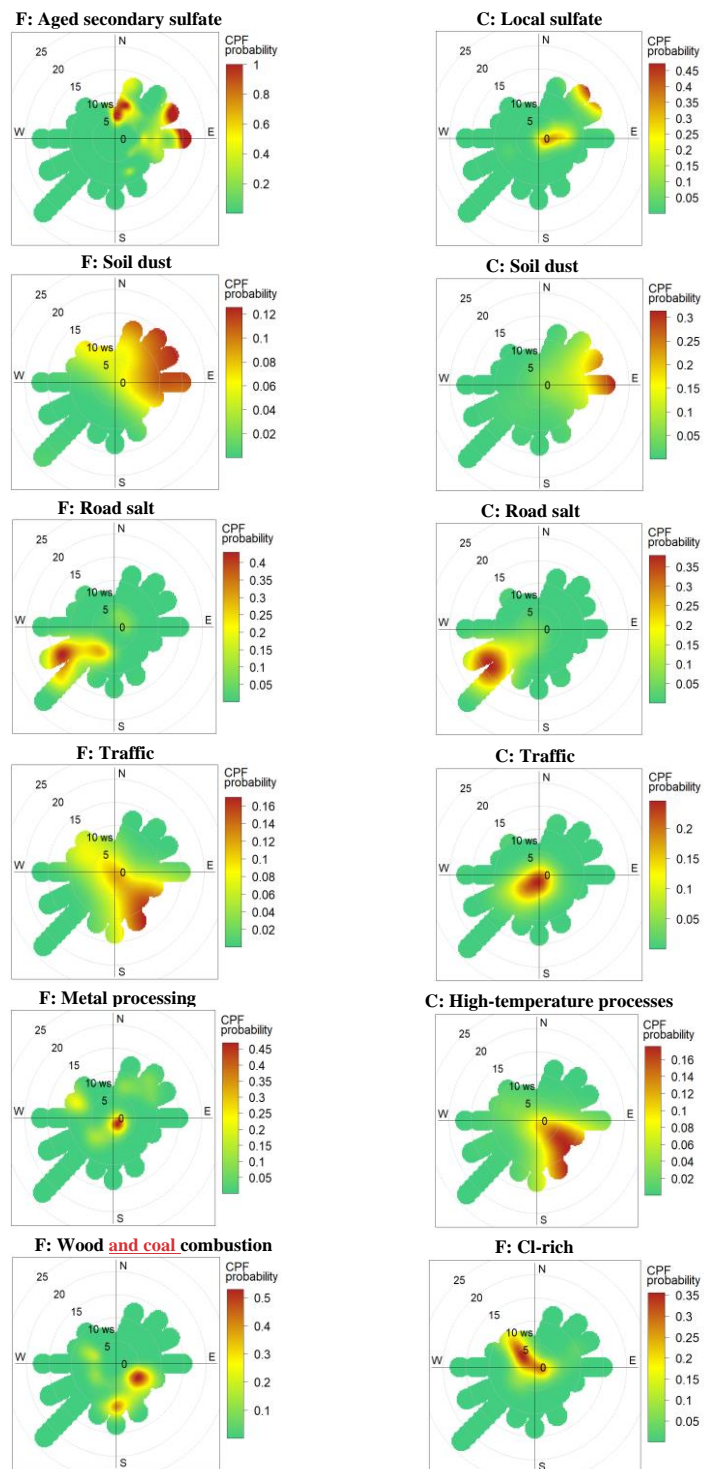
395 Figure 6: Conditional Probability Function (CPF) analysis (at 90th percentile) of the PMF sources identified in the fine (F) and coarse (C) fractions. Wind speed (ws) is expressed in \text{km h}^{-1} .
