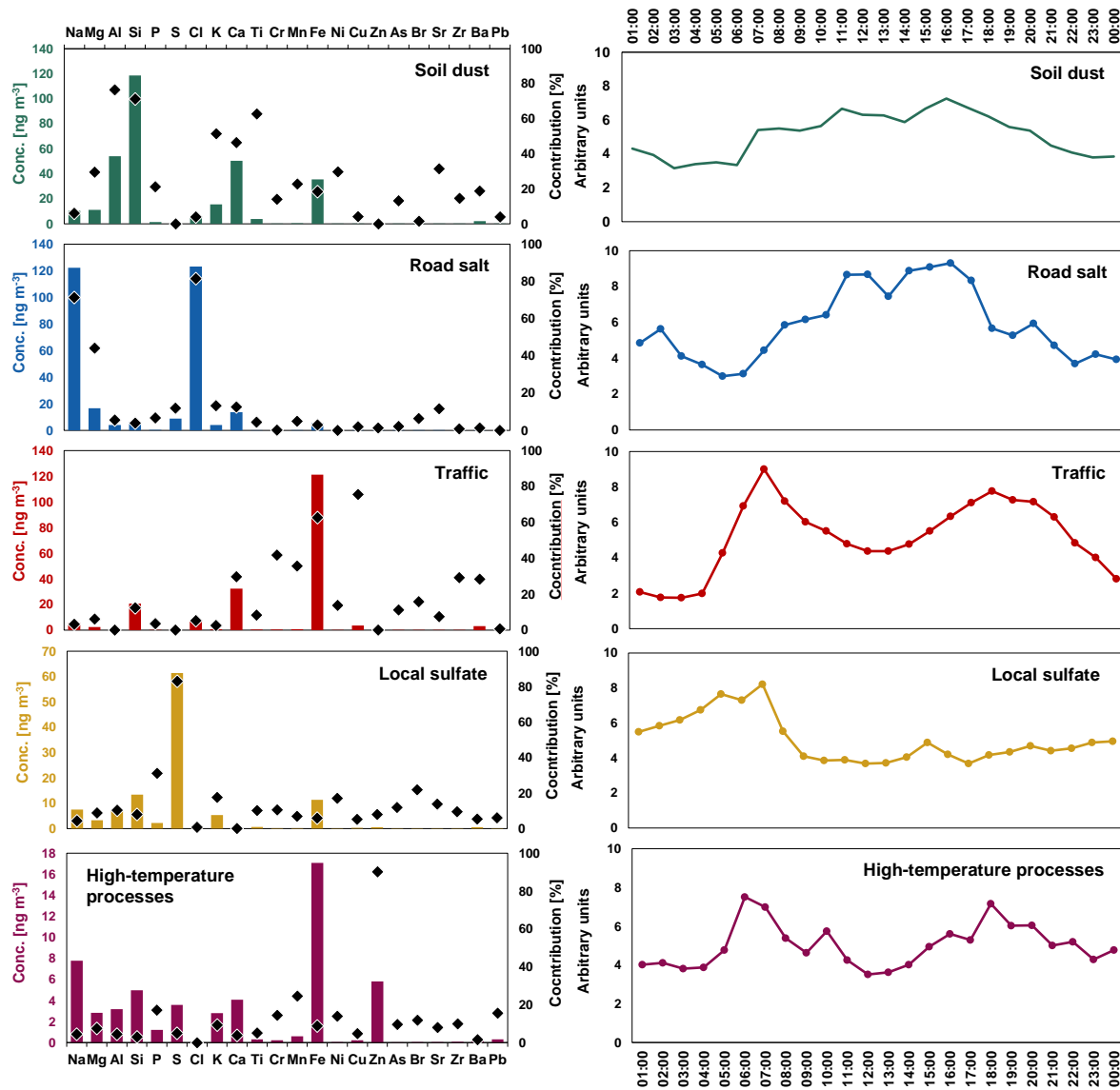
Figure 5: Left panel: PMF profiles (bars, left y axis) and explained variations contributions (black diamonds, right y axis) of the identified sources for the coarse fraction. Right panel: Daily patterns of the identified sources (in arbitrary units).
