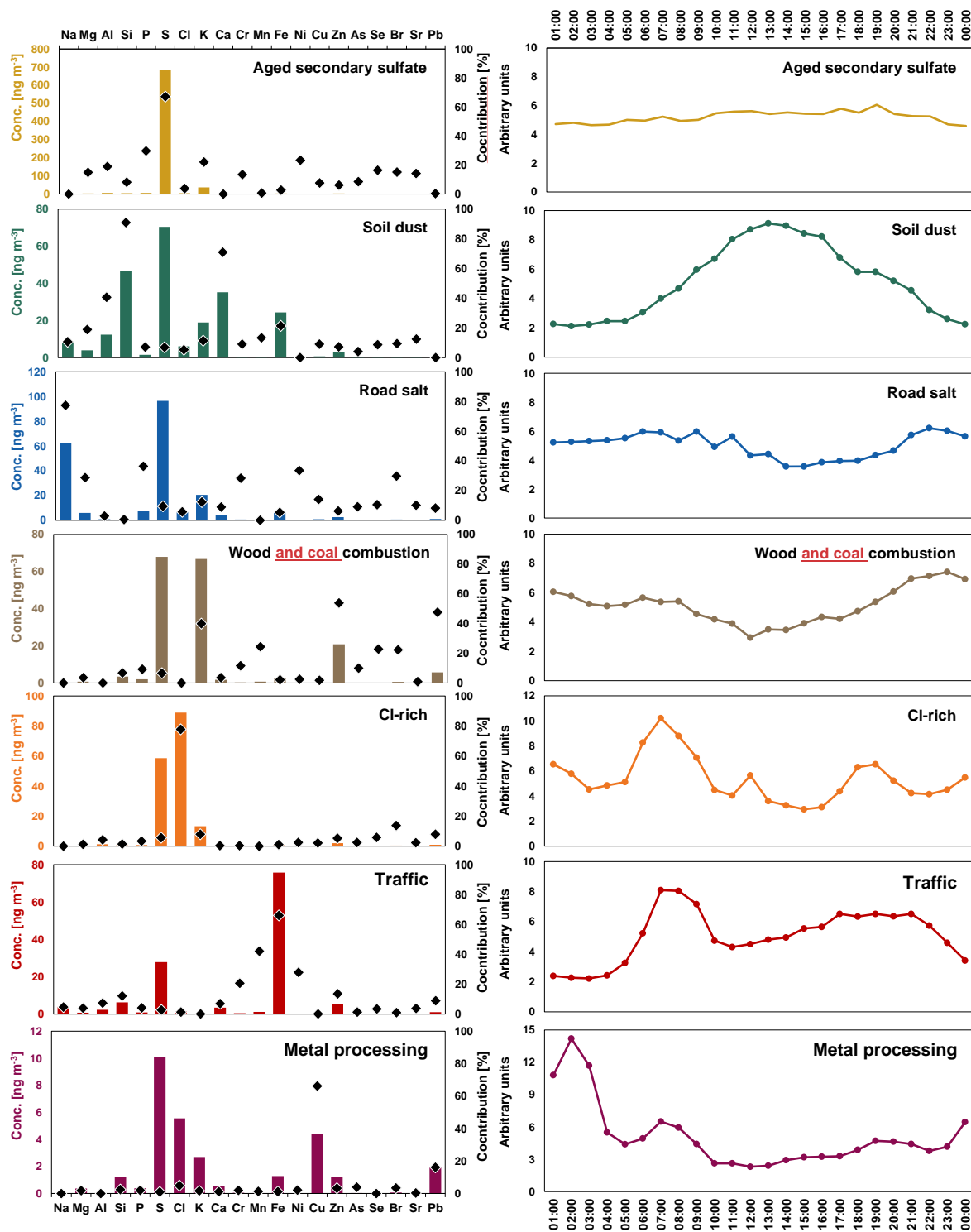
Figure 4: Left panel: PMF profiles (bars, left y axis) and explained variations contributions (black diamonds, right y axis) of the identified sources for the fine fraction. Right panel: Daily patterns of the identified sources (in arbitrary units).
