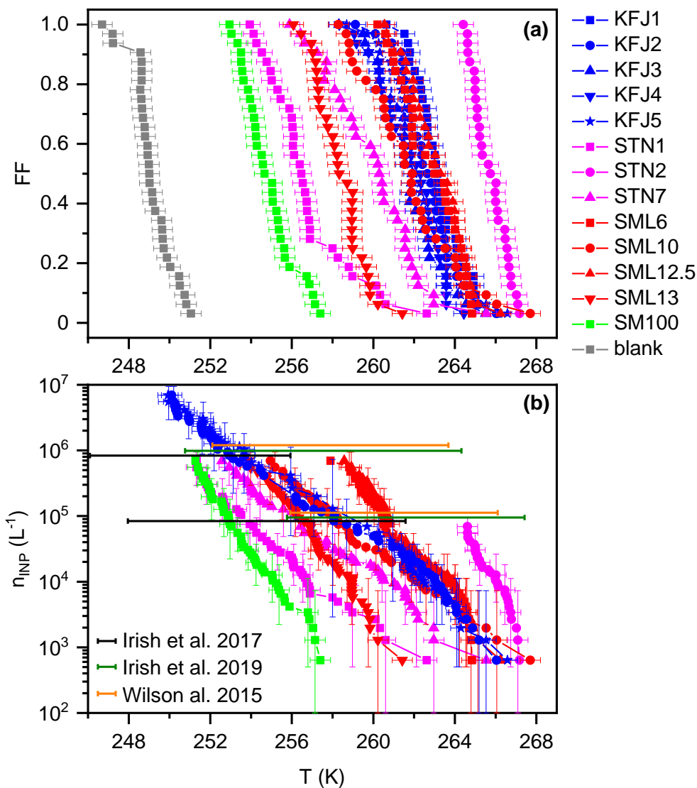
1325 Figure 2: (a) Frozen fraction, FF , curves of the investigated samples from cold-stage measurements with INSEKT, corrected for the freezing point depression by the salts. (b) Cumulative INP concentrations, n_{\text{INP}} ( \text{L}^{-1} ), as computed with Eq. (1) from the measurements in panel (a) and additional INSEKT measurements where the solutions were diluted by a factor of 10 and 100 with ultrapure water to extend their n_{\text{INP}} ( \text{L}^{-1} ) spectrum to lower temperatures. The error bars reflect the statistical uncertainty (Koop et al., 1997). The coloured horizontal bars, positioned at n_{\text{INP}} = 10^5 and 10^6 \text{L}^{-1} (shown with a slight vertical offset as a matter of clarity), comprise the range of temperatures where such INP concentrations were encountered in previous droplet 1330 freezing experiments with Arctic microlayer samples (Wilson et al., 2015; Irish et al., 2017; Irish et al., 2019).
