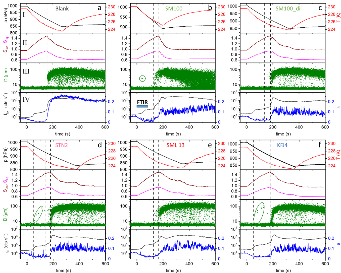
Figure 3: Time series of the AIDA records from the expansion cooling experiments started at 229 K for six different samples (a – f). The sample called “blank” refers to a commercial bulk Atlantic water sample that has already previously been probed in the AIDA chamber (Wagner et al., 2018). The four individual panels for each part show the following data: I: AIDA mean gas temperature (red line) and pressure (black line); II: saturation ratios with respect to ice ( S_{ice} , brown line) and supercooled water ( S_{liq} , magenta line); III: size-resolved single-particle scattering signals from the optical particle counter (green dots); IV: forward scattering intensity ( I_{for} , 2^\circ scattering angle, grey line) and backscattering linear depolarization ratio ( \delta , 178^\circ scattering angle, blue line). The blue horizontal bar in panel IV of Fig. 3b symbolises the time period where the series of FTIR spectra shown in Fig. 4 were recorded. See text for details.
