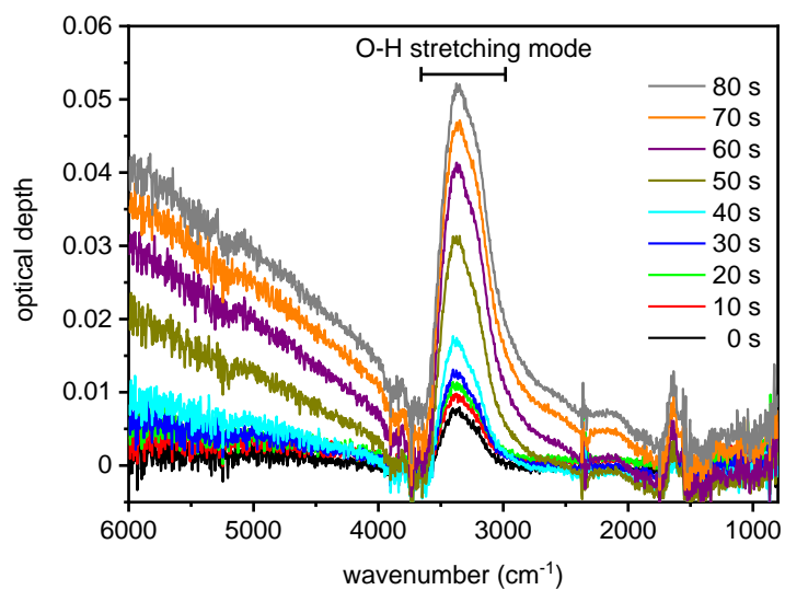
1345 Figure 4: Series of infrared extinction spectra that were recorded in the first 80 s during the expansion run with the particles generated from the SM100 culture (see Fig. 3b). The broad peak between about 3500 and 2800 \text{cm}^{-1} is due to the O – H stretching mode of liquid water. As described in the text, this spectra series is representative for all measurements with the various samples and is therefore also used to discuss the hygroscopic behaviour of the particles from the bulk Atlantic water sample in Sect. 3.2.1.
