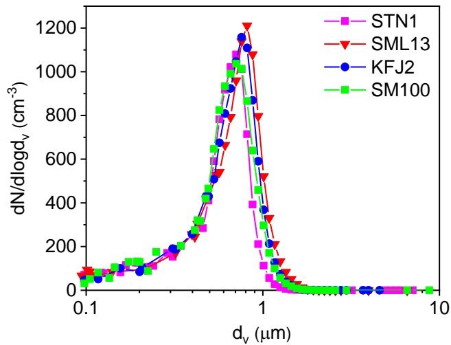
Figure 1: Number size distributions of aerosol particles generated by nebulising the STN1, SML13, KFJ2, and SM100 bulk solutions. The size spectra were measured at 298 K and RH < 3\% , thereby reflecting the dry particle diameters. The mobility and aerodynamic diameters from the SMPS and APS measurements were converted into the equal-volume sphere diameter, d_v , by assuming a dynamic shape factor of 1.08 (Hinds, 1999) and a particle density of 2.017 \text{ g cm}^{-3} for sea salt (Zieger et al., 2017).
