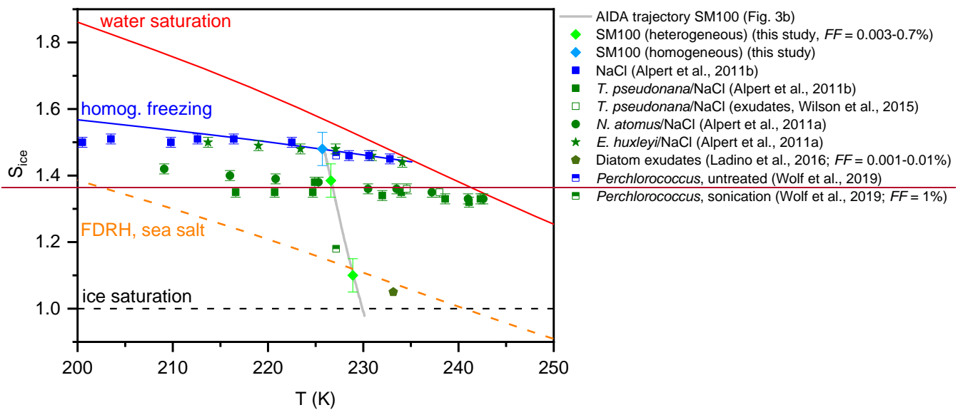
1370 Figure 7: Homogenous and heterogeneous ice nucleation onsets from the AIDA expansion run with the particles generated from the SM100 culture shown in Fig. 3b (light green and blue diamonds) in comparison with data from previous experiments with phytoplankton and marine bacterial species (see Sect. 1.2). The onsets from the immersion freezing measurements with the technique by Alpert et al. (2011a) were evaluated at median freezing temperatures for homogeneous and heterogeneous ice nucleation. The heterogeneous ice nucleation onsets from the AIDA and the various CFDC experiments correspond to different FF values as indicated in the legend and discussed in Sect. 4.1. The S_{ice} vs. T trajectory of the AIDA experiment is shown as the grey line. The other reference lines are the same as shown in Fig. 6. 1375
