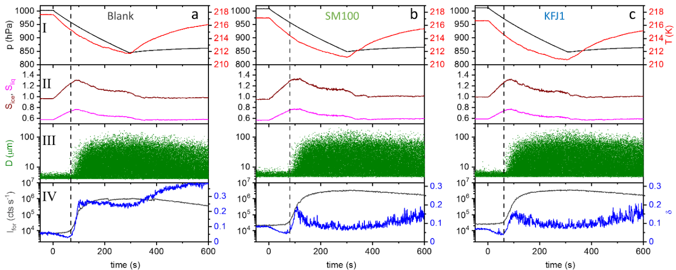
1350 Figure 5: Time series of the AIDA records from the expansion cooling experiments started at 217 K for three different samples (a – c). The sample called “blank” again refers to the commercial bulk Atlantic water sample that has already previously been probed in the AIDA chamber (Wagner et al., 2018). The individual panels show the same data types as in Fig. 3.
