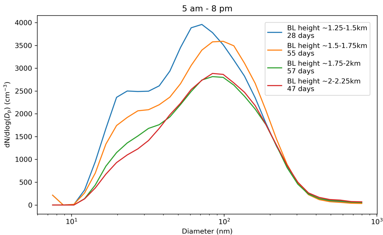
Figure 8. Impact of boundary layer height on the aerosol particle size distribution in dN/d\log(d_p) ( \text{cm}^{-3} ) measured at the surface during daytime mixing (from 5 am to 8 pm). Hourly median values are used. Number of days included in each boundary layer height range are given in the figure legend.
