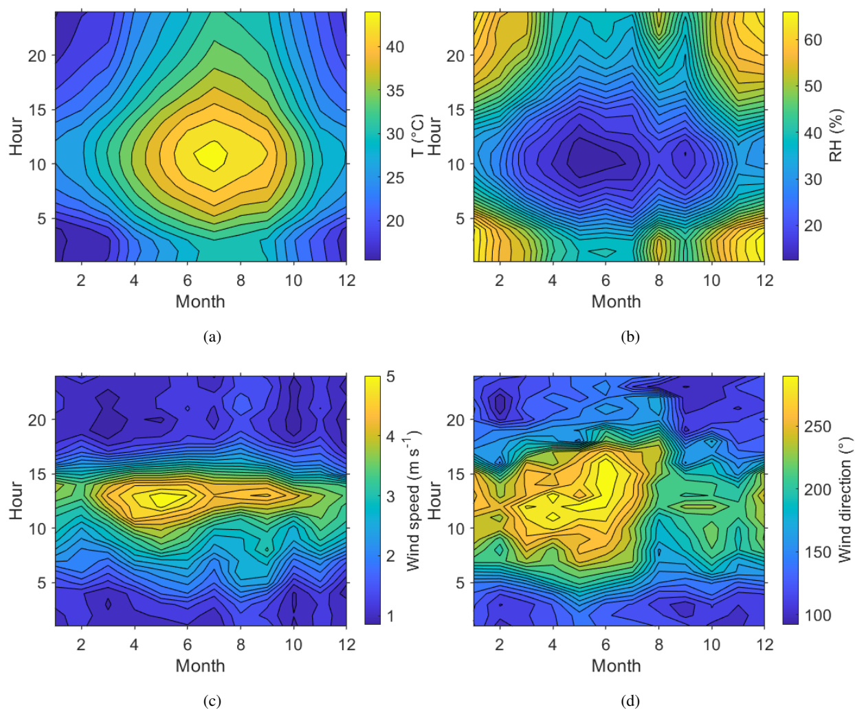
Figure 1. Seasonal and diurnal variation in surface a) temperature, T ( ^{\circ}\text{C} ), b) relative humidity, RH (%), c) wind speed, WS ( \text{m s}^{-1} ) and d) wind direction, WD ( ^{\circ} ). All measurements made at 7 m above ground level.
