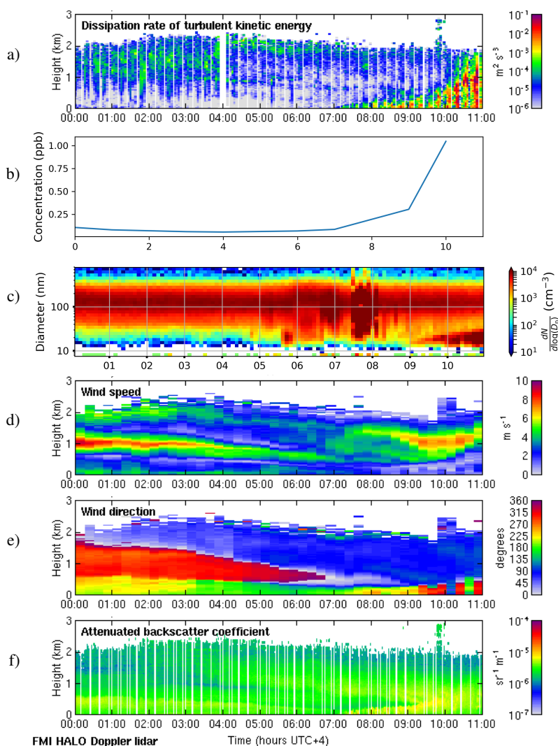
Figure 10. Deep boundary layer case on 19 May 2018. Panel a) displays a time-height plot of dissipation rate of turbulent kinetic energy, \epsilon , b) \text{SO}_2 concentration (ppb) measured at the surface, c) aerosol particle size distribution measured at the surface (the color indicates the concentration dN/d\log(D_p) in \text{cm}^{-3} ), and time-height plots of d) wind speed, e) wind direction, and f) attenuated backscatter coefficient. For all panels, the time axis is local time (hours UTC+4). The measurements in panels a), d), e) and f) were obtained from the HALO Doppler lidar.
