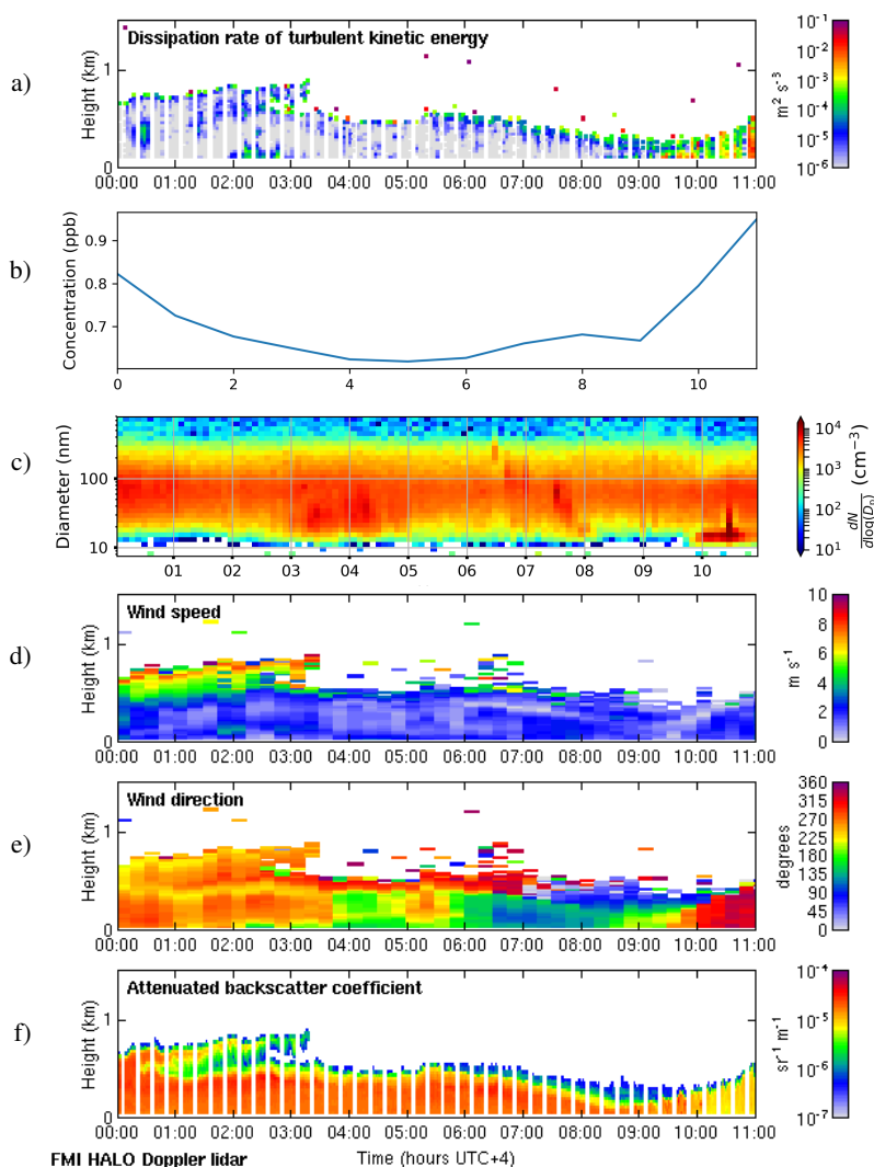
Figure B1. Shallow boundary layer case on 21 February 2018. Panel a) displays a time-height plot of dissipation rate of turbulent kinetic energy, \epsilon , b) \text{SO}_2 concentration (ppb) measured at the surface, c) aerosol particle size distribution measured at the surface (the color indicates the concentration dN/d\log(d_p) in \text{cm}^{-3} ), and time-height plots of d) wind speed, e) wind direction, and f) attenuated backscatter coefficient. For all panels, the time axis is local time (hours UTC+4). The measurements in panels a), d), e) and f) were obtained from the HALO Doppler lidar.
