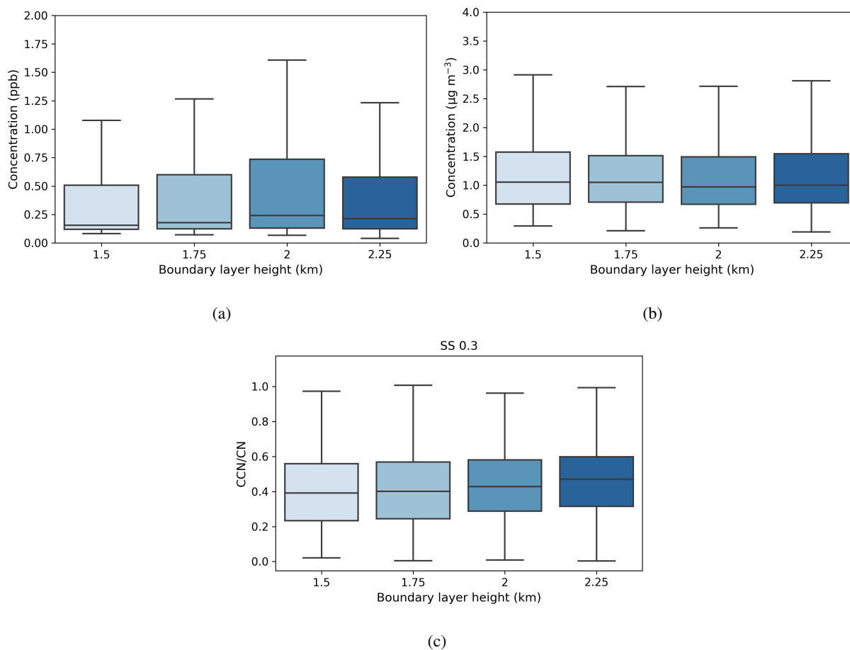
Figure 7. Box-and-whisker plots of hourly median values for a range of boundary layer heights for a) SO 2 (ppb), b) black carbon ( \mu\text{g m}^{-3} ), and c) activation fraction (CCN/CN) at a supersaturation of 0.3. The central line in the boxes indicate the median, and the bottom and top lines of the boxes indicate the 25 th and 75 th percentiles. The whiskers mark the most extreme data points that are not considered outliers. The boundary layer height value refers to the top of each height bin.
