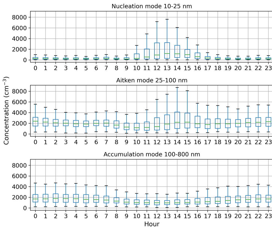
Figure 4. Box-and-whisker plots for hourly median concentration values (cm -3 ) of different aerosol particle modes. The central line (green) in each box indicates the median, and the bottom and top lines of the boxes indicate the 25 th and 75 th percentiles. The whiskers mark the most extreme data points that are not considered as outliers (within a range of 1.5 x interquartile range from the edges of the box).
