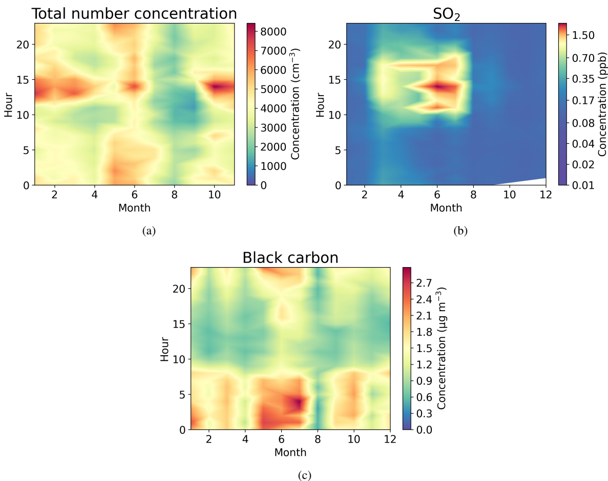
Figure 3. Seasonal-diurnal contour plots of a) aerosol particle total number concentration ( \text{cm}^{-3} ) measured with the DMPS, b) \text{SO}_2 concentration (ppb) measured with the \text{SO}_2 gas analyser and c) black carbon mass concentration ( \mu\text{g m}^{-3} ) measured with the Aethalometer. Hourly median values have been used.
