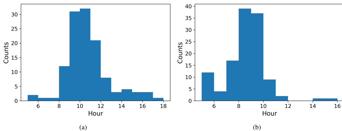
Figure 9. Histograms of start time for a) NPF events and b) boundary layer growth. The time axis is local time (hours UTC+4).
