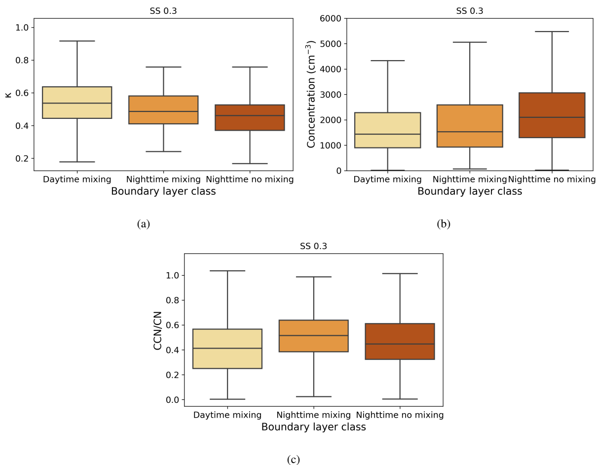
Figure 6. Box-and-whisker plots of hourly median values for 3 boundary layer conditions for a) \kappa parameter, b) CCN number concentration ( \text{cm}^{-3} ) and c) activation fraction (CCN/CN) at a supersaturation of 0.3. The central line in each box indicates the median, and the bottom and top lines of the boxes indicate the 25 th and 75 th percentiles. The whiskers mark the most extreme data points that are not considered as outliers.
