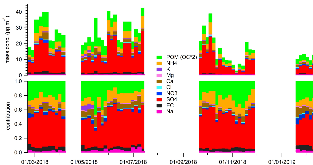
Figure 2. Aerosol particle chemical composition during the campaign.
