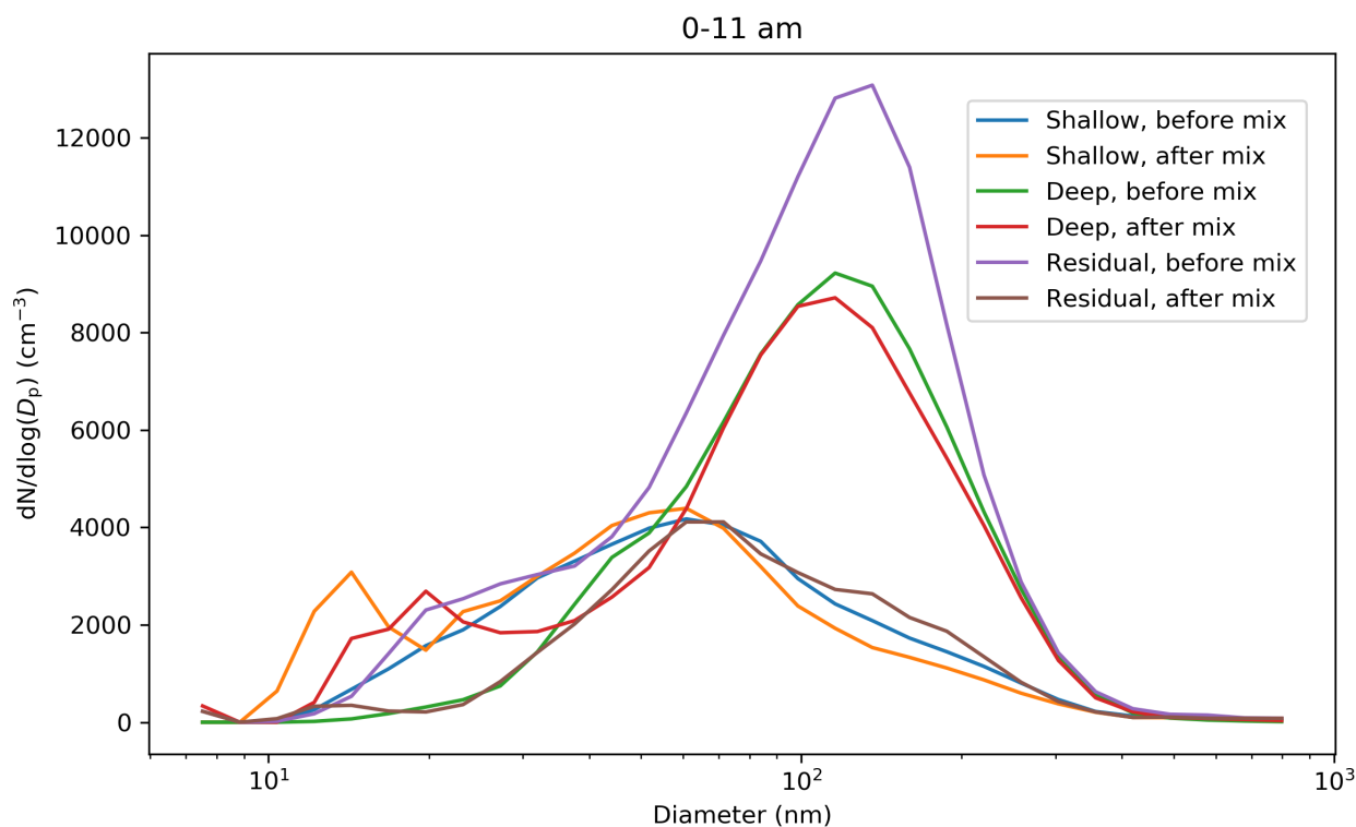
Figure 11. Impact of convective mixing on the aerosol particle size distributions measured at the surface for three case study days. Hourly median values are used. Aerosol particle size distributions are averaged from midnight to start of convective mixing, and from start of convective mixing to 11 am. Convective mixing was assumed to start at 9 am for the shallow boundary layer case study, 7 am for the deep boundary layer case study, and around 8 am for the case study entraining a residual layer with different properties (denoted residual in the plot).
