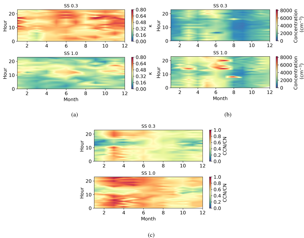
Figure 5. Seasonal-diurnal contour plots of a) \kappa parameter, b) CCN number concentration ( \text{cm}^{-3} ) and c) activation fraction (CCN/CN), in different supersaturations. Hourly median values have been used.
