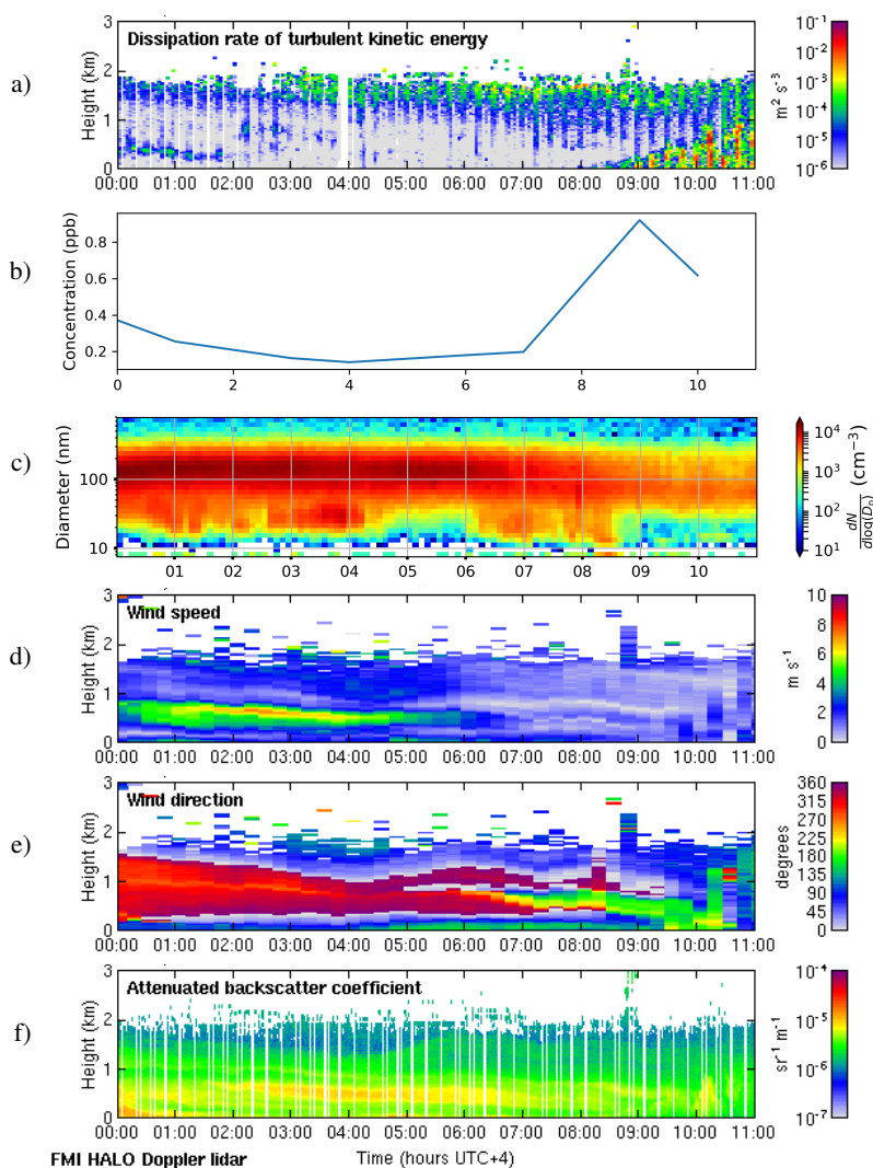
Figure C1. Residual layer case on 8 May 2018. Panel a) displays a time-height plot of dissipation rate of turbulent kinetic energy, \epsilon , b) \text{SO}_2 concentration (ppb) measured at the surface, c) aerosol particle size distribution measured at the surface (the color indicates the concentration dN/d\log(d_p) in \text{cm}^{-3} ), and time-height plots of d) wind speed, e) wind direction, and f) attenuated backscatter coefficient. For all panels, the time axis is local time (hours UTC+4). The measurements in panels a), d), e) and f) were obtained from the HALO Doppler lidar.
