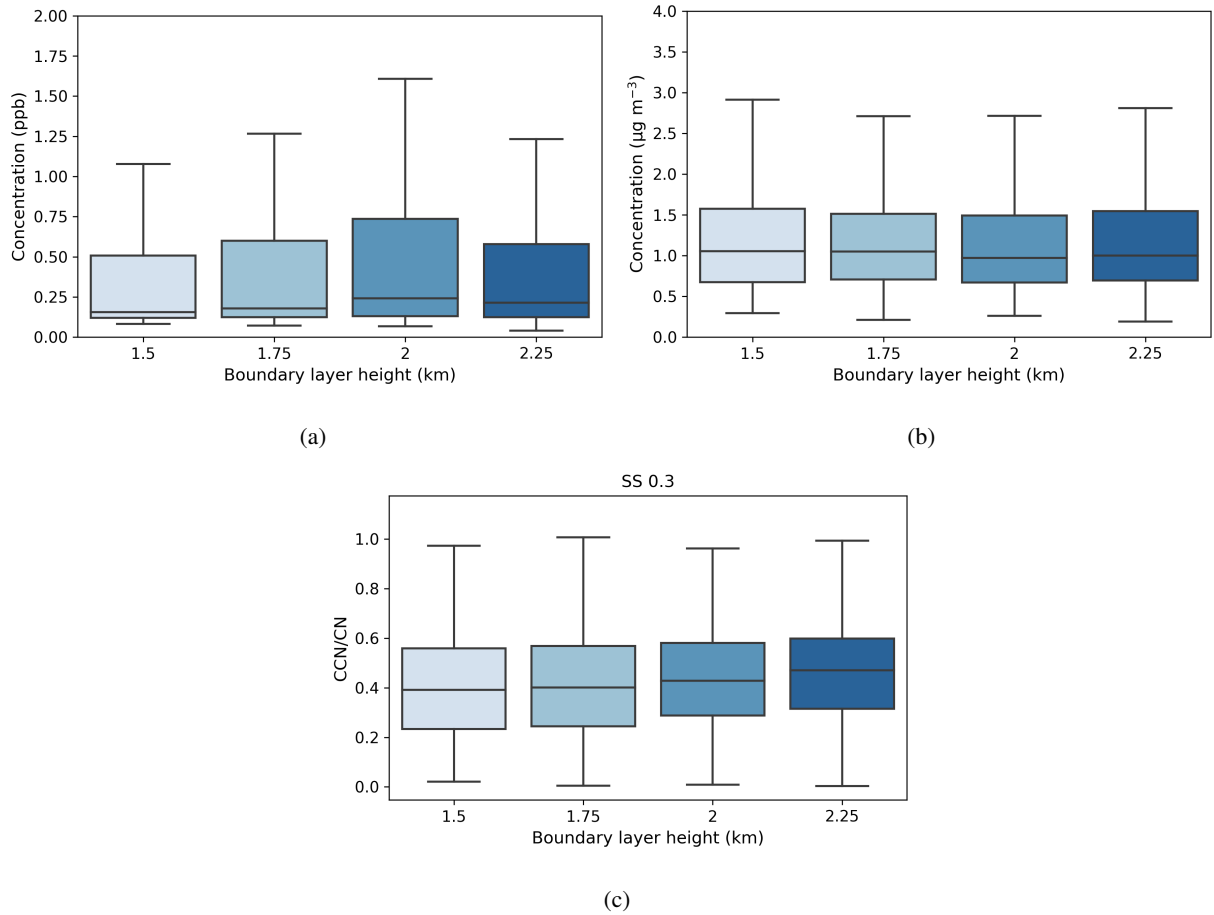
Figure 8. Box-and-whisker plots of hourly median values for a range of boundary layer heights for a) \text{SO}_2 (ppb), b) black carbon ( \mu\text{g m}^{-3} ), and c) activation fraction (CCN/CN) at a supersaturation of 0.3. The central line in the boxes indicate the median, and the bottom and top lines of the boxes indicate the 25 th and 75 th percentiles. The whiskers mark the most extreme data points that are not considered outliers. The boundary layer height value refers to the top of each height bin.
