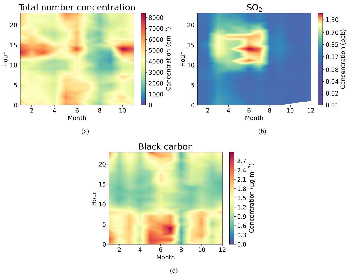
Figure 4. Seasonal-diurnal contour plots of a) aerosol particle total number concentration ( \text{cm}^{-3} ) measured with the DMPS, b) \text{SO}_2 concentration (ppb) measured with the \text{SO}_2 gas analyser and c) black carbon mass concentration ( \mu\text{g m}^{-3} ) measured with the Aethalometer. Hourly median values have been used.
