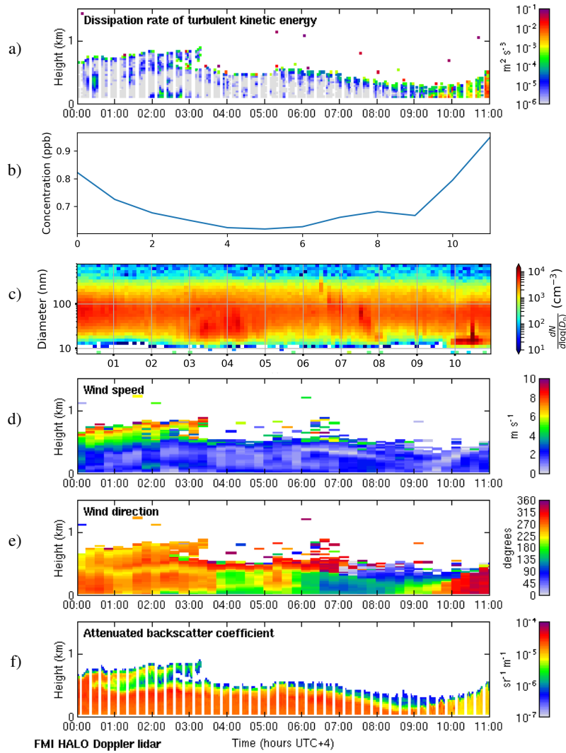
Figure C1. Shallow boundary layer case on 21 February 2018. Panel a) displays a time-height plot of dissipation rate of turbulent kinetic energy, \epsilon , b) SO 2 concentration (ppb) measured at the surface, c) aerosol particle size distribution measured at the surface (the color indicates the concentration dN/d\log(d_p) in \text{cm}^{-3} ), and time-height plots of d) wind speed, e) wind direction, and f) attenuated backscatter coefficient. For all panels, the time axis is local time (hours UTC+4). The measurements in panels a), d), e) and f) were obtained from the HALO Doppler lidar.
