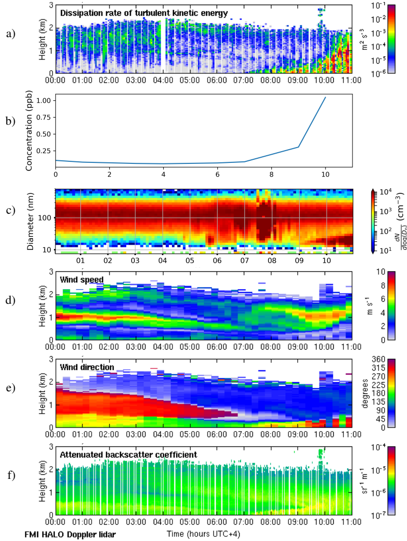
Figure 11. Deep boundary layer case with transport aloft on 19 May 2018. Panel a) displays a time-height plot of dissipation rate of turbulent kinetic energy, \epsilon , b) \text{SO}_2 concentration (ppb) measured at the surface, c) aerosol particle size distribution measured at the surface (the color indicates the concentration dN/d\log(d_p) in \text{cm}^{-3} ), and time-height plots of d) wind speed, e) wind direction, and f) attenuated backscatter coefficient. For all panels, the time axis is local time (hours UTC+4). The measurements in panels a), d), e) and f) were obtained from the HALO Doppler lidar.
