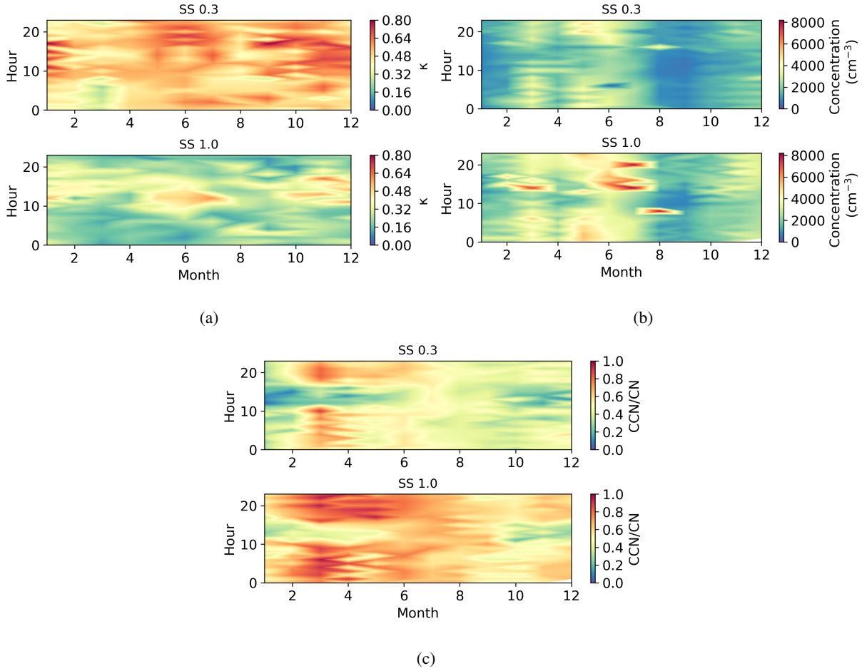
Figure 6. Seasonal-diurnal contour plots of a) \kappa parameter, b) CCN number concentration ( \text{cm}^{-3} ) and c) activation fraction (CCN/CN), in different supersaturations. Hourly median values have been used.
