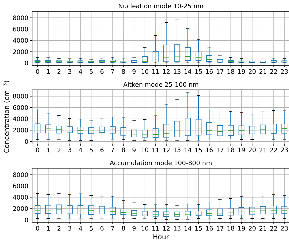
Figure 5. Box-and-whisker plots for hourly median concentration values (cm -3 ) of different aerosol particle modes. The central line (green) in each box indicates the median, and the bottom and top lines of the boxes indicate the 25 th and 75 th percentiles. The whiskers mark the most extreme data points that are not considered as outliers (within a range of 1.5 x interquartile range from the edges of the box).
