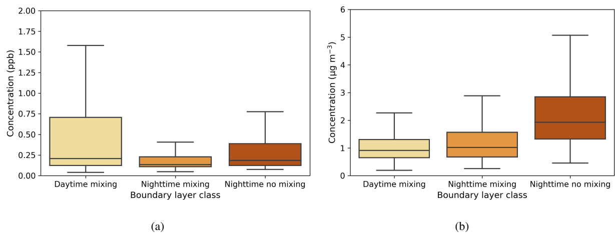
Figure A1. Box-and-whisker plots of hourly median values for 3 boundary layer conditions for a) \text{SO}_2 (ppb) and b) black carbon ( \mu\text{g m}^{-3} ). The central line in the boxes indicate the median, and the bottom and top lines of the boxes indicate the 25 th and 75 th percentiles. The whiskers mark the most extreme data points that are not considered as outliers.
