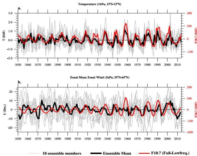
120 Fig. 3. Direct solar cycle signal in the upper stratosphere. a) Time series of the tropical stratopause temperature (1hPa, 15°S-15°N) averaged over the winter season (DJF) for the individual ensemble members (grey thin lines), ensemble mean (black thick line) and the solar cycle index F10.7 (red line). b) Same as a), but for December zonal mean zonal wind averaged over 55-65°N, 1hPa, smoothed with a 3-year running mean. To isolate 11-year solar cycle effects, differences between the FULL and the LOWFREQ ensemble simulations have been calculated. The grey lines include internal variability and the 11-year solar signal, their spread represents the internal variability, and the ensemble mean (thick black line) represents the 11-year solar cycle. The 11-year solar cycle has been isolated in a similar way from the original solar forcing time series by subtracting the low-frequency part of the solar forcing (Fig. S1). 125
