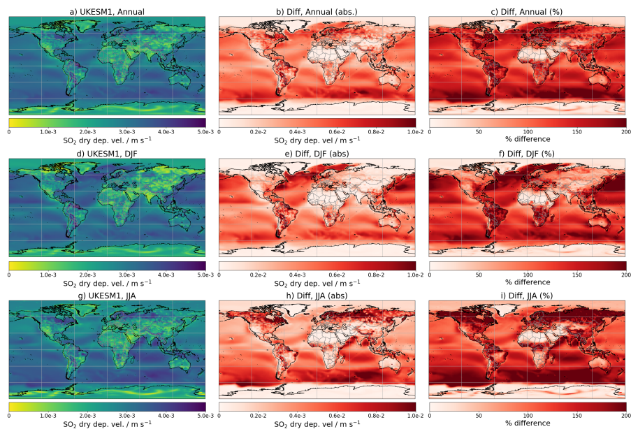
Figure 10. SO 2 dry deposition velocity for UKESM1, (left column); absolute difference in SO 2 dry deposition velocity for UKESM1-SO 2 - UKESM1, (middle column) and percentage difference in SO 2 dry deposition velocity for UKESM1-SO 2 - UKESM1, (right column). Annual means are shown in a–c, the DJF mean is shown in d–f and the JJA mean is shown in g–i). Each plot shows mean data for the period 1987–2014. Deposition velocity is calculated from the simulated surface SO 2 and dry deposition flux values and represents the ‘bulk’ deposition velocity for each model grid cell.
