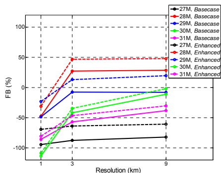
Figure 11. Daily (a) fractional bias vs. domain resolution and (b) correlation coefficient vs. domain resolution for the Basecase (solid lines) and Enhanced (dash lines) simulations.
