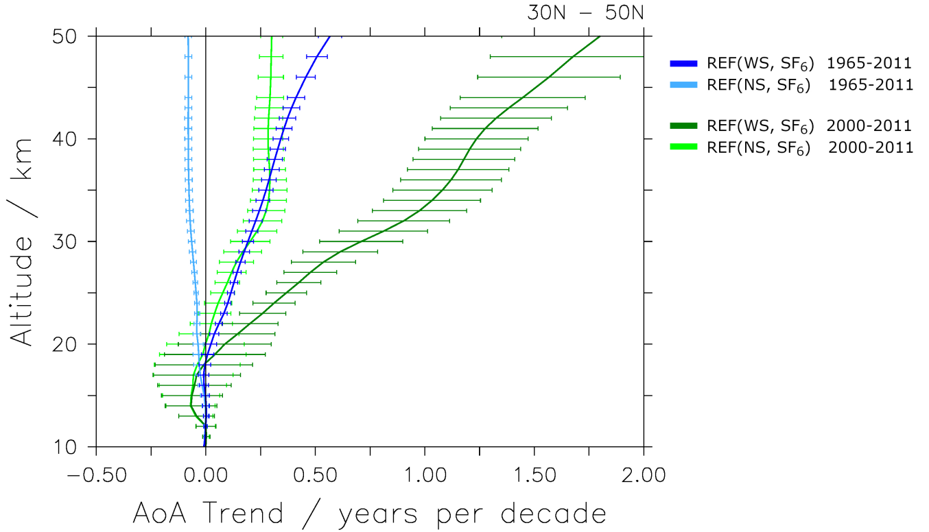
Figure 5. Vertical profile of the linear trends of \text{AoA}(\text{WS}, \text{SF}_6)_{\text{REF}} and \text{AoA}(\text{NS}, \text{SF}_6)_{\text{REF}} over 30°N-50°N, calculated for the two time periods 1965-2011 and 2000-2011. Error bars depict the 2\sigma standard deviation of the trend over the respective time period, and the black vertical line denotes the zero-line.
