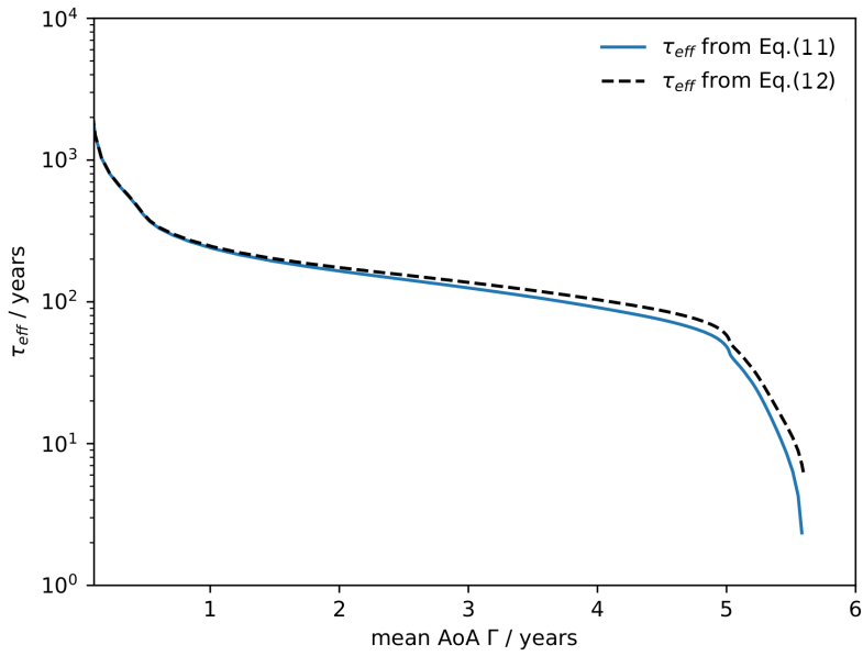
Figure 8. Effective lifetime derived from average mid-latitude (30°N-50°N) ideal mean AoA and apparent mean AoA (from the linearly increasing SF 6 -like tracer) from the TS2000 simulations. The calculation of \tau_{eff} is based on Eq.11 (blue solid) and its linear approximation Eq.12 (black dashed).
