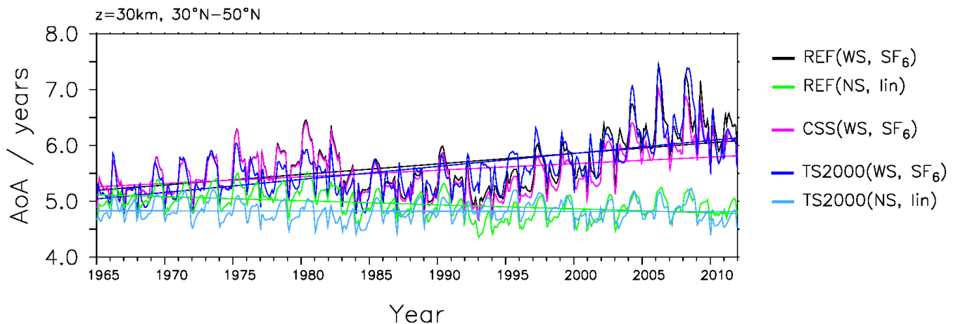
Figure 6. AoA (at 10 hPa, averaged over 30^\circ\text{N} - 50^\circ\text{N} ) time series and linear regression of sensitivity experiments TS2000( \text{WS}, \text{SF}_6 ), TS2000( \text{NS}, \text{lin} ), and CSS( \text{WS}, \text{SF}_6 ) shown in dark blue, light blue, and pink, respectively. Reference simulations \text{REF}(\text{WS}, \text{SF}_6) and \text{REF}(\text{NS}, \text{lin}) shown in black and green, respectively.
