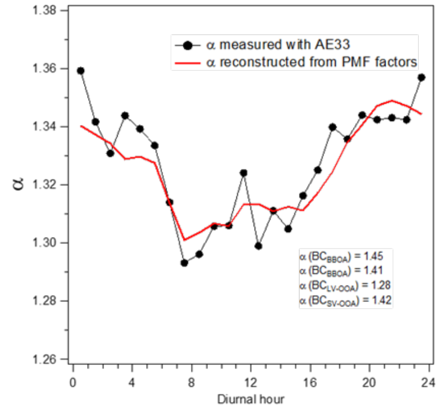
Figure R2. Comparison of \alpha values measured with AE33 and reconstructed from the AMS PMF data with multi-linear regression at the residential site. Scatter plot (left) and average diurnal variations (right).
