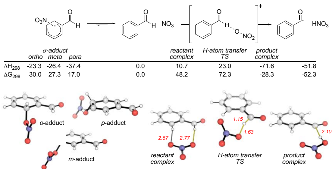
Figure 6. Pathways for the reaction between BA and \text{NO}_3 calculated using DLPNO-CCSD(T)/cc-pVTZ//BH&HLYP/6-311G(d,p). Enthalpic and Gibbs energy values are in kJ/mol.
