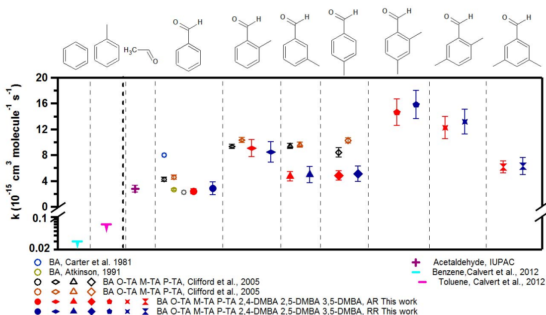
445 Figure 5 The measured rate coefficients for the reactions of NO 3 radical with the seven aldehydes studied here. The results of previously reported rate coefficients are also shown (values are presented in Table 2). The rate coefficient for acetaldehyde of k_{(\text{CH}_3\text{CHO})} = (2.7 \pm 0.5) \times 10^{-15} \text{ cm}^3 \text{ molecule}^{-1} \text{ s}^{-1} is from IUPAC recommendations. The rate coefficients for benzene, k_{(\text{benzene})} < 3 \times 10^{-17} \text{ cm}^3 \text{ molecule}^{-1} \text{ s}^{-1} , and for toluene, k_{(\text{toluene})} \leq 6.6 \times 10^{-17} 450 \text{cm}^3 \text{ molecule}^{-1} \text{ s}^{-1} are from Calvert et al., 2011. 88.4 90.2
