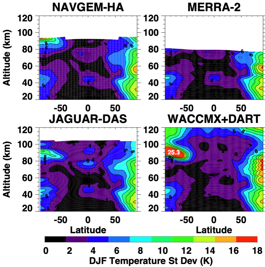
Figure S1. Latitude-altitude cross sections of the standard deviation in DJF mean temperatures from NAVGEM-HA, MERRA2, JAGUAR-DAS, and WACCMX+DART. Contour interval is 2 K.
