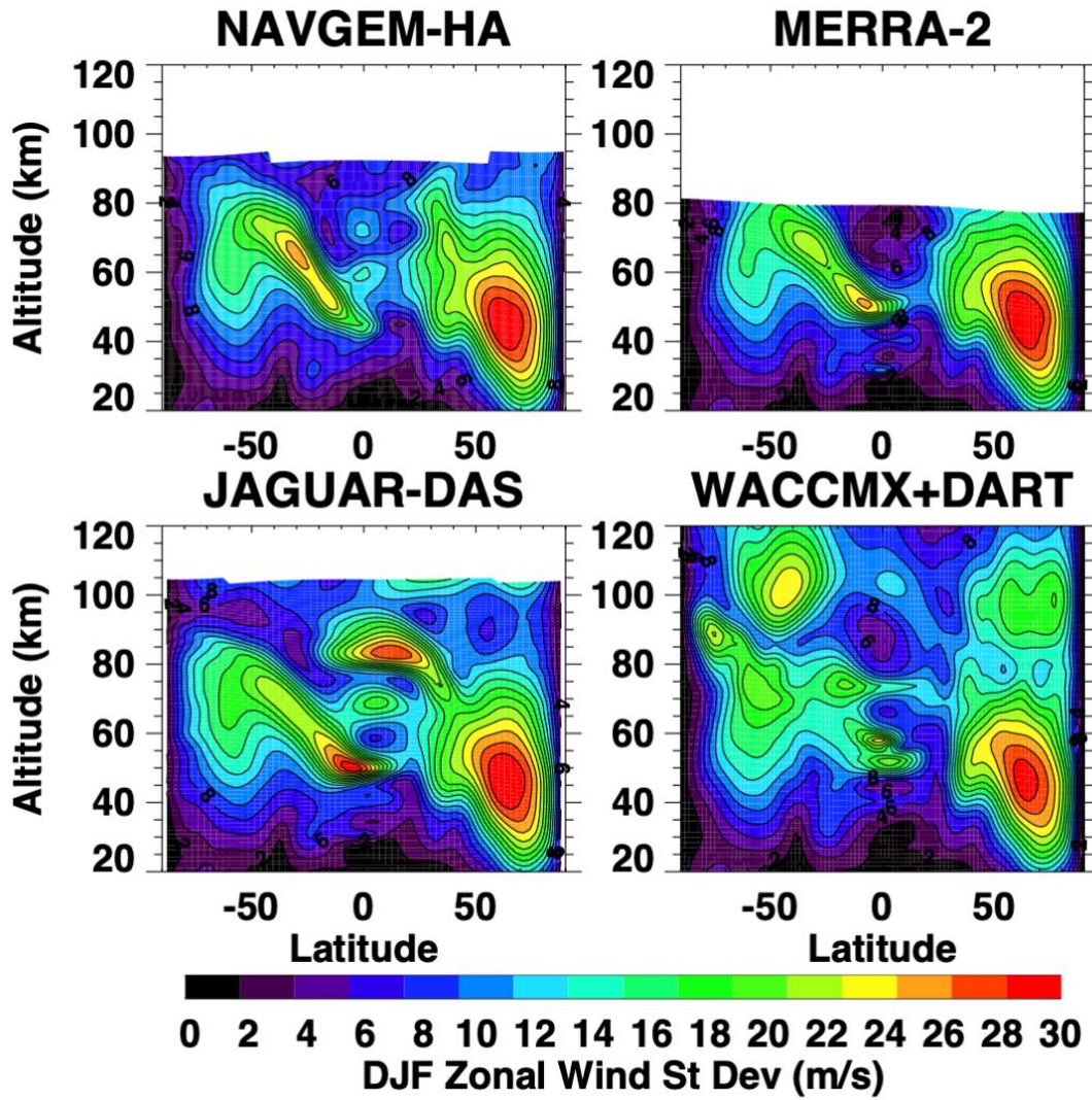
Figure S2. Latitude-altitude cross sections of the standard deviation in DJF mean zonal wind from NAVGEM-HA, MERRA2, JAGUAR-DAS, and WACCMX+DART. Contour interval is 2 \text{ m s}^{-1} .
