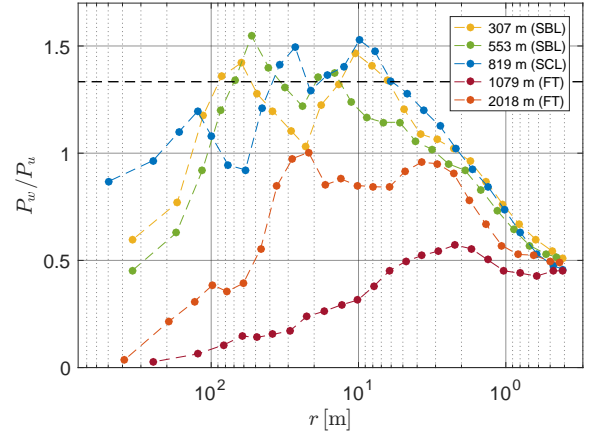
Figure 17. Spectral anisotropy ratio in the coupled STBL (flight #5). The horizontal dashed line denotes the 4/3 level expected for isotropy in the inertial range.
