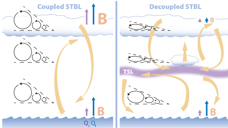
Figure 21. Schematic of main processes in the coupled (left) and decoupled (right) STBL: primary circulation (yellow arrows), turbulence eddy cascade (circular arrows confined in an angle with extent proportional to inertial range scaling exponent p ), TKE buoyancy production (red B letter of size proportional to strength), sensible and latent heat fluxes (purple and blue arrows, respectively, of length proportional to strength) at the surface and in the cloud top region.
