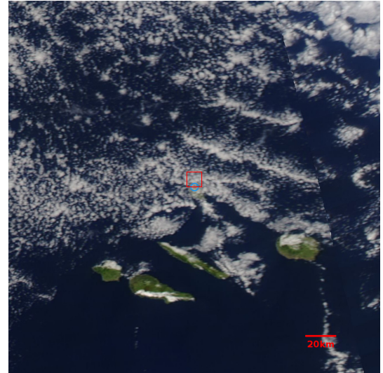
Figure 1. Satellite true color image (250 x 250 km) taken on 8 July 2017 at 15:45 UTC (i.e. during flight #5, the time given corresponds to the left swath covering most of the image) by the MODIS instrument on Aqua overpassing Azores, centered on Graciosa airport (blue circle), with overlaid helicopter operation area (red box). The image was acquired from NASA Worldview Snapshots.
