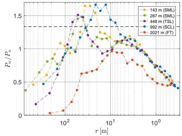
Figure 18. As in Fig. 17 but for the decoupled STBL (flight #14).
