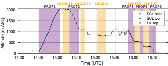
Figure 2. ACTOS altitude in flight #5 with marked selected profiles (purple) and horizontal legs (yellow). PROFs are ordered chronologically, LEGs are ordered according to their altitude. Line style styles of the profiles is PROFs are consistent with the figures in following sections. Altitude ranges corresponding to PROF2-PROF5 of this flight do not overlap and are all marked with dashed lines. Dots indicate the penetrations of the boundaries of the specific sublayers described in sec. 3.
