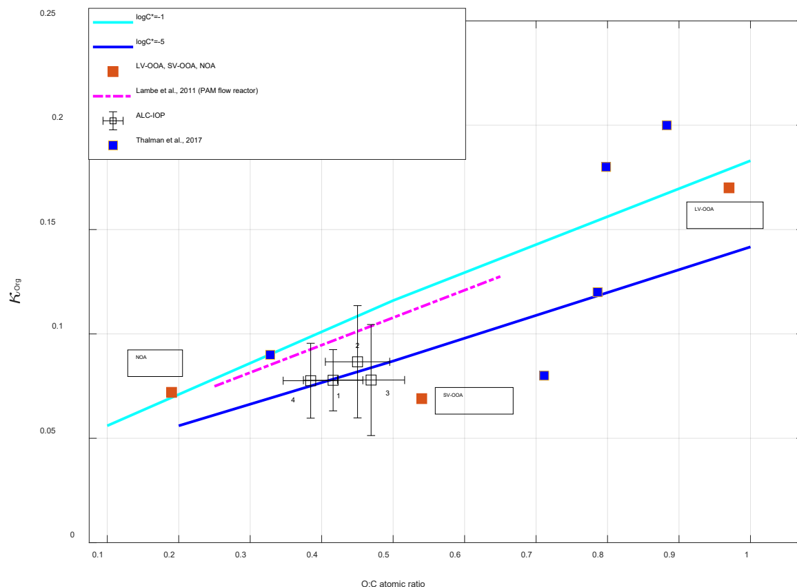
Figure 2. Derived \kappa_{org} as a function of O:C atomic ratio for four clusters, and the \kappa_{org} values of SOA positive matrix factorization (PMF) factors (LV-OOA, SV-OOA, NOA) derived from measurements during the ALC-IOP. Also shown with the predicted variation for organics with a mean \log C^* equals to -1 and -5, and the \kappa_{org} values of SOA PMF factors from measurements during GoAmazon 2014/5 (Thalman et al., 2017), and the relationship between \kappa_{org} and O:C for SOA derived from a laboratory study (Lambe et al., 2011).
