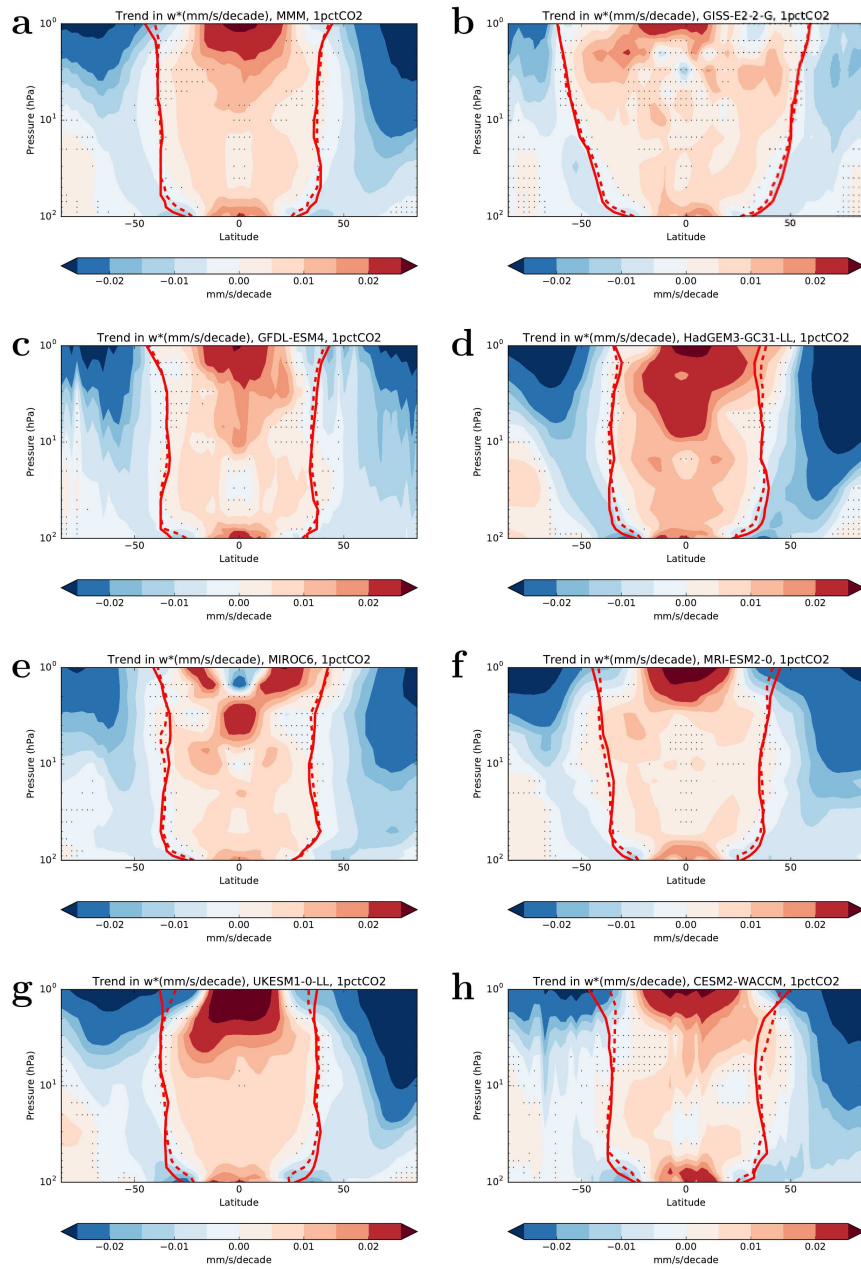
Figure 8. Trend in \bar{w}^* ( mm \cdot s^{-1} \cdot decade^{-1} ), computed using 150 year time series from 1pctCO2 experiments. The top left panel shows multi-model mean (MMM). All other panels show individual models. Turn around latitudes show region of upwelling in first 20 years (solid red lines) and last 20 years (dashed red lines) of these 150 year simulations. Stippling in top left panel denotes regions where it is not the case that the trend is significant in at least 66% of models. Stippling in all other panels denotes regions where the trend in that model is not significant.
