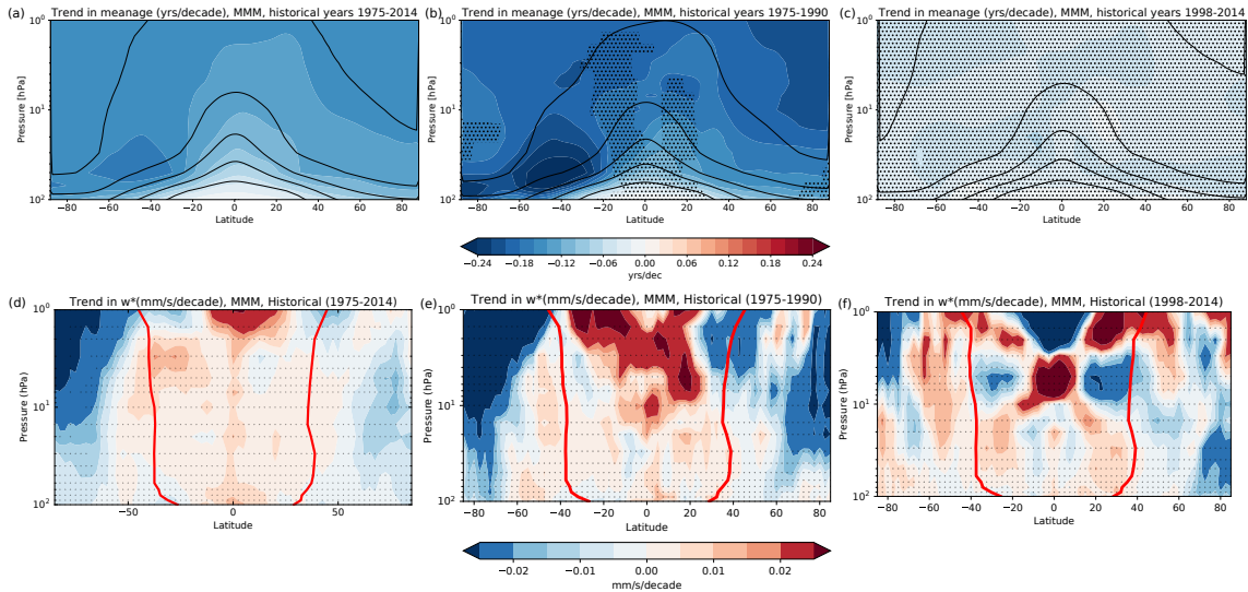
Figure 4. Multimodel mean linear trend in AoA (top panels, years/decade) and \bar{w}^* (bottom panels, in mm \cdot s^{-1} \cdot decade^{-1} ) from historical simulations in shading over years 1975-2014 (a and d) 1975-1990 (b and e) and 1998-2014 (c and f). In top panels the contours show the climatological AoA (years, contour interval 1 year, lower contour: 1 year). In the bottom panels the red contours show the turnaround latitudes averaged over each corresponding period. Stippling indicates statistically insignificant trends obtained with a Student's t test at 95% confidence level for more than 66% of the models.
