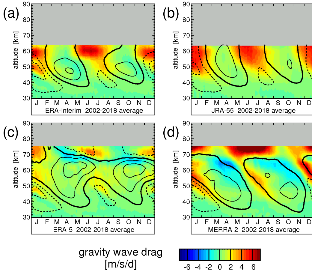
Figure 4. ERA-Interim estimates Typical seasonal variation of the “total” gravity wave drag averaged \overline{X}_{GW} estimated from the TEM momentum budget. The values are averages over 10^{\circ}\text{S} – 10^{\circ}\text{N} for and the 2002–2018 time period, as well as 2002–2018 for the multi-year average over these years four reanalyses (a) ERA-Interim, (b) JRA-55, (c) ERA-5, and (d) MERRA-2. Overplotted are contour lines are ERA-Interim zonal winds averaged over 10^{\circ}\text{S} – 10^{\circ}\text{N} (cf. Fig ?? of the respective wind data set). Contour line increment is 20\text{ m s}^{-1} . The zero wind line is highlighted in bold solid, and westward (eastward) zonal wind is winds are indicated by dashed (solid) contour lines.
