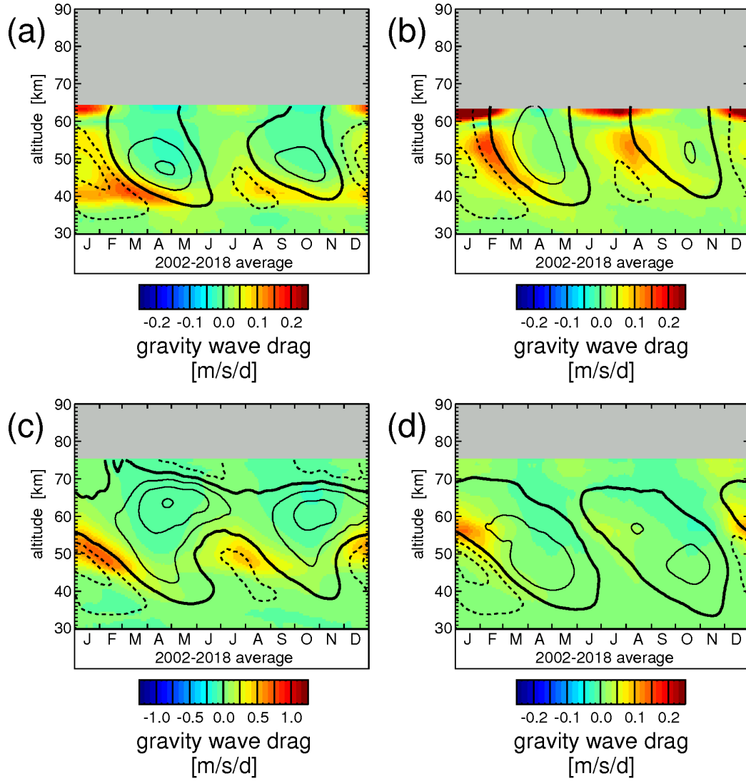
Figure 5. Same as Fig. 224, but for JRA-55 the zonal gravity wave drag \overline{X}_{res}(k > 20) of model-resolved gravity waves at zonal wavenumbers exceeding k = 20 .
