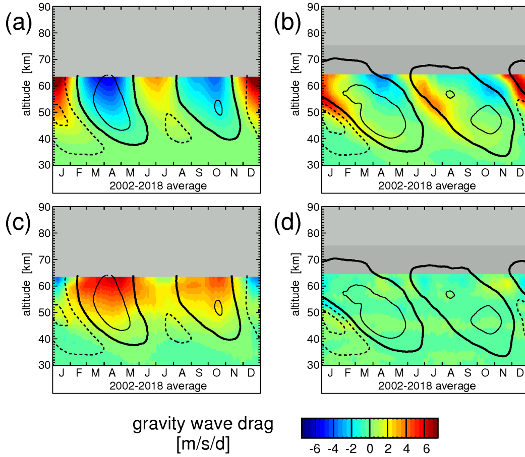
Figure 6. Typical seasonal variation of parameterized gravity wave drag \overline{X}_{drag} for the reanalyses (a) JRA-55 and (b) MERRA-2, as well as the gravity wave drag term \overline{X}_{imbalance} for (c) JRA-55 and (d) MERRA-2. The term \overline{X}_{imbalance} includes, but for MERRA-2 example, the model imbalance that is caused by data assimilation. Again, values are averages over 10^{\circ}\text{S} – 10^{\circ}\text{N} and the time period 2002–2018, and contour lines of the respective wind data set are overplotted. Contour line increment is 20\text{ m s}^{-1} . The zero wind line is highlighted in bold solid, and westward (eastward) winds are indicated by dashed (solid) contour lines.
