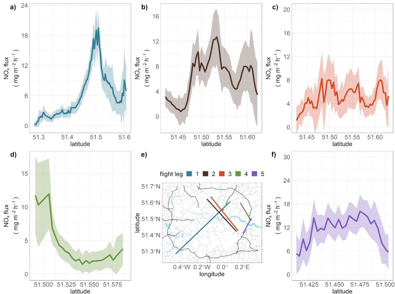
Figure 5. Ensemble \text{NO}_x flux flight track averages (400 m) across the campaign, with the shaded area representing the average random error divided by the square root of the number of sample points which went into each mean (error/sqrt(n)). The top row (a, b & c) shows flight transects 1, 2 and 3 which ran over central areas of London such as City of London Borough. The bottom row (d & f) transects 4 and 5, ran over eastern regions of Greater London, home to industry and major road network. e) shows each individual track transect overlaid onto the OpenStreetMap's; major road infrastructure, local boundaries, and rivers around the GLR (OpenStreetMap contributors, 2021; Padgham et al., 2020).
