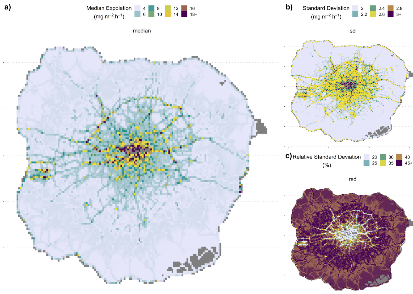
Figure 8. The median average projection of NO x emissions ( \text{mg m}^{-2} \text{h}^{-1} ) at 400 m 2 resolution from all flight transect data. The standard deviation (b) and relative standard deviation (c) show the variability between individual flight transect projects. Missing areas outside of the ERF training dataset are shown in grey.
