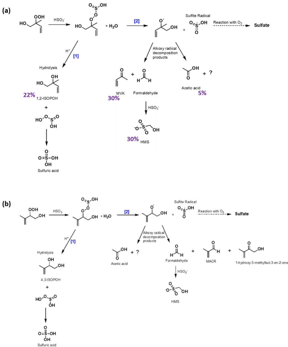
Figure 3. Proposed chemical mechanisms of the oxidation of \text{SO}_{2,\text{aq}} by a) 1,2-ISOPOOH with carbon yields of identified products at \text{pH}=5.5 (Table 2) presented in purple and b) 4,3-ISOPOOH. There are two competing mechanisms: after ISOPOOH reacts with \text{SO}_{2,\text{aq}} , displacing water, a hydrolysis reaction is taking place [1] or an O-O bond breakage [2]. In mechanism [1], the product hydrolysis results in the same intermediate that the reaction of \text{SO}_{2,\text{aq}} with \text{H}_2\text{O}_2 is forming and either a formation of a diol or an epoxide is being generated (Figure S2). In mechanism [2], an alkoxy radical and sulfite radical are formed leading to the production
