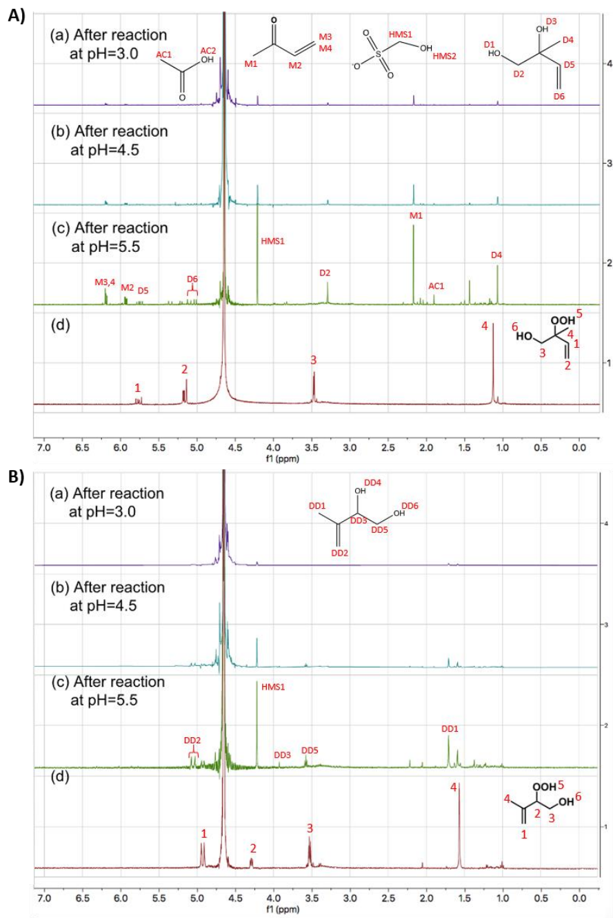
Figure 1: Proton NMR spectra ( ^1\text{H-NMR} , 400MHz, \text{D}_2\text{O} ) of (A) 1,2-ISOPOOH (d) and the products of the reaction of \text{SO}_{2,\text{aq}}+1,2 -ISOPOOH at (a) pH=3, (b) pH=4.5 and (c) pH=5.5 and (B) 4,3-ISOPOOH (d) and the products of the reactions of \text{SO}_{2,\text{aq}}+4,3 -ISOPOOH at (a) pH=3, (b) pH=4.5 and (c) pH=5.5. The concentration of the ISOPOOH isomers was 1 mM and the concentration of \text{SO}_{2,\text{aq}} was 2 mM. The spectra are focused on the areas of change. Chemical structures of (A,d) 1,2-ISOPOOH and (B,d) 4,3-ISOPOOH are presented. The labels at each peak represent the hydrogens of the compounds and the spectra are shifted for \text{D}_2\text{O} at 4.67 ppm.
