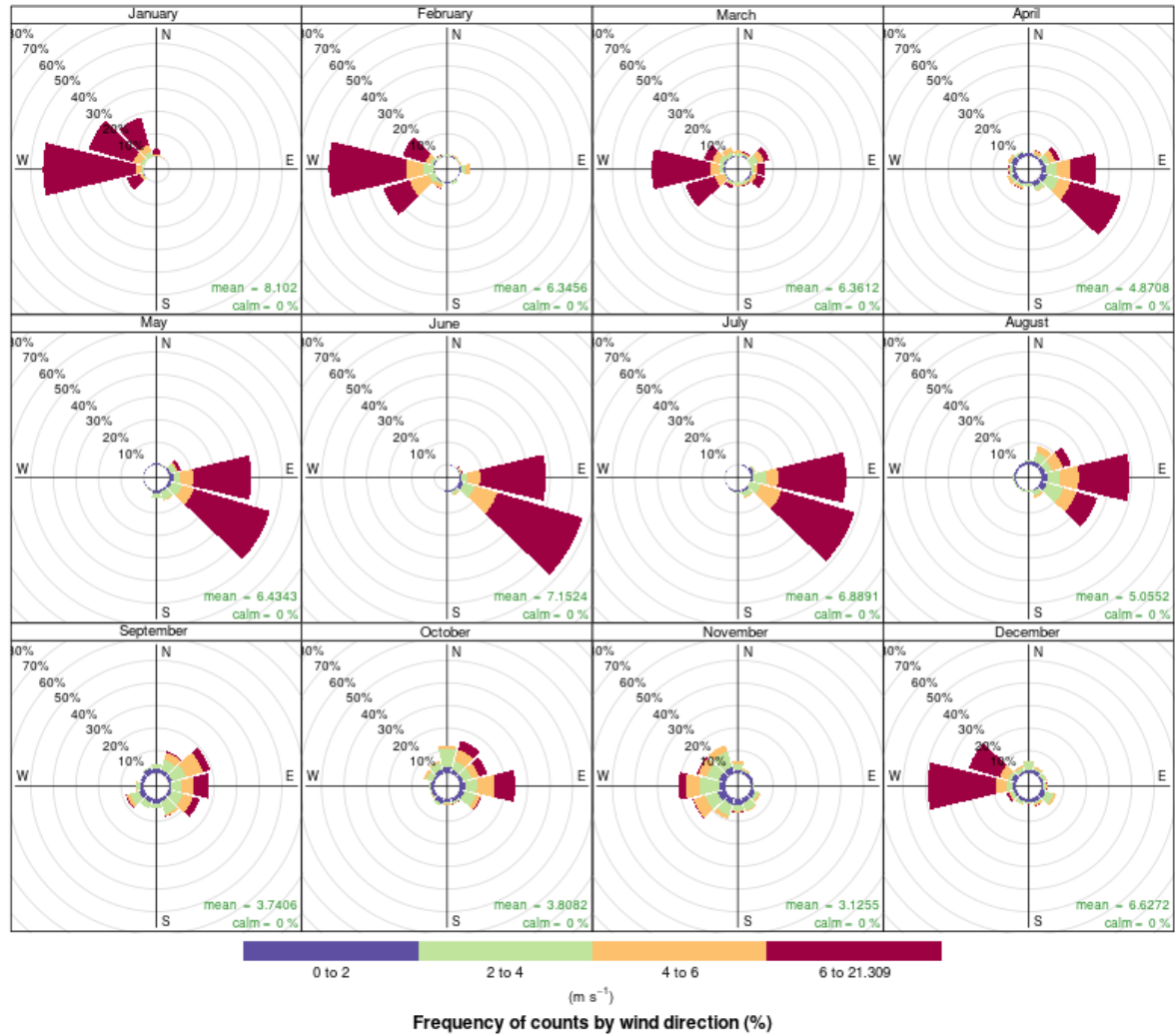
Figure S3. Wind rose TCCON Darwin location for 2015.
