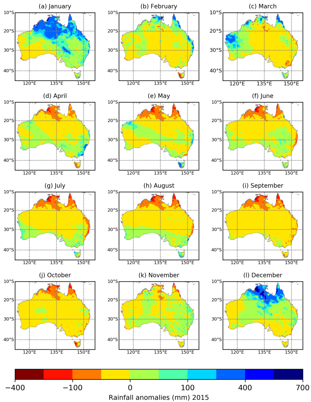
Figure S2. Rainfall anomalies (mm) for 2015.
