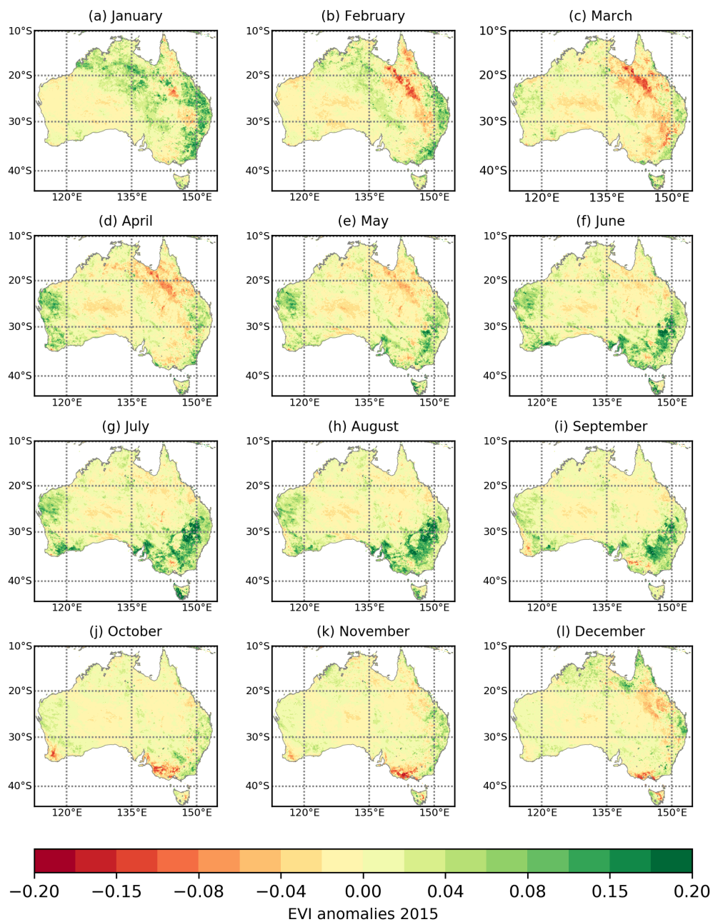
Figure S1. Enhanced vegetation index (EVI) anomalies for 2015.
