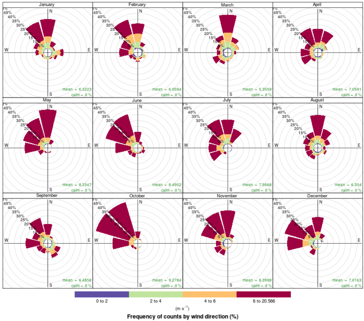
Figure S5. Wind rose TCCON Lauder location for 2015.
