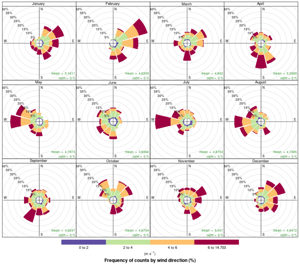
Figure S4. Wind rose TCCON Wollongong location for 2015.
