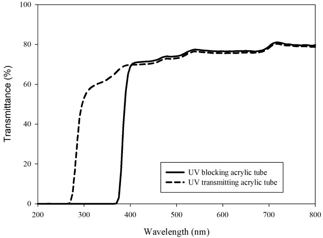
20 Figure S1. Light transmittance of the two acrylic tubes used in the experiments
