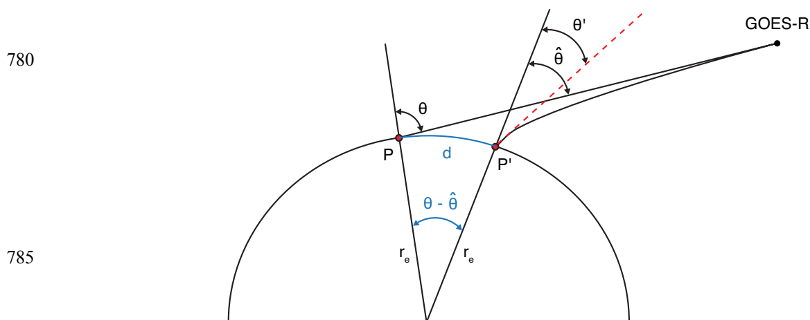
Figure 5. Terrestrial refraction geometry after Noerdlinger (1999). The distant observer (GOES-R) views point P' , which is displaced by distance d and registered in the satellite image at point P . Noerdlinger (1999) provides analytical formulas that relate the known zenith angle \theta of the unrefracted ray to \hat{\theta} and \theta' , from which the horizontal displacement along the surface can be calculated using the local Earth curvature radius r_e ( = 6,371,000 m in the spherical model).
