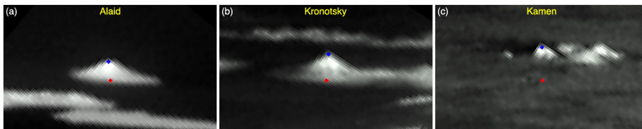
Figure 7. GOES-17 band 2 fixed grid image after 8x magnification of (a) Alaid (Atlasov Island, 2339 m) on 30 March 2020 at 00:00 UTC, (b) Kronotsky (3528 m) on 13 June 2020 at 23:00 UTC, and (c) Kamen (4619 m) on 8 April 2020 at 19:00 UTC. The image pixel corresponding to the geodetic latitude/longitude of the vent is marked by a red diamond. The visually identified peak with a 1-pixel radial refraction correction applied is marked by a blue diamond. The images were rotated clockwise by the geodetic colatitude angle. In panel (c) , the tops of (left to right or south to north) Kamen, Ushkovskiy (3891 m), Klyuchevskoy (4835 m), and Krestovskiy (4048 m) are seen peeking through the cloud layer.
