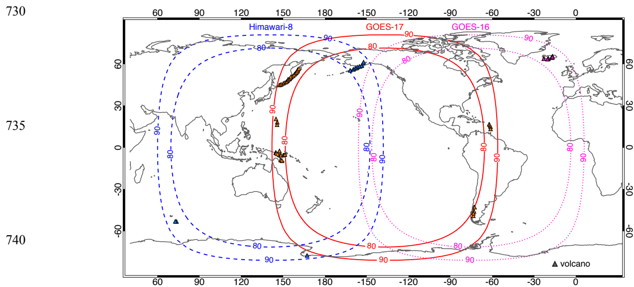
745 Figure 2. Limb area between the 80° and 90° view zenith angle isolines of the GOES-16 (dotted magenta), GOES-17 (solid red), and Himawari-8 (dashed blue) full disk. Triangles indicate volcanoes that erupted within the limb areas in the past 100 years.
