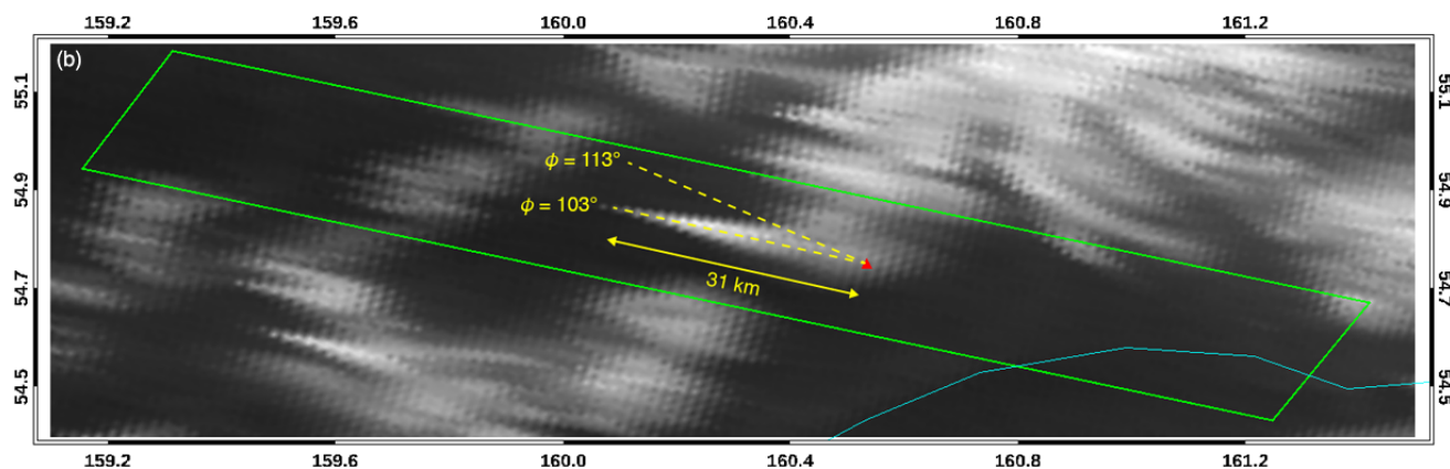
Figure 8. GOES-17 band 2 image of Kronotsky (3528 m) on 13 June 2020 at 23:00 UTC in (a) fixed grid projection (8x magnification) and (b) equirectangular (Plate-Carrée) projection. In panel (a) , the red and blue diamonds mark the volcano base and peak, respectively, and the horizontal lines are base-relative isoheights drawn at 1 km intervals (solid red: surface, cyan dotted: odd numbers, yellow dotted: even numbers). In panel (b) , the green quadrilateral bounds the area shown in panel (a) , the red triangle indicates the volcano base, and the cyan curve is the coastline. The true view azimuth ( \phi = 113^\circ ), the apparent (distorted) azimuth ( \phi = 103^\circ ), and the ellipsoid-projected distance between the base and peak locations are also indicated.
