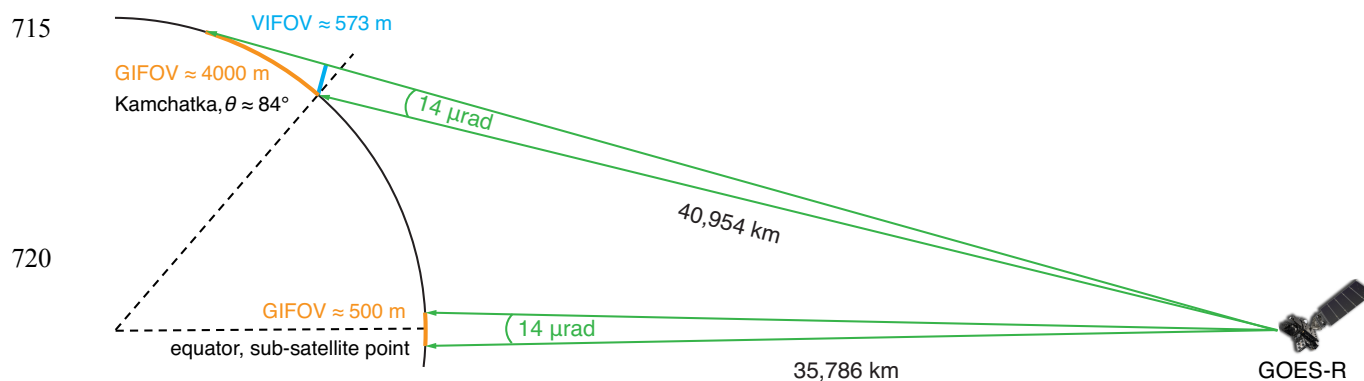
725 Figure 1. Horizontal (GIFOV, orange) and vertical (VIFOV, blue) spatial resolution of an ABI band 2 fixed grid pixel at the sub-satellite point and the Sheveluch volcano in Kamchatka observed at a view zenith angle of \theta \approx 84^\circ . The fixed grid has an angular resolution of 14 \mu\text{rad} in both the east-west and the north-south directions and is rectified to the GRS80 ellipsoid as viewed from an idealized geostationary position. Note the figure is not drawn to scale.
