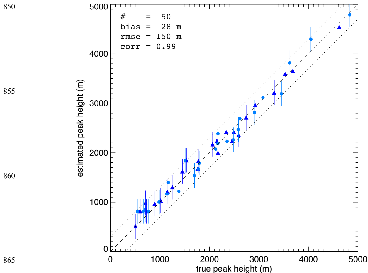
870 Figure 9. Peak height estimated by the side view method versus true peak height; two different colors and symbols are used only to help distinguish overlapping data points. The dashed line is the 1:1 line and the dotted lines mark \pm 2 \times \text{RMSE} about the 1:1 line. The error bars on a data point represent the standard deviation of the nine height estimates corresponding to the visually identified peak location and its 8-pixel neighborhood.
