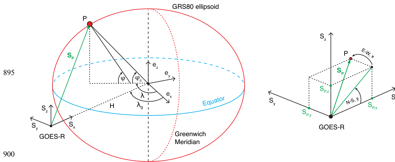
Figure A1. Coordinate systems used for ABI fixed grid navigation.
