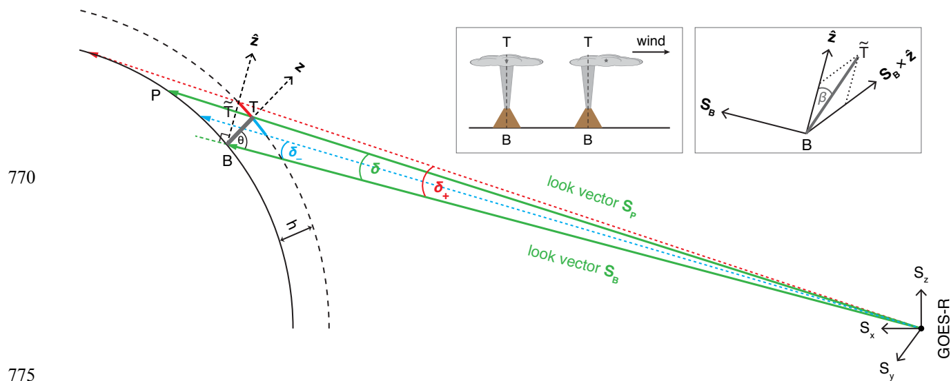
Figure 4. Side view geometry of a vertical column located near the limb as imaged by a geostationary sensor.
