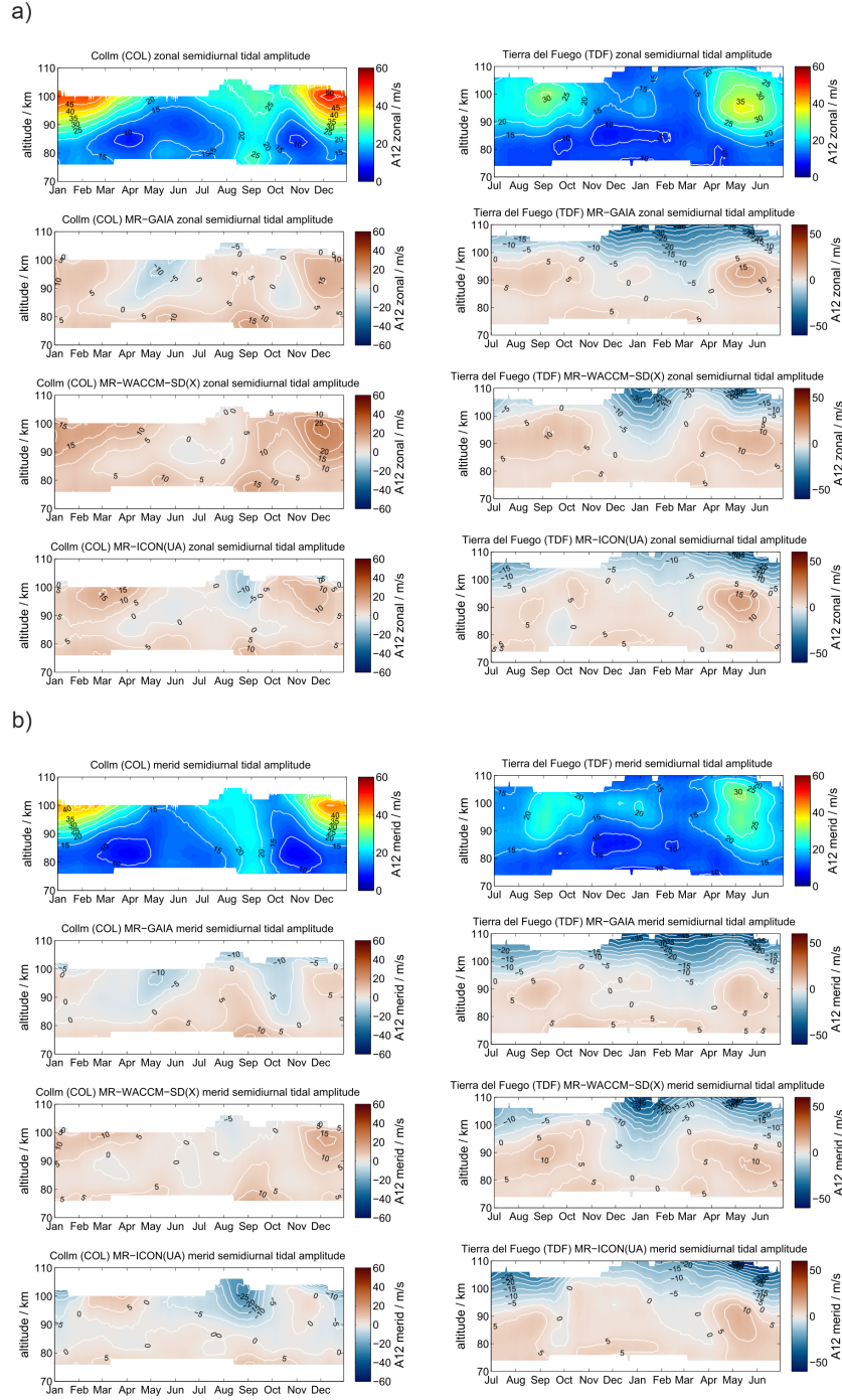
Figure D2. The same as Figure D1, but for COL and TDF.
