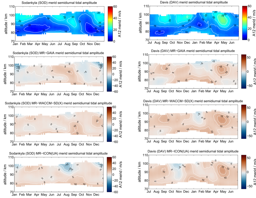
Figure D1. Absolute difference plots for semidiurnal tidal amplitudes meteor radar - model fields for SOD and DAV.
