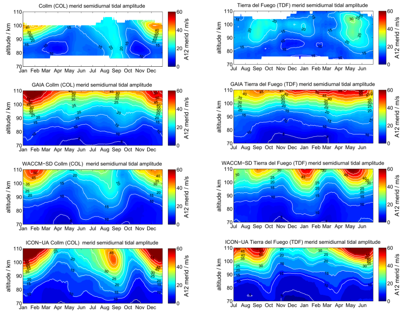
Figure 13. The same as Figure 2, but for the semidiurnal tidal amplitudes above COL and TDF.
