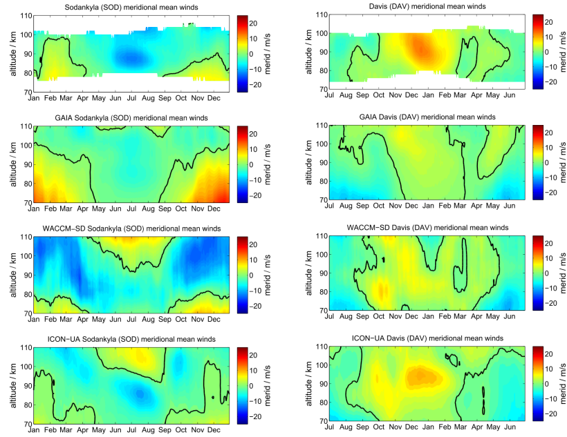
Figure 2. Comparison of zonal (panel a) and meridional (panel b) daily mean winds for the MRs at SOD (left column) and DAV (right column). The winds for Davis are shifted by half a year.
