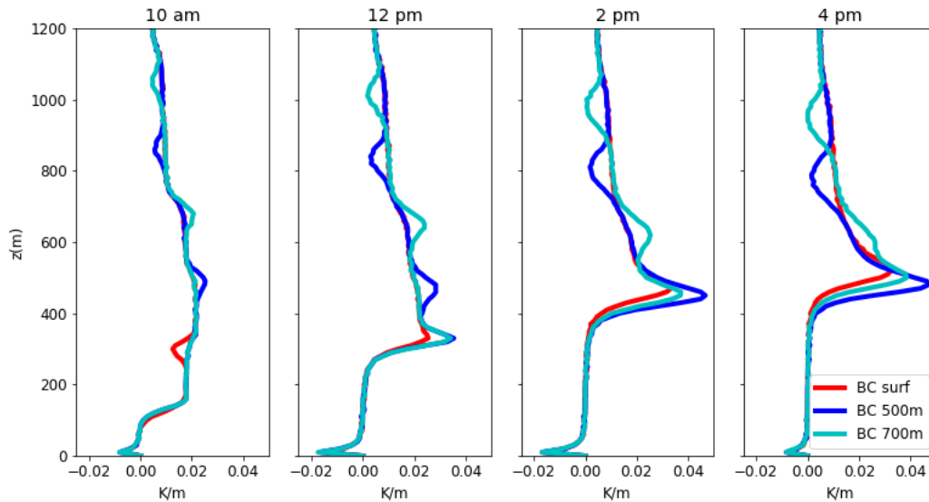
Figure 6. Potential temperature lapse rate for simulations on 3rd Dec at 10am, 12pm, 2pm and 4pm for Aero_load_BCsurf (red), Aero_load_BC500 (blue) and Aero_load_BC700 (cyan) simulations
