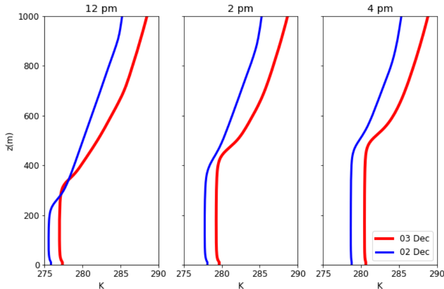
Figure 7. Potential temperature profiles for Met_0312_noaero simulations (red lines) and Met_0212_noaero (blue lines) at 12pm, 2pm and 4pm LST
