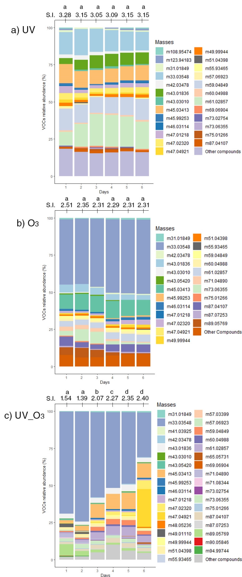
625 Figure 5: VOC relative abundance for rapeseed litter samples under a) UV light b) O 3 and c) UV_O 3 conditions. S.I. is the Shannon index representing the diversity of the VOC (for each day). Letters indicate significant differences of the S.I. according to the Tukey test with p.value < 0.05.
