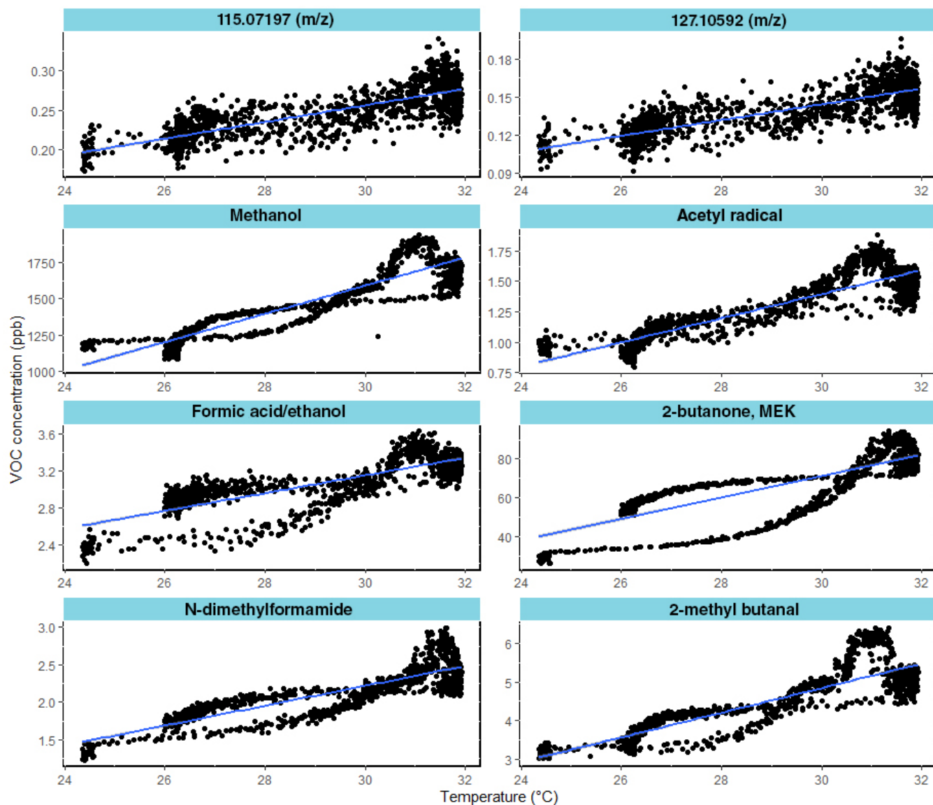
Figure 7 Correlation between VOC mixing ratios and temperature under the UV_O 3 condition. The 8 most correlated VOC are shown(Pearson correlation coefficients > 0.8). .
